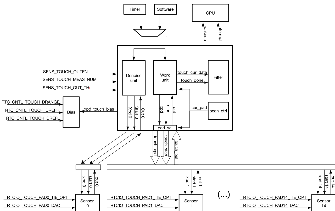
Figure 39-4. Touch FSM Structure
