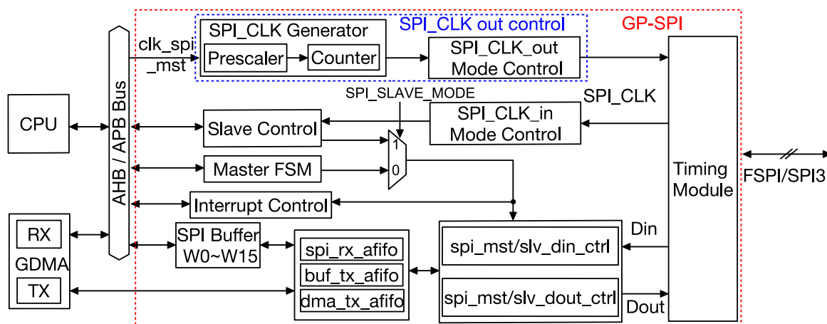
Figure 30-3. GP-SPI Block Diagram
