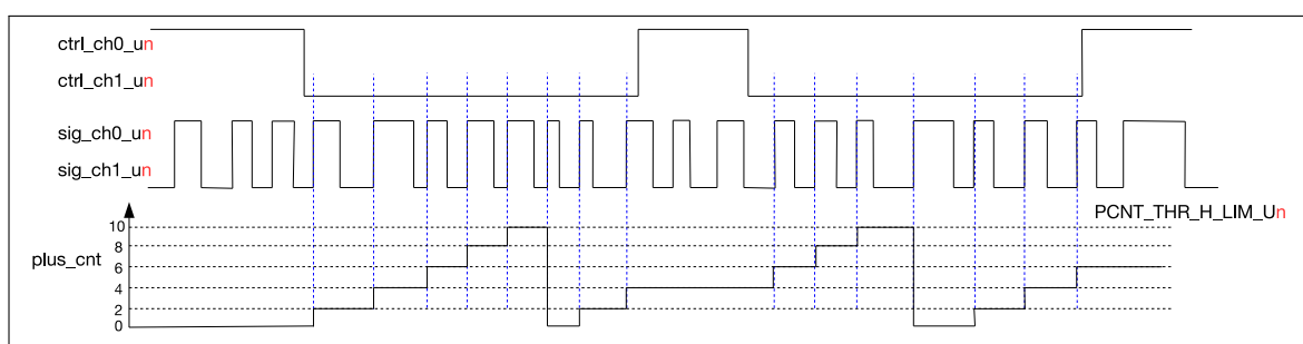
Figure 38-5. Two Channels Up Counting Diagram
