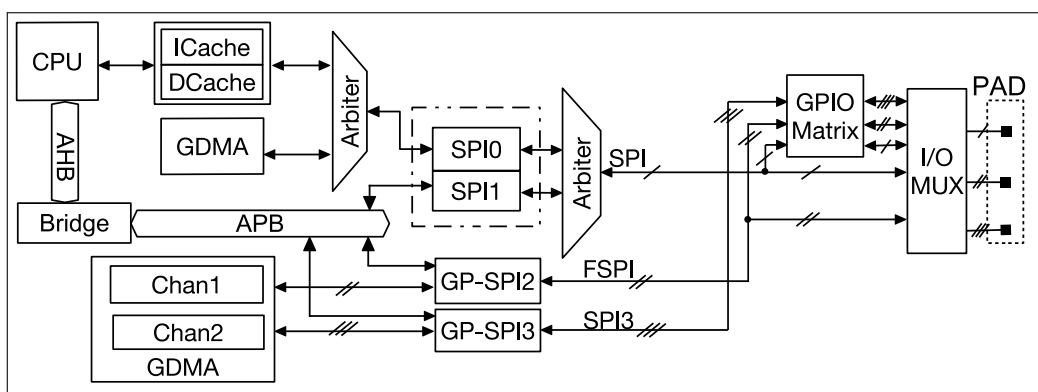
Figure 30-1. SPI Module Overview
