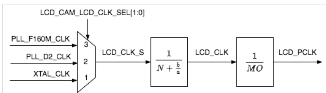
Figure 29-2. LCD Clock
