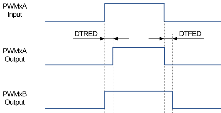
Figure 36-25. Active High (AH) Dead Time Waveforms
