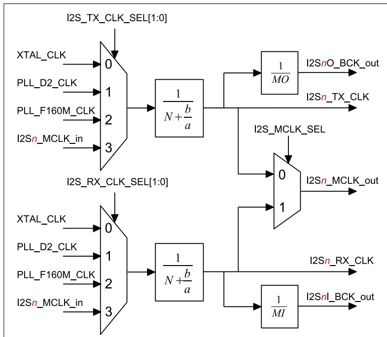
Figure 28-6. I2S n Clock
