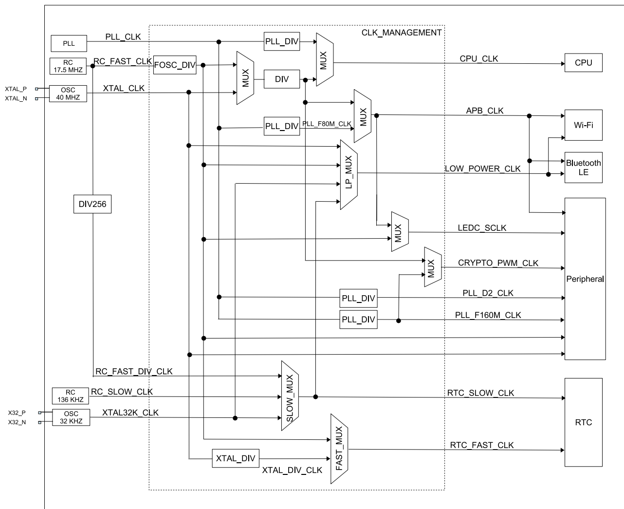
Figure 7-2. Clock Structure
