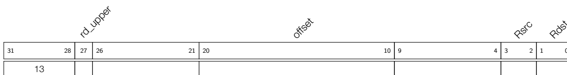
Figure 2-15. Instruction Type - LD
