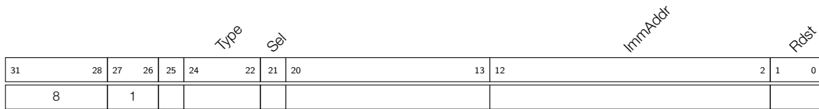
Figure 2-16. Instruction Type - JUMP
