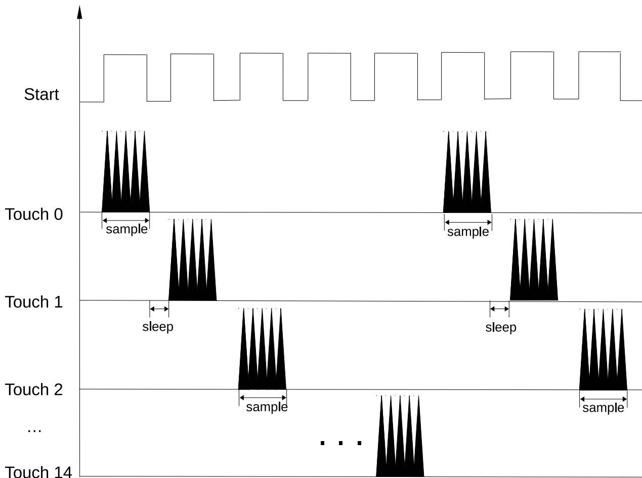
Figure 39-5. Timing Diagram of Touch Scan
