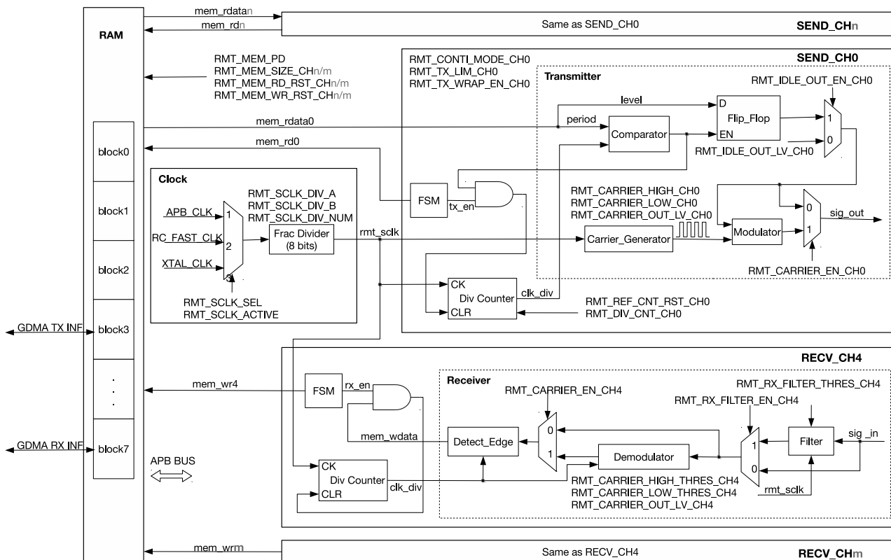
Figure 37-1. RMT Architecture
