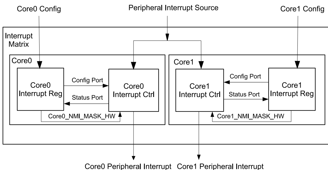
Figure 9-1. Interrupt Matrix Structure
