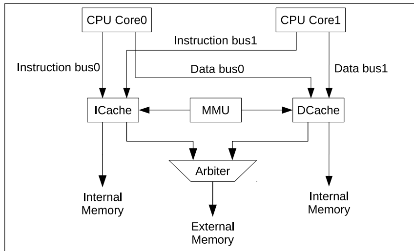
Figure 4-2. Cache Structure
