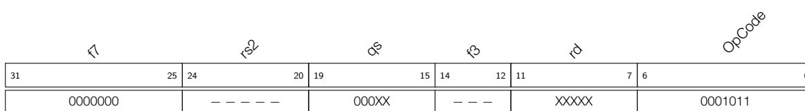
Figure 2-27. Interrupt Instruction - getq rd, qs
