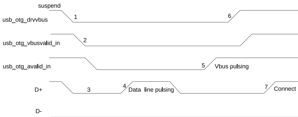
Figure 32-7. A-Device SRP
