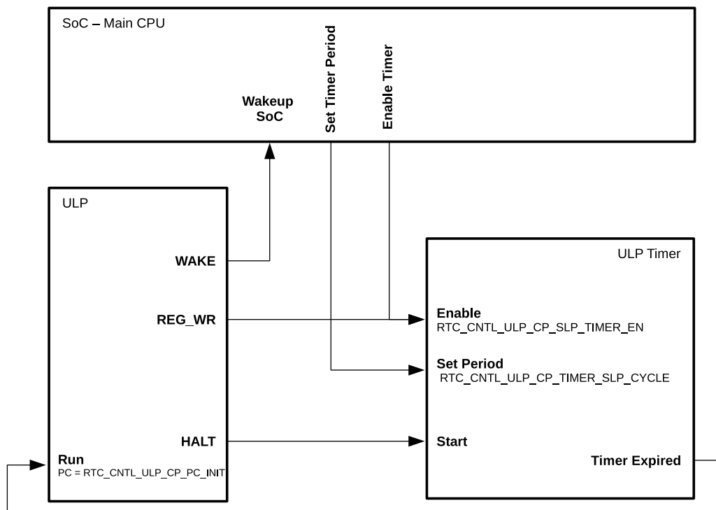
Figure 2-5. Control of ULP Program Execution
