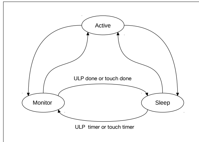
Figure 10-10. RTC States
