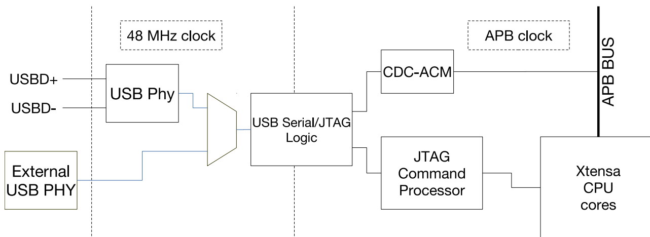
Figure 33-1. USB Serial/JTAG High Level Diagram
