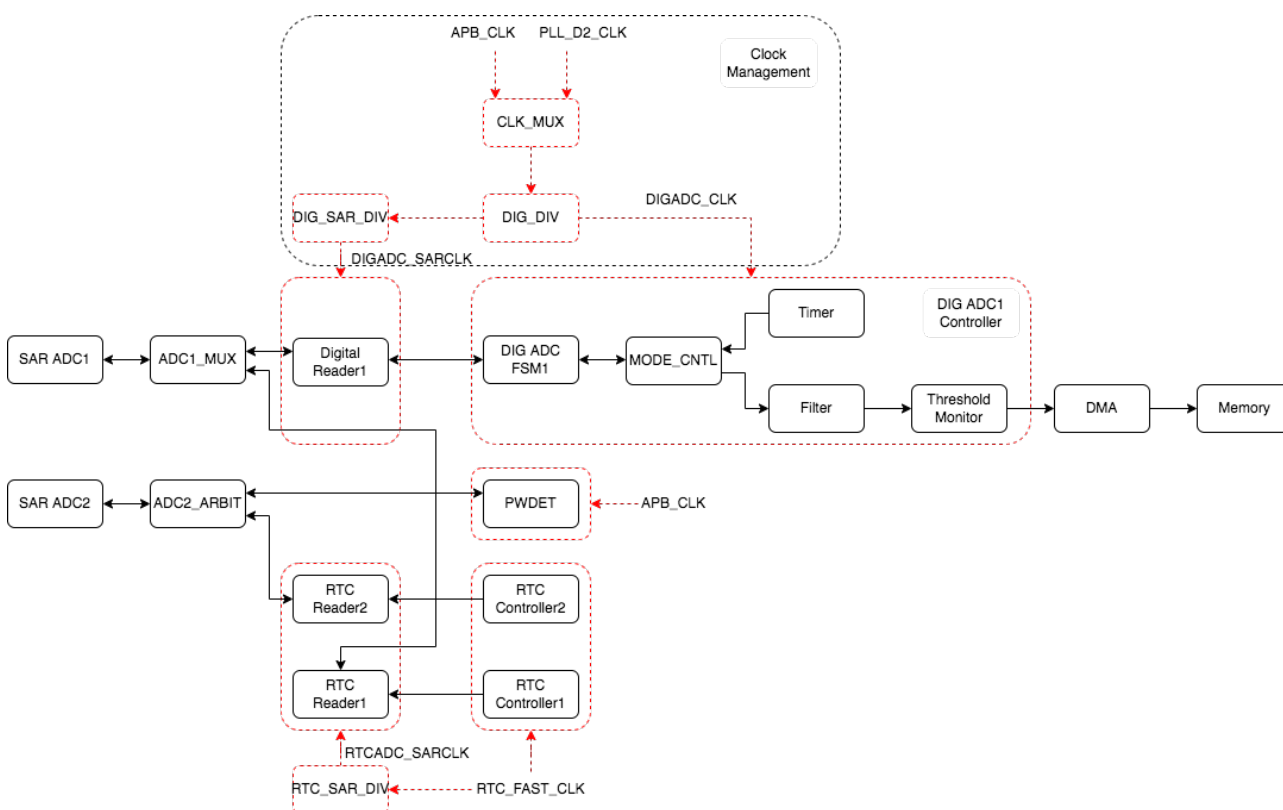
Figure 39-8. SAR ADC Architecture
