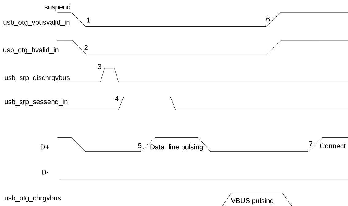
Figure 32-8. B-Device SRP
