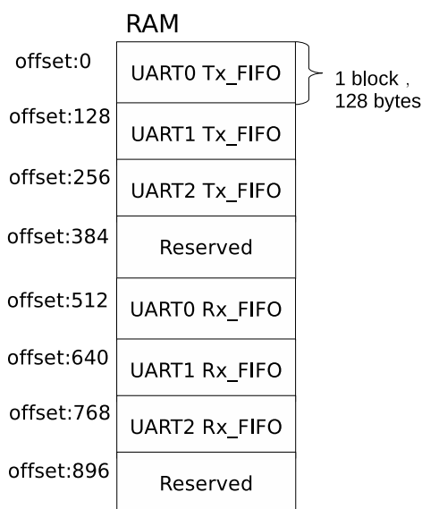
Figure 26-2. UART Controllers Sharing RAM
