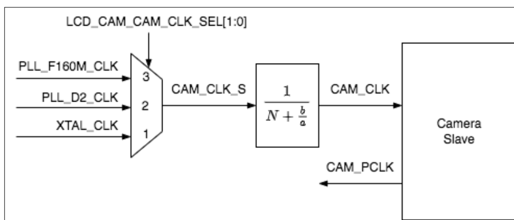
Figure 29-3. Camera Clock
