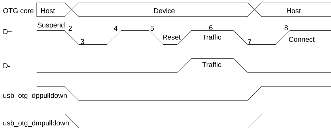
Figure 32-9. A-Device HNP
