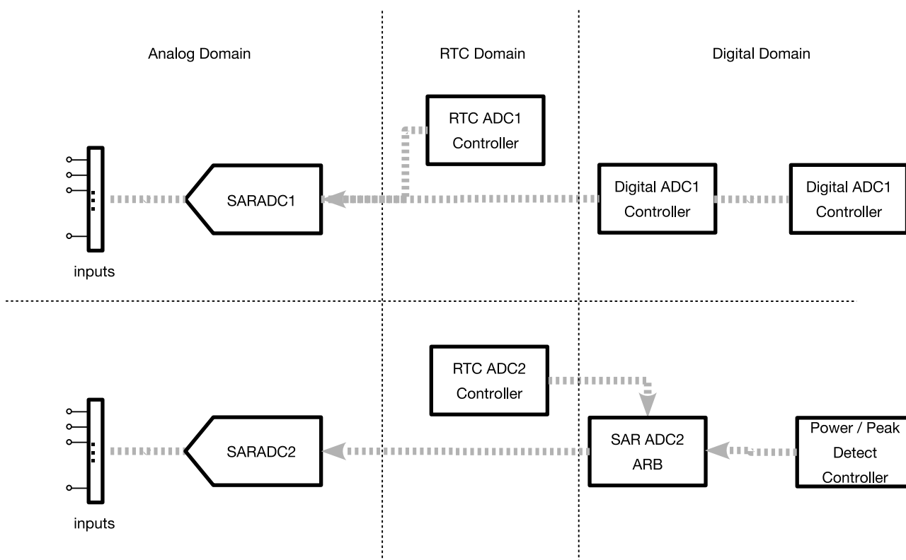
Figure 39-7. SAR ADC Overview
