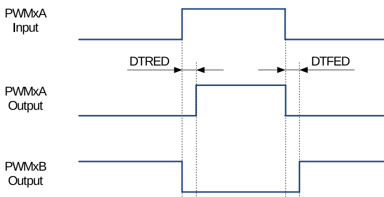
Figure 36-23. Active High Complementary (AHC) Dead Time Waveforms
