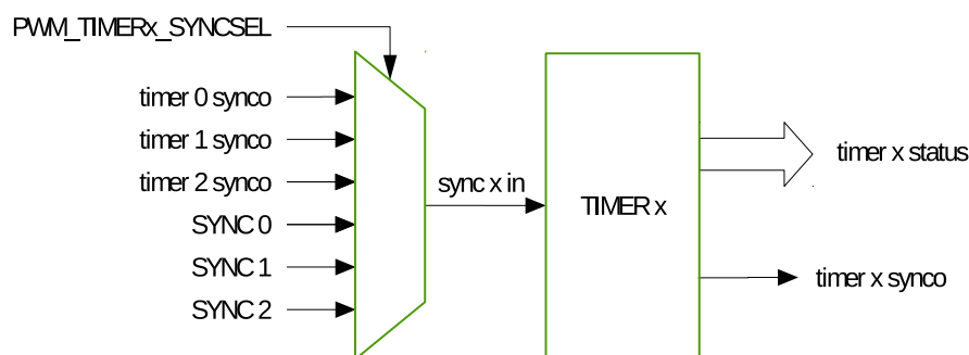
Figure 36-3. Timer Submodule
