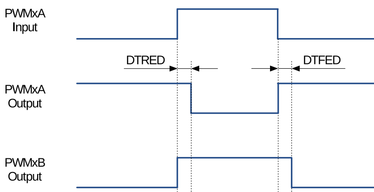
Figure 36-24. Active Low Complementary (ALC) Dead Time Waveforms
