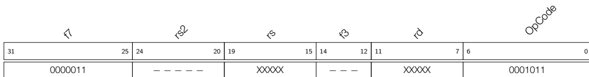
Figure 2-30. Interrupt Instruction — Maskirq rd rs
