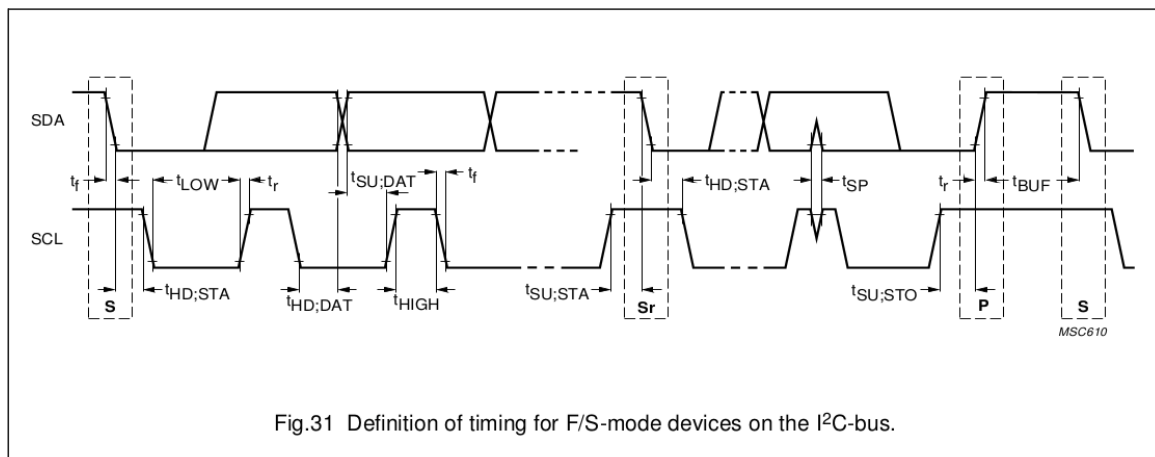
Figure 27-3. I2C Protocol Timing (Cited from Fig.31 in The I2C-bus specification Version 2.1 )
