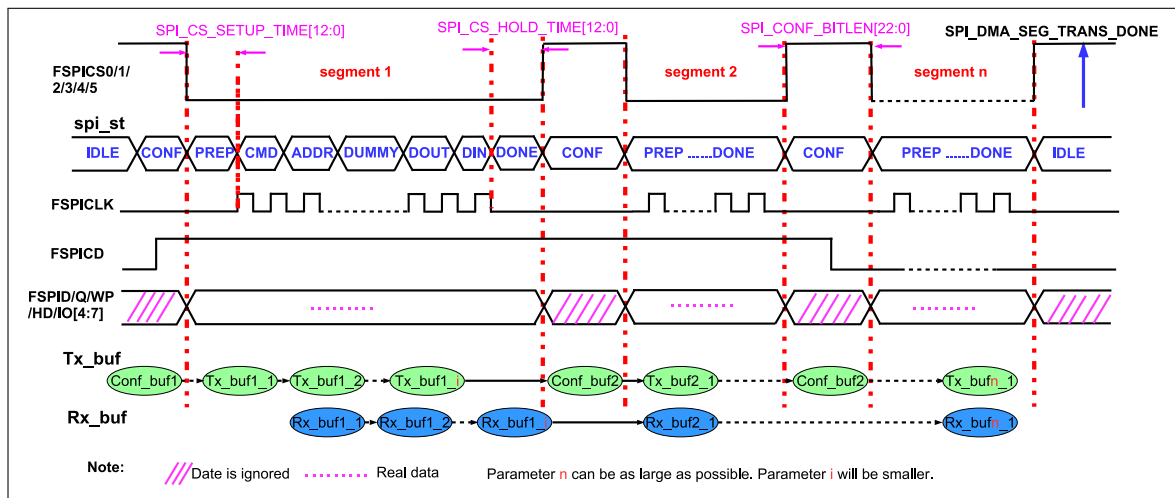
Figure 30-10. Configurable Segmented Transfer in DMA-Controlled Master Mode
