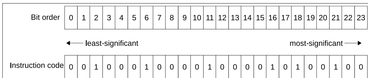
Figure 1-3. EE.ZERO.QACC in Big-Endian Bit Order
