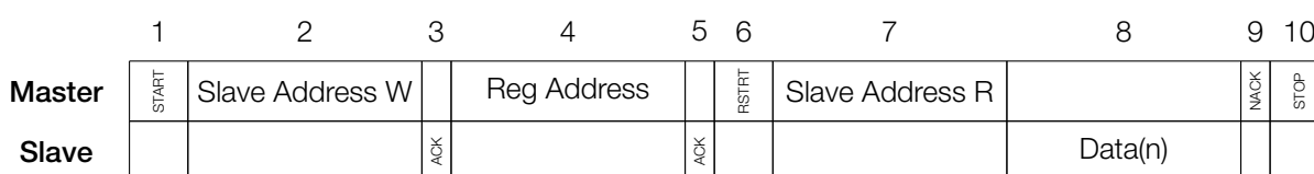
Figure 2-31. I2C Read Operation
