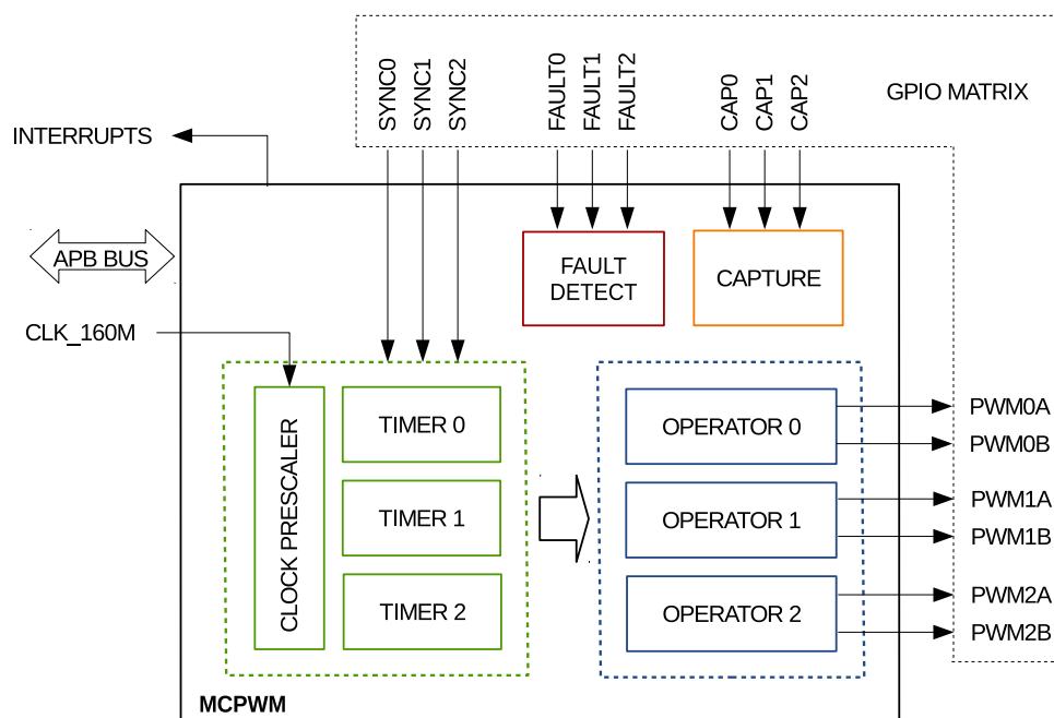
Figure 36-1. MCPWM Module Overview
