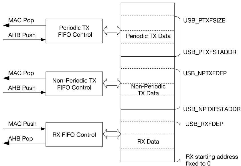
Figure 32-3. Host Mode FIFOs
