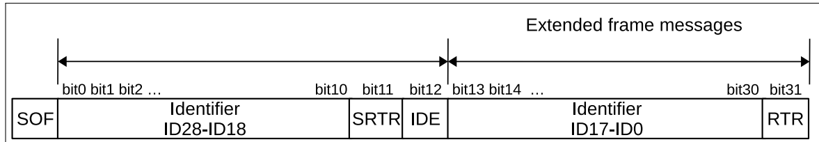
Figure 31-11. Positions of Arbitration Lost Bits
