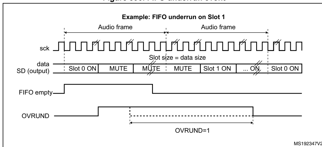
Figure 390. FIFO underrun event
