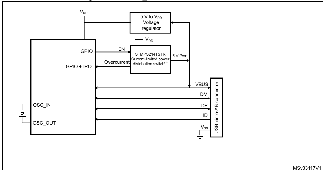
Figure 439. OTG_FS A-B device connection
