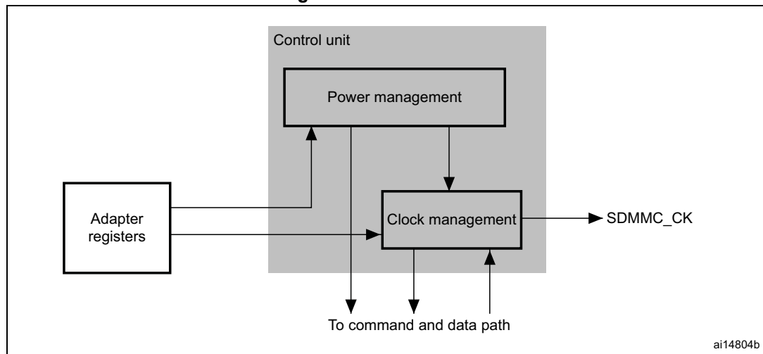
Figure 414. Control unit
