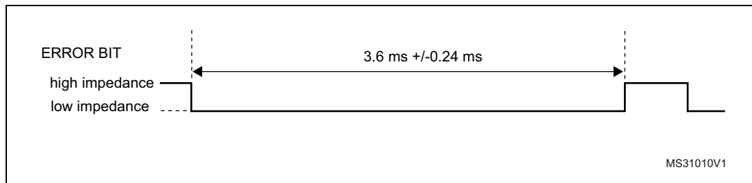
Figure 512. Error bit timing
