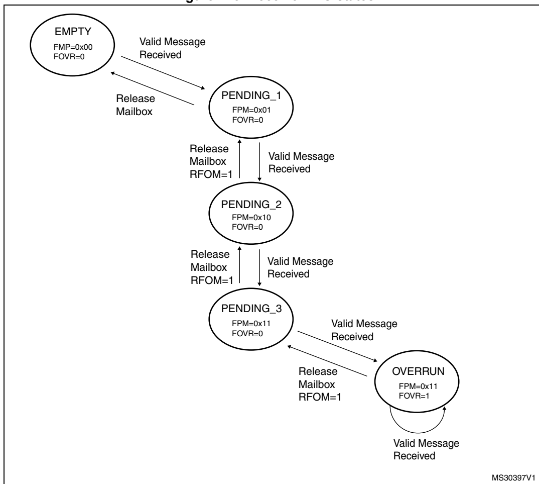
Figure 428. Receive FIFO states
