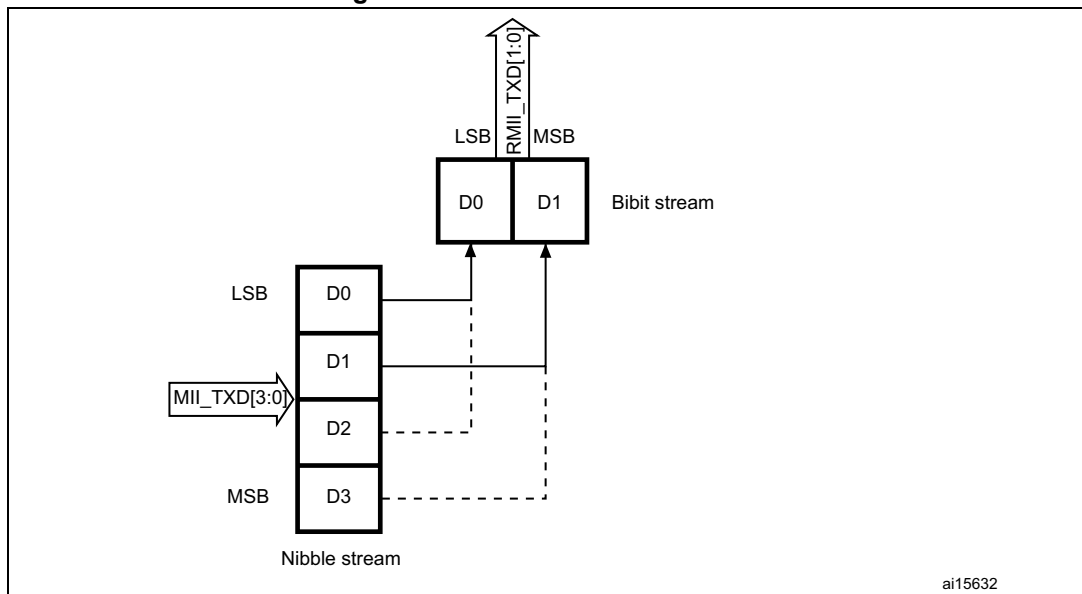
Figure 481. Transmission bit order
