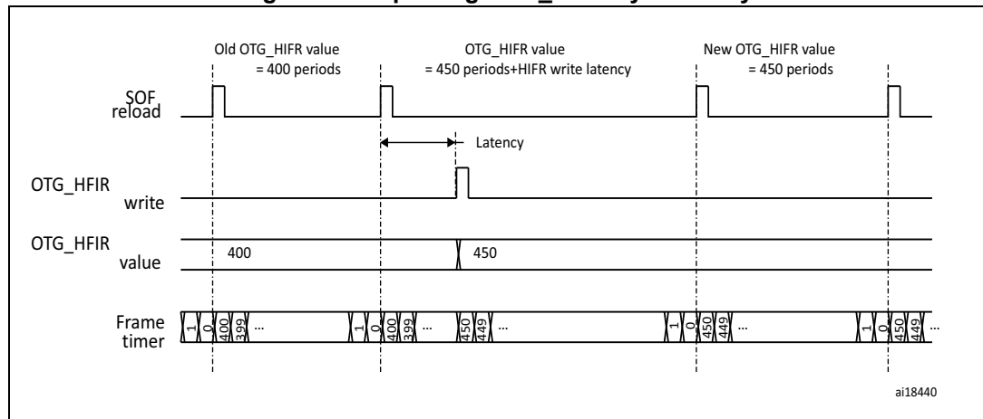
Figure 443. Updating OTG_HFIR dynamically
