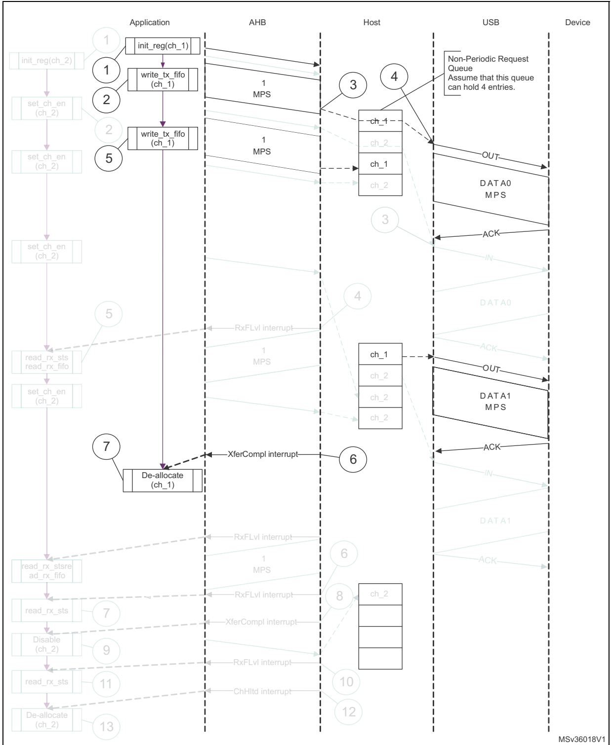
Figure 449. Normal bulk/control OUT/SETUP
