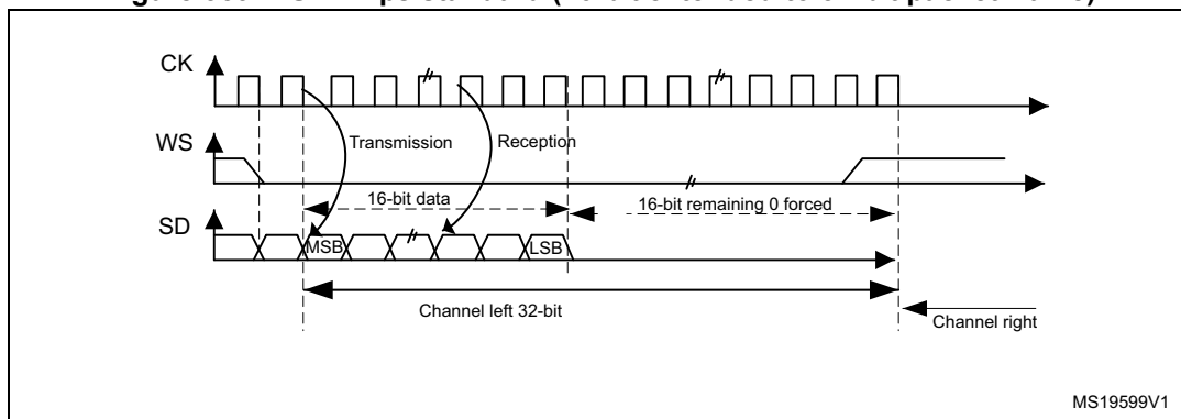
Figure 359. I 2 S Philips standard (16-bit extended to 32-bit packet frame)
