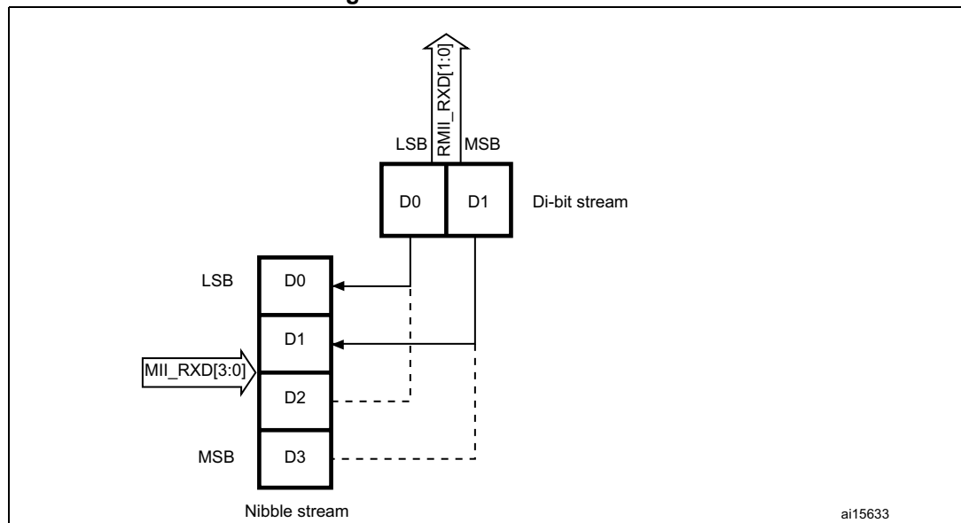
Figure 485. Receive bit order
