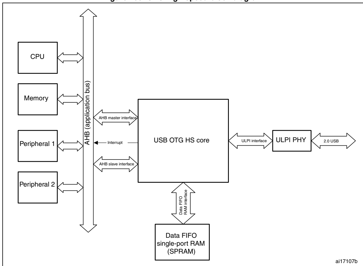
Figure 438. OTG high-speed block diagram
