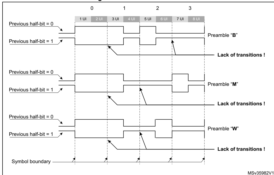
Figure 394.S/PDIF Preambles
