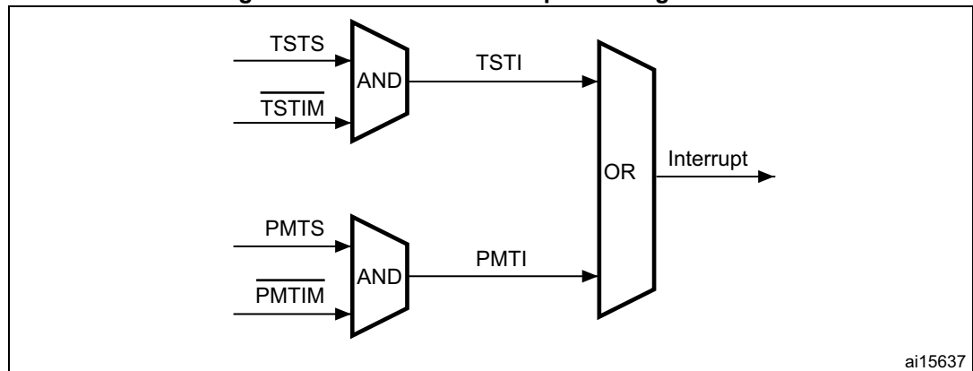
Figure 489. MAC core interrupt masking scheme
