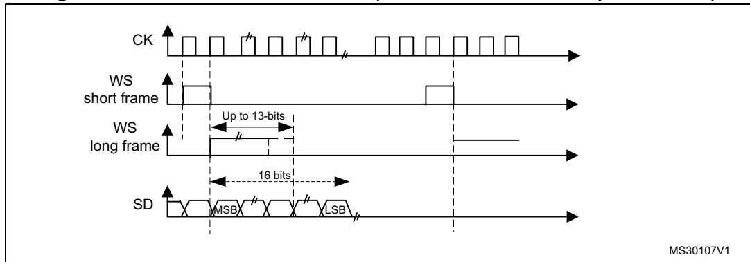
Figure 371. PCM standard waveforms (16-bit extended to 32-bit packet frame)
