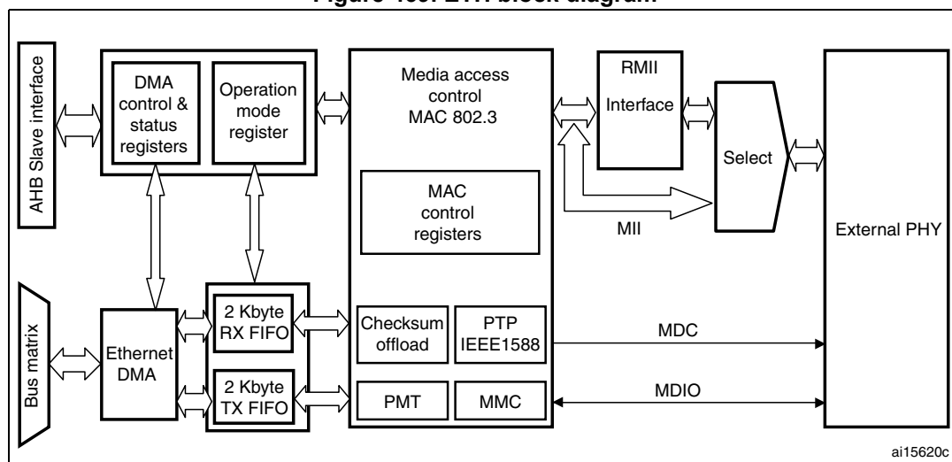
Figure 469. ETH block diagram
