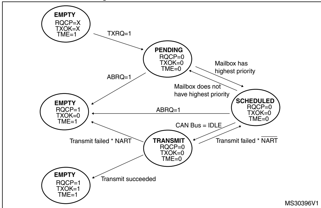
Figure 427. Transmit mailbox states
