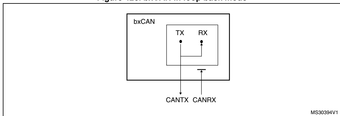
Figure 425. bxCAN in loop back mode
