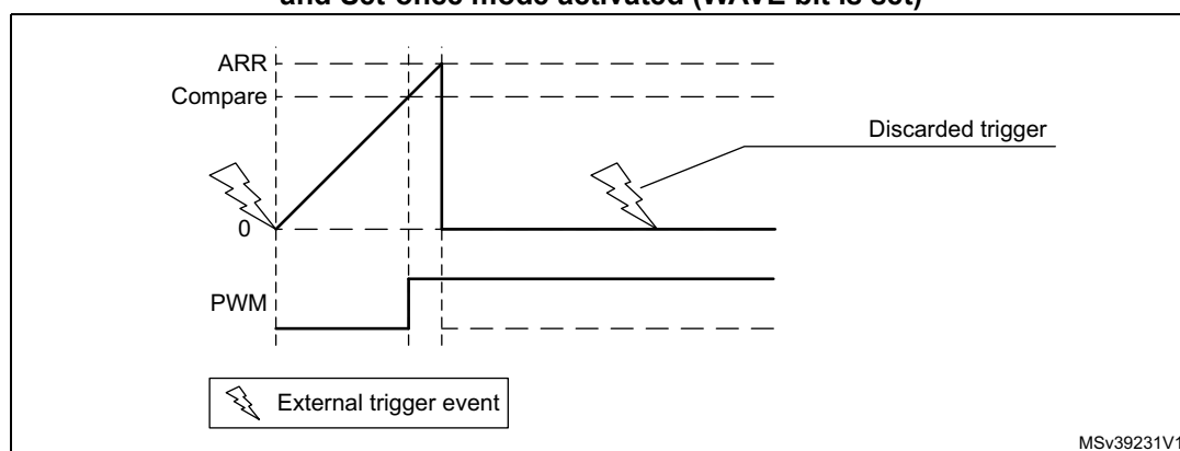
Figure 275. LPTIM output waveform, Single counting mode configuration and Set-once mode activated (WAVE bit is set)
