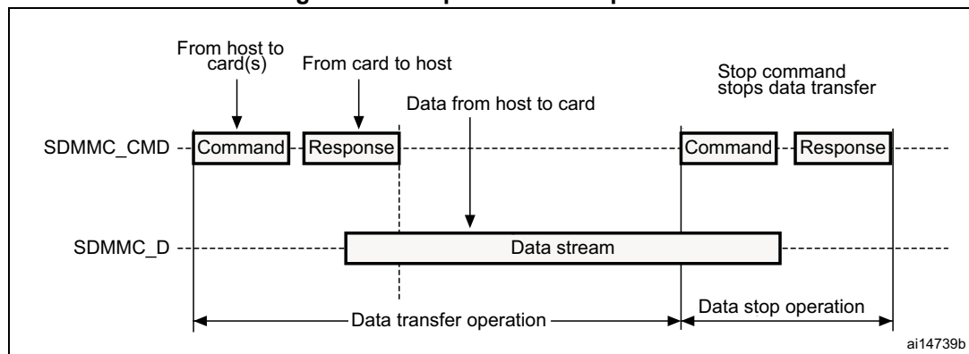
Figure 411. Sequential write operation
