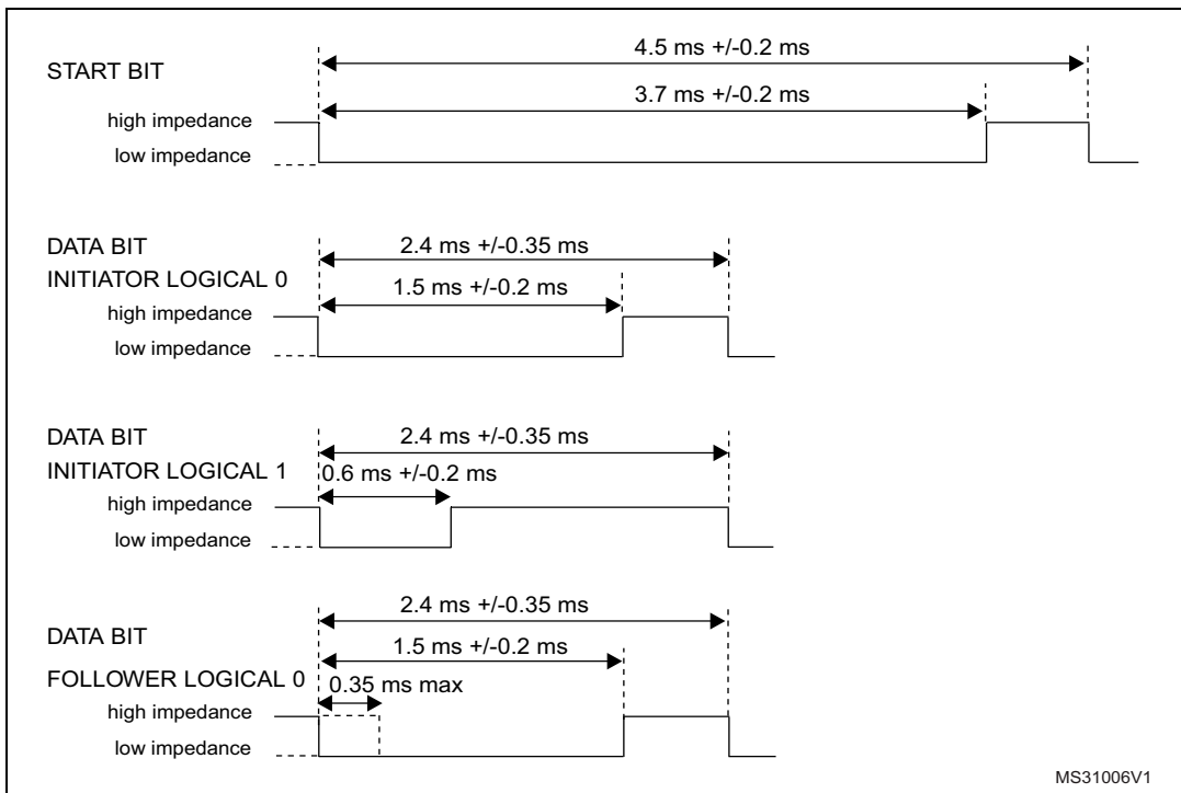
Figure 508. Bit timings
