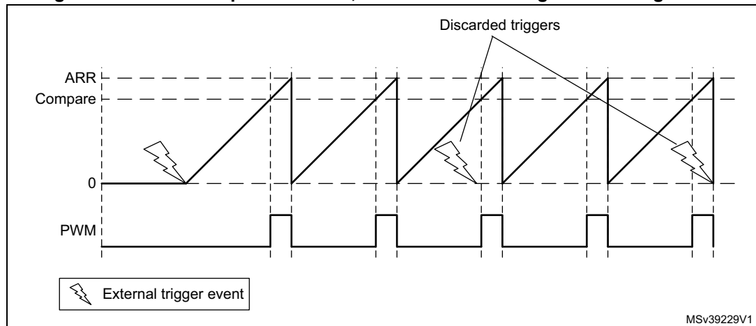
Figure 276. LPTIM output waveform, Continuous counting mode configuration
