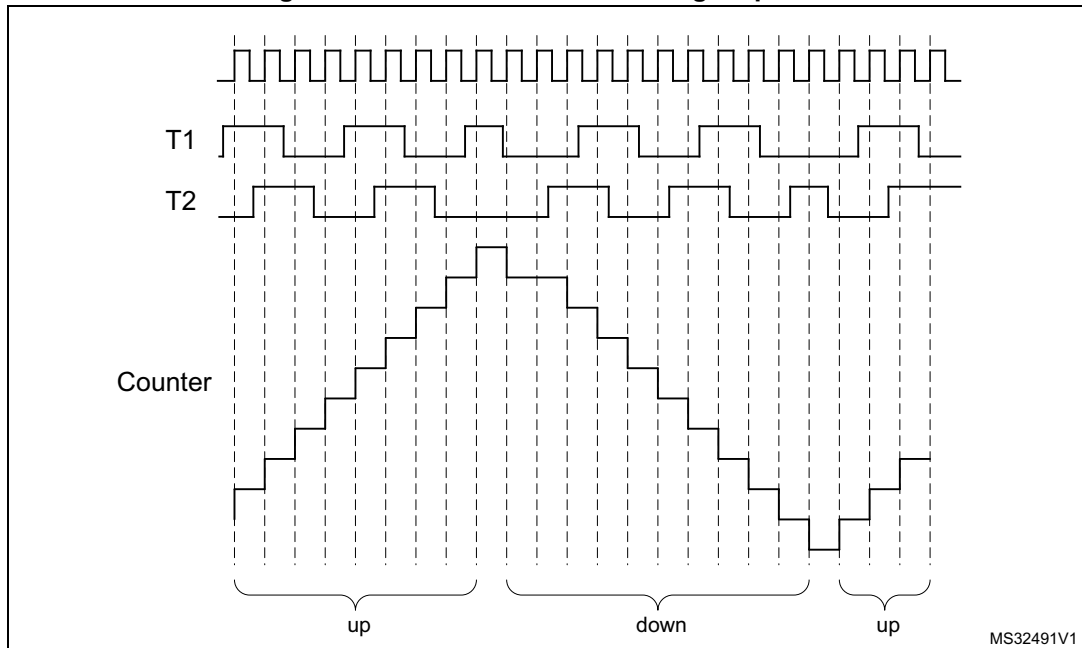
Figure 278. Encoder mode counting sequence
