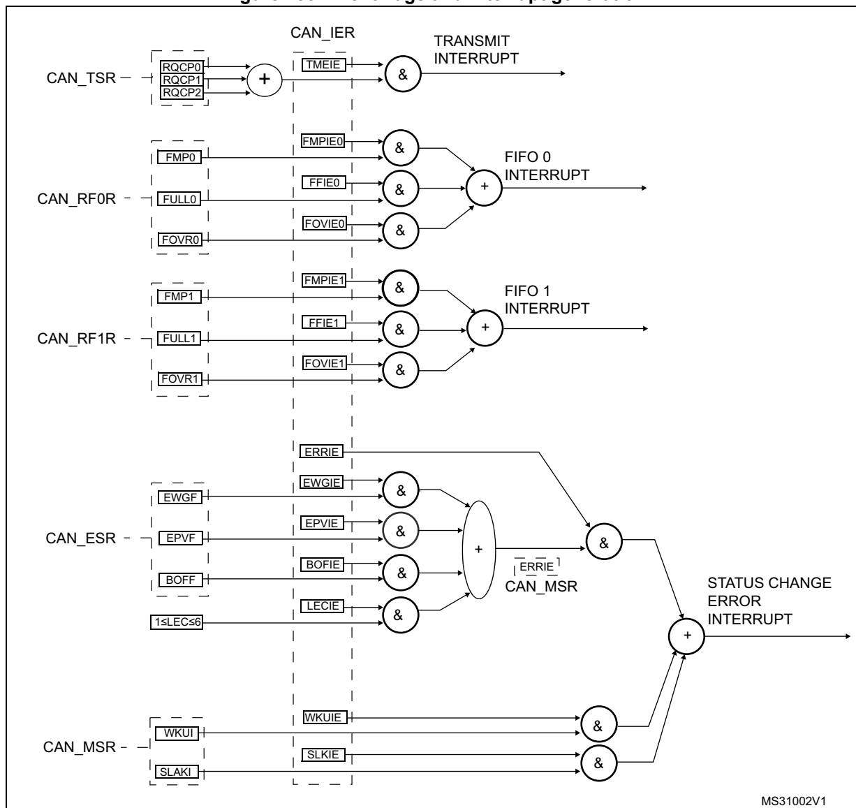
Figure 435. Event flags and interrupt generation
