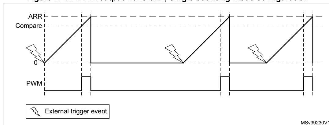
Figure 274. LPTIM output waveform, Single counting mode configuration
