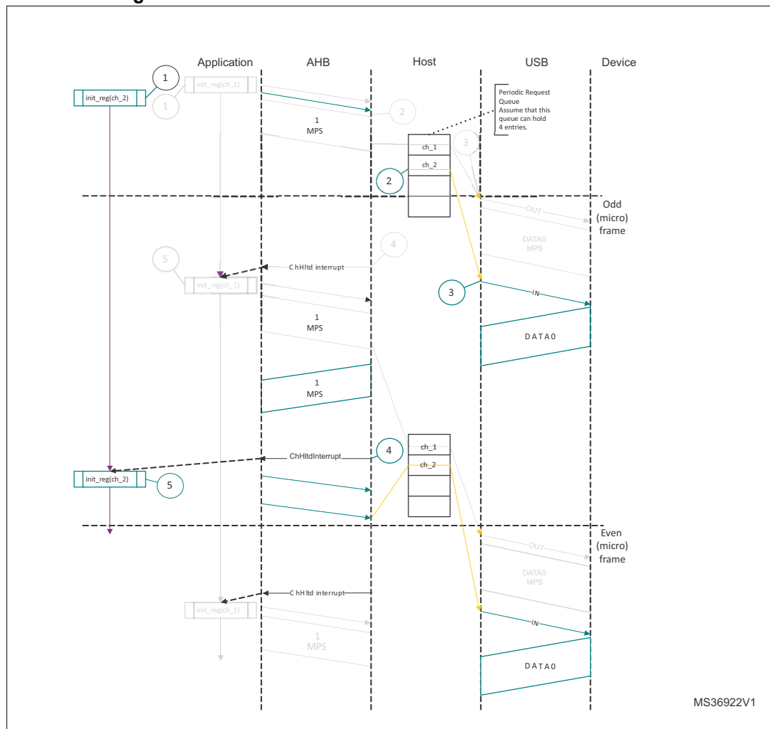
Figure 460. Normal isochronous IN transactions - DMA mode
