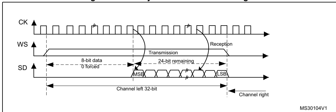
Figure 365. LSB justified 24-bit frame length
