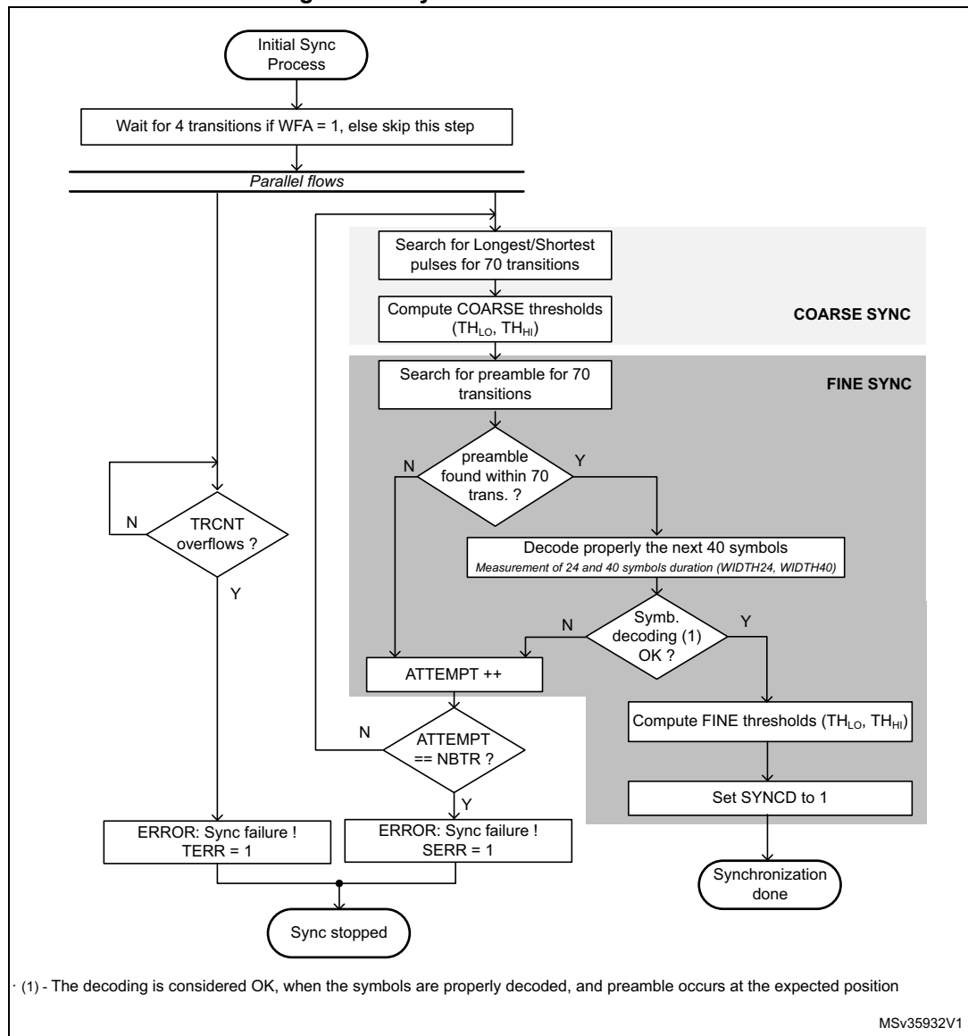
Figure 399.Synchronization flowchart
