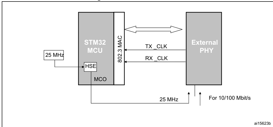
Figure 474. MII clock sources
