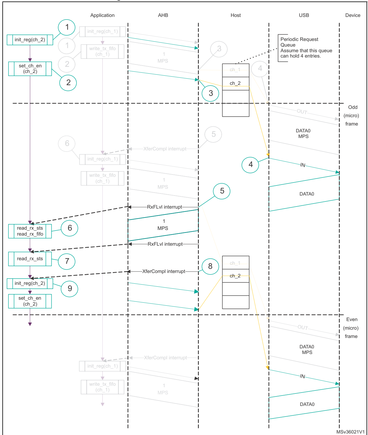
Figure 454. Isochronous IN transactions
