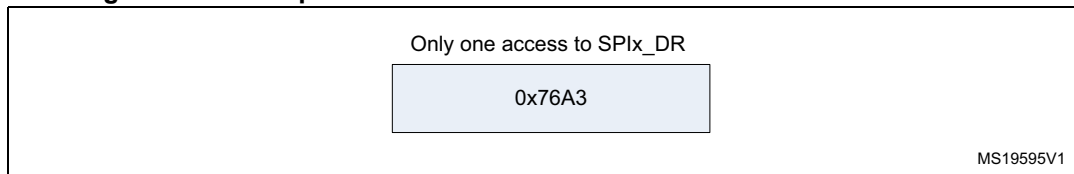
Figure 360. Example of 16-bit data frame extended to 32-bit channel frame
