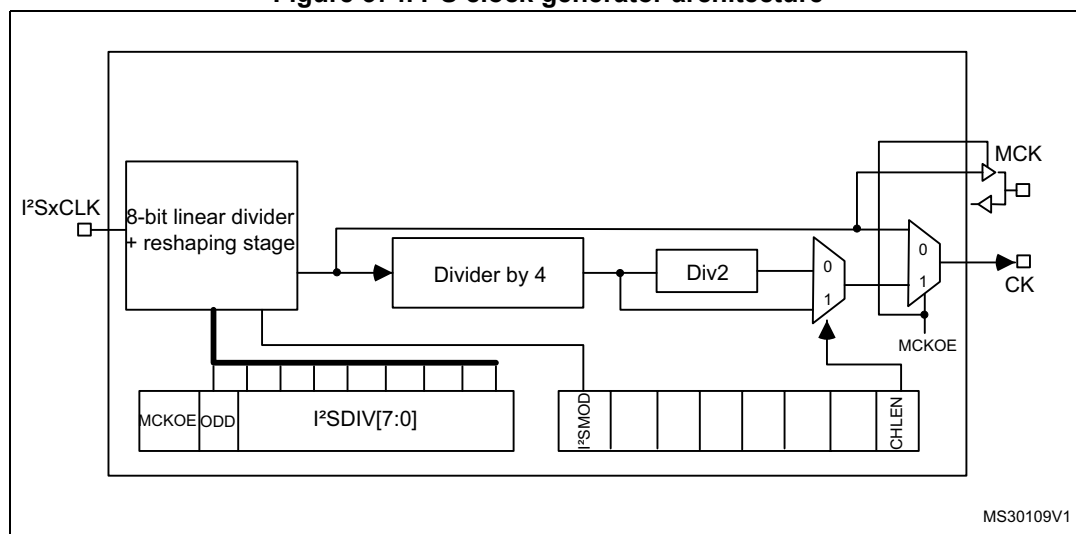
Figure 374. I 2 S clock generator architecture
