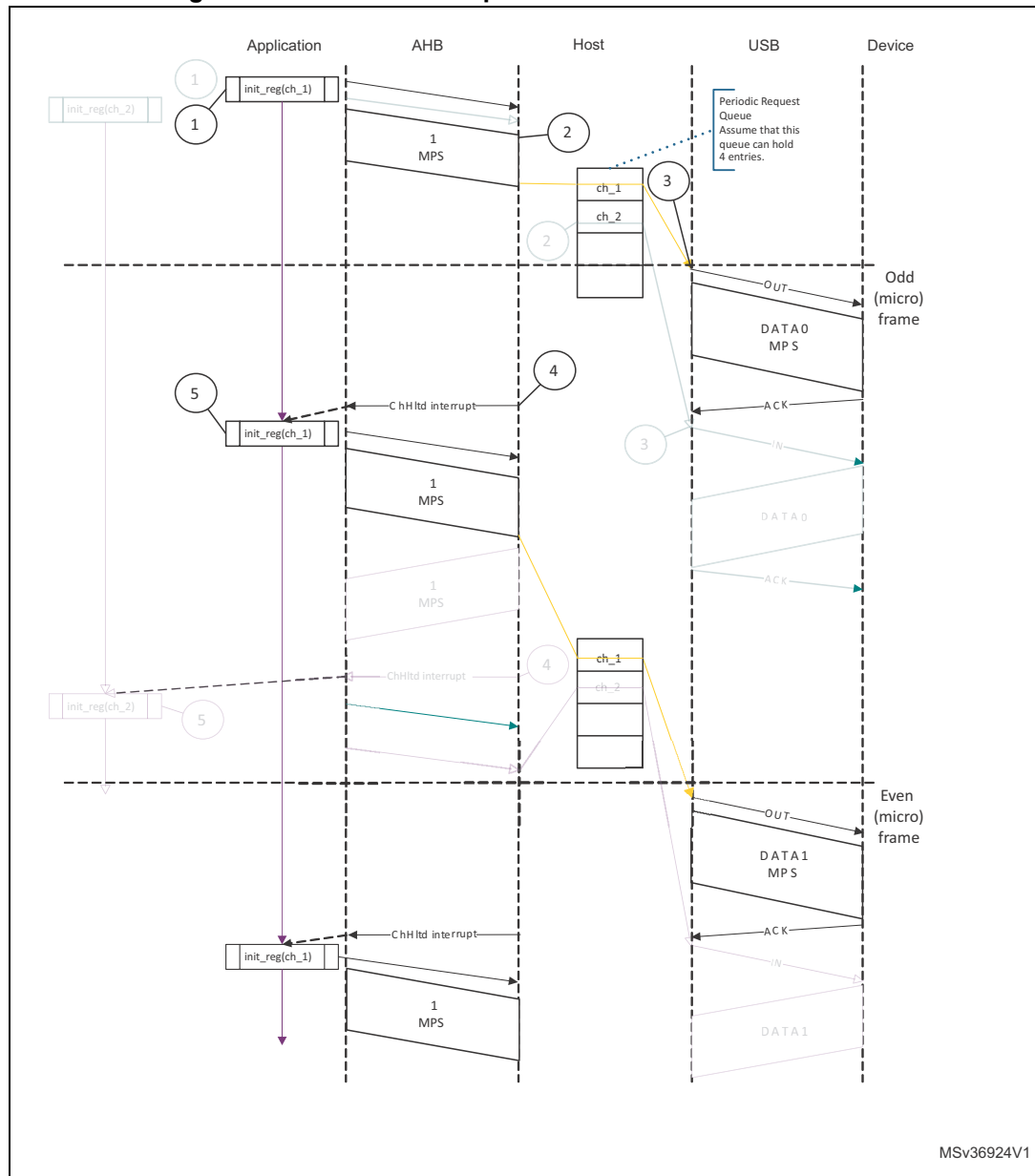
Figure 457. Normal interrupt OUT transactions - DMA mode
