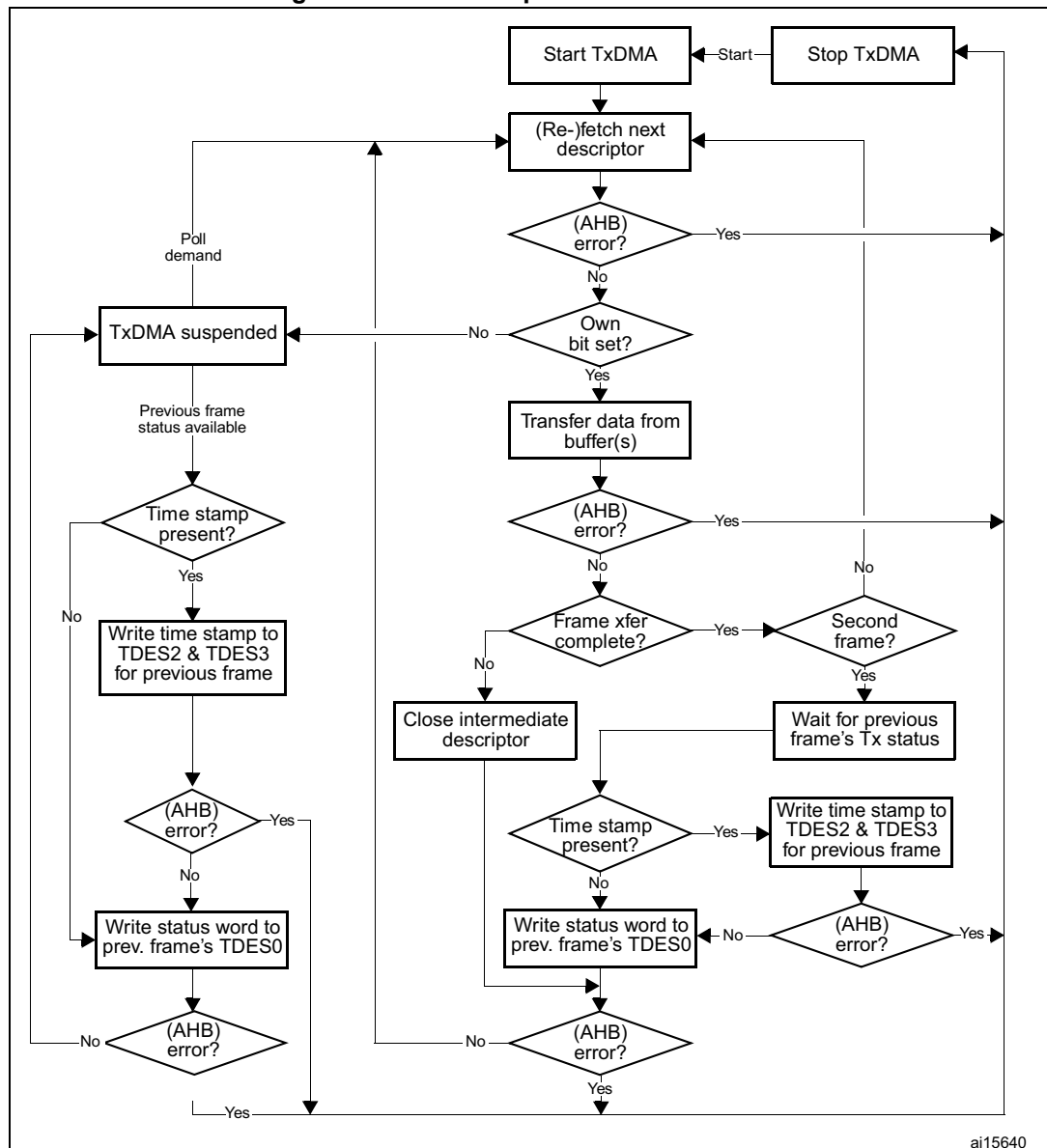
Figure 497. TxDMA operation in OSF mode
