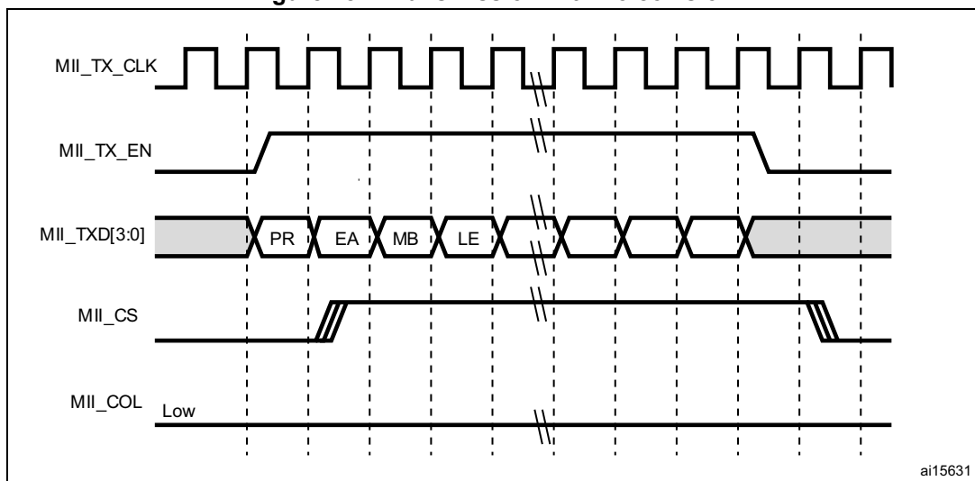
Figure 482. Transmission with no collision
