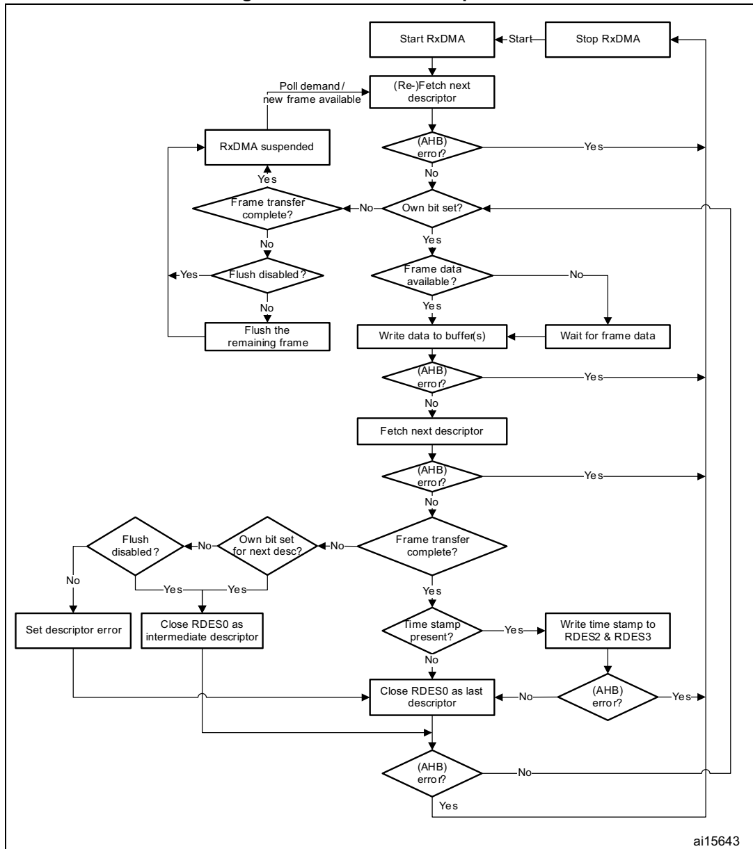
Figure 500. Receive DMA operation
