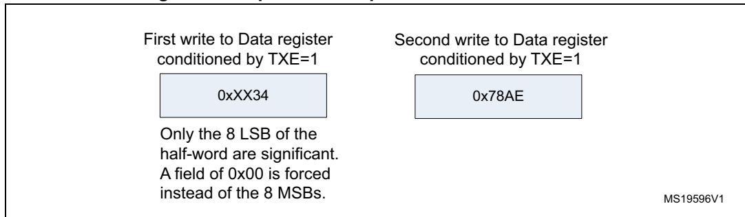
Figure 366. Operations required to transmit 0x3478AE
