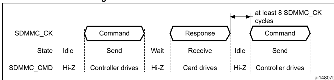
Figure 418. SDMMC command transfer
