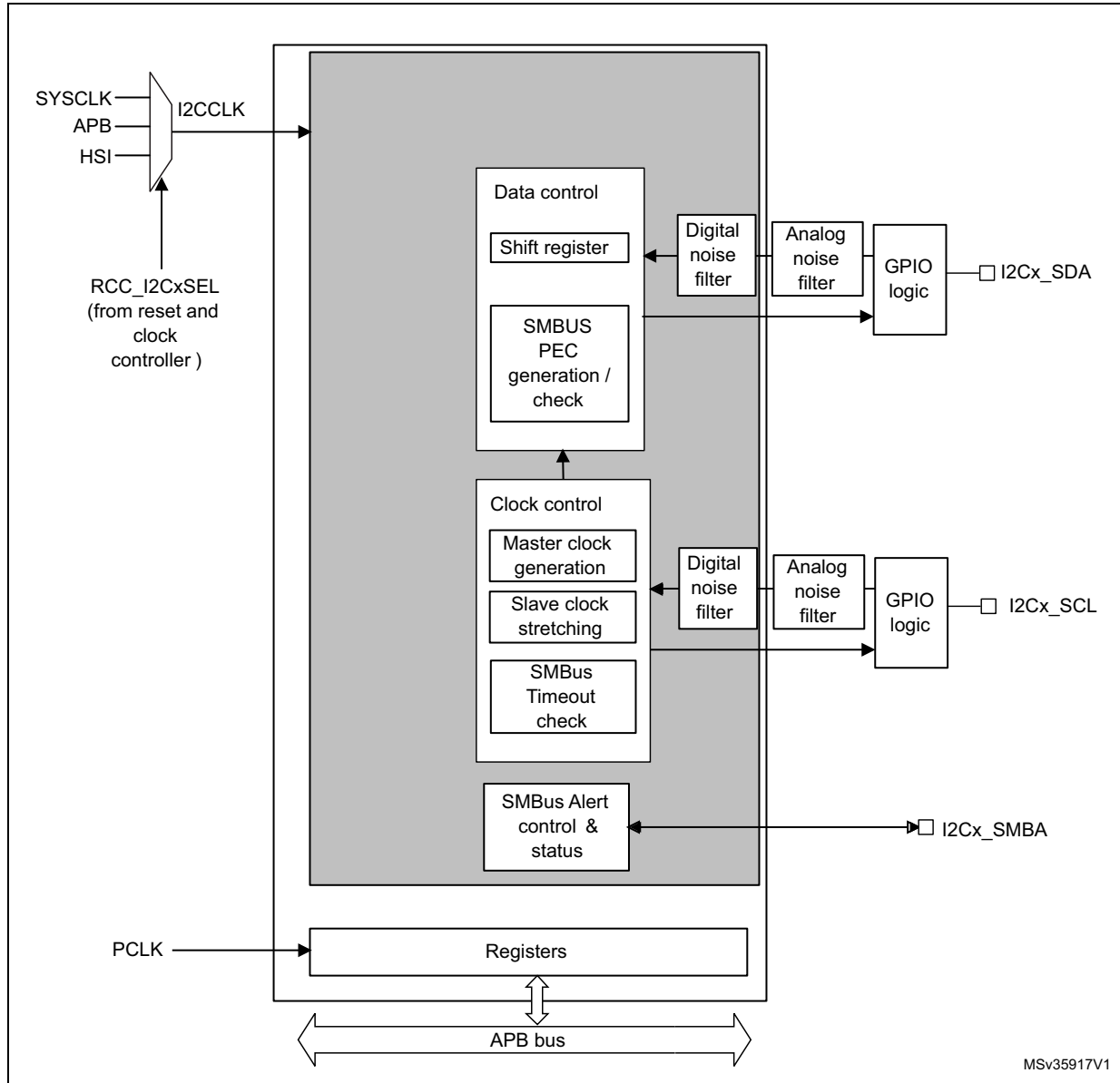
Figure 283. I2C block diagram
