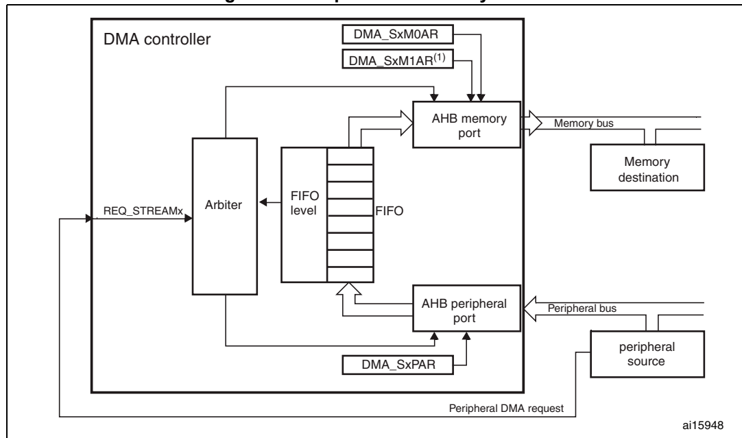
Figure 24. Peripheral-to-memory mode
