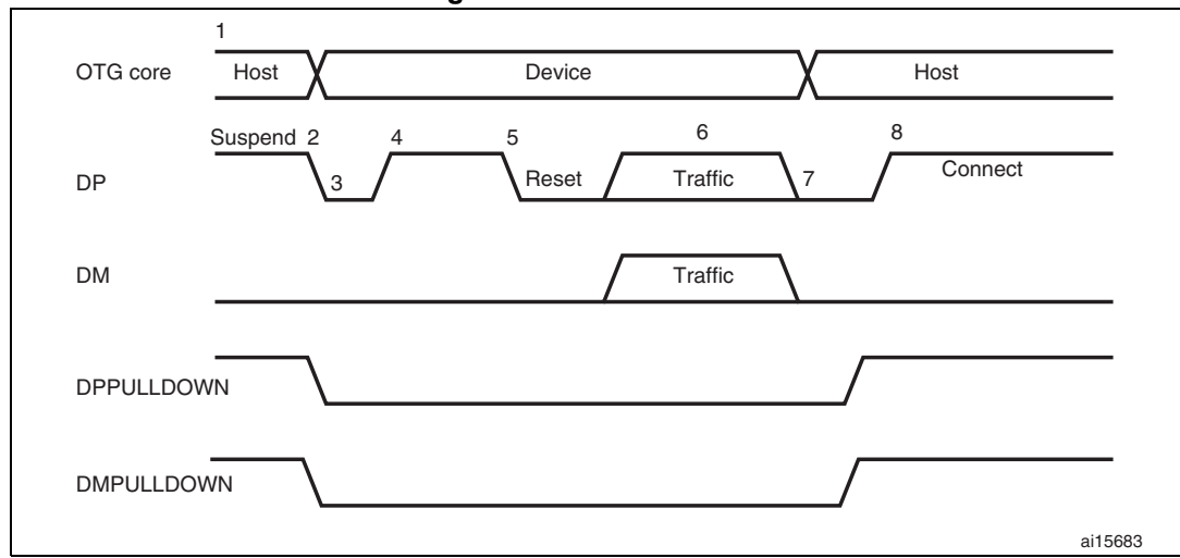
Figure 467. A-device HNP
