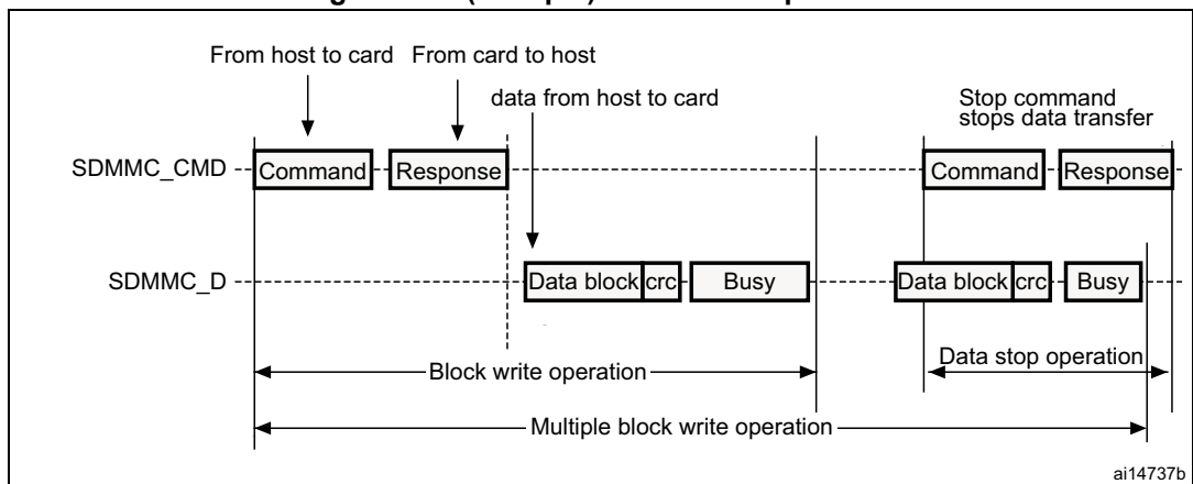
Figure 409. (Multiple) block write operation
