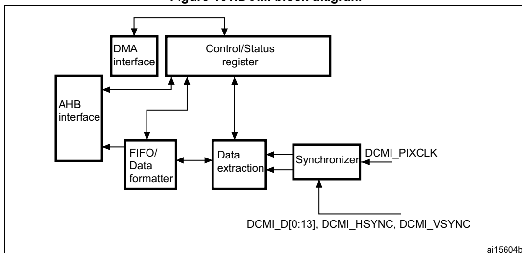
Figure 101.DCMI block diagram
