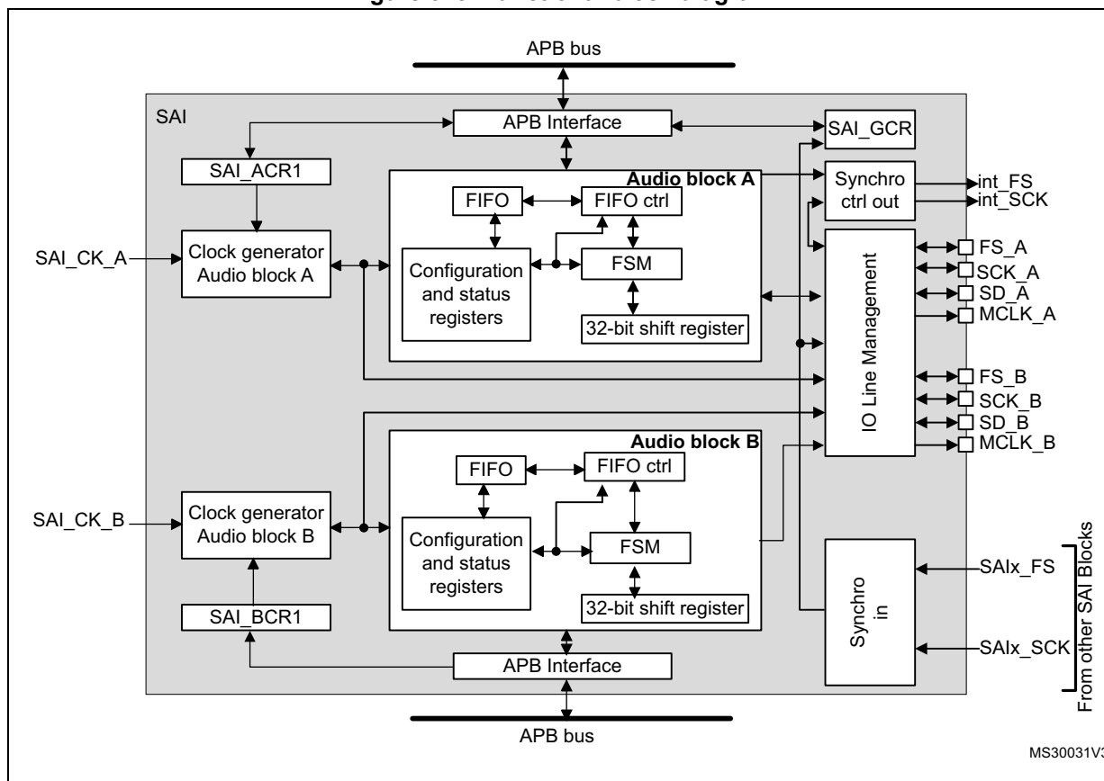
Figure 375. Functional block diagram
