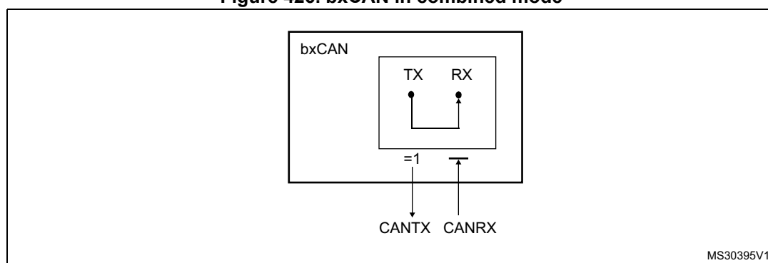
Figure 426. bxCAN in combined mode
