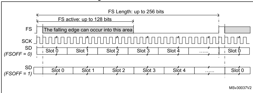
Figure 376. Audio frame
