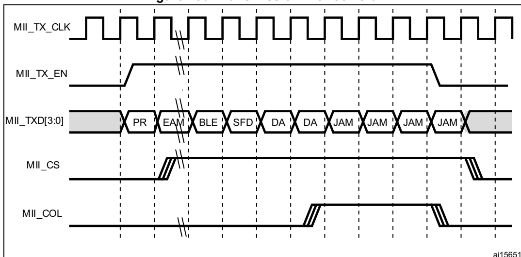
Figure 483. Transmission with collision
