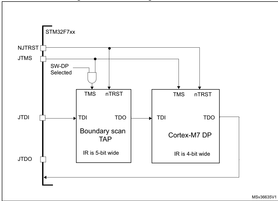
Figure 517. -JTAG Debug Port connections
