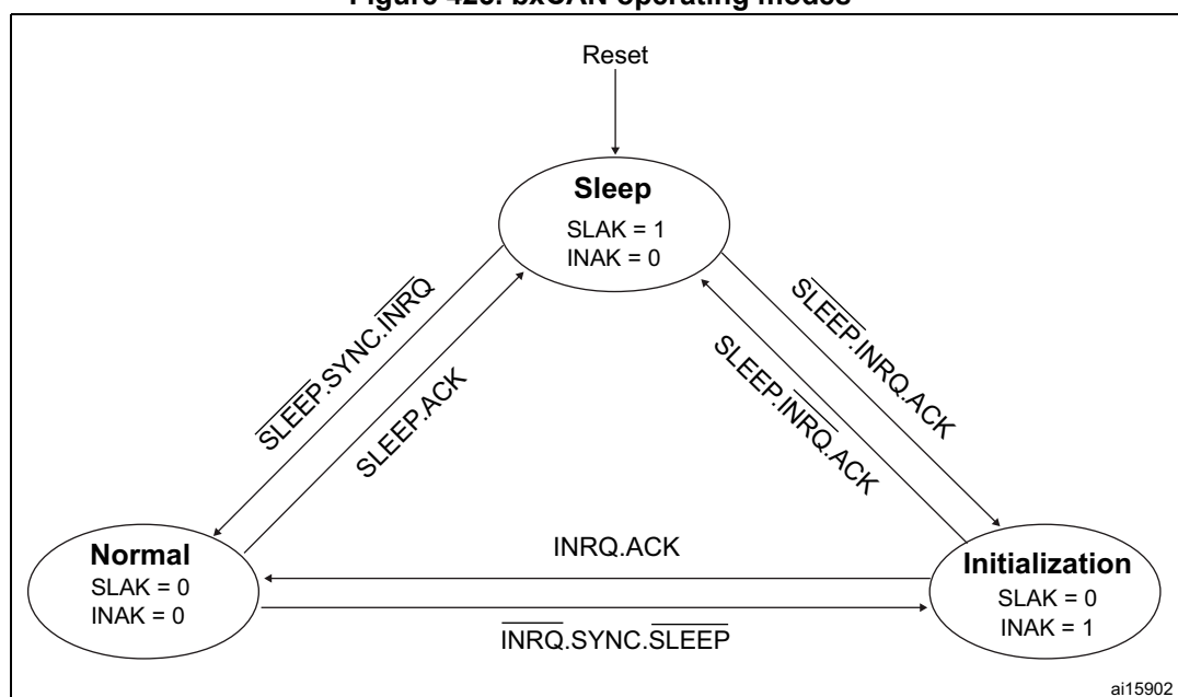
Figure 423. bxCAN operating modes
