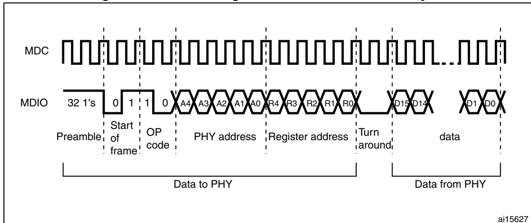
Figure 472. MDIO timing and frame structure - Read cycle
