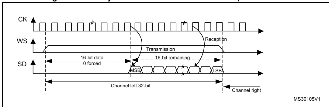
Figure 368. LSB justified 16-bit extended to 32-bit packet frame
