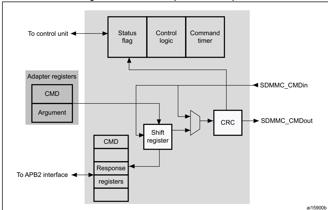
Figure 416. SDMMC adapter command path
