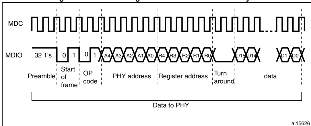
Figure 471. MDIO timing and frame structure - Write cycle
