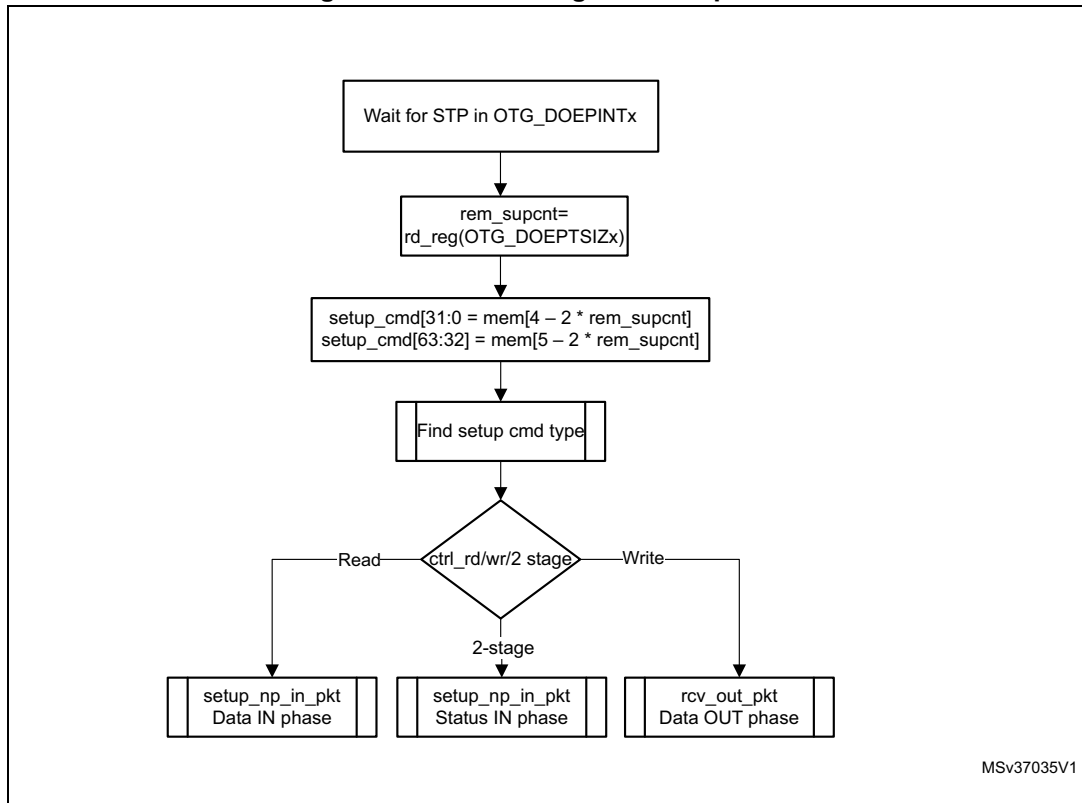
Figure 462. Processing a SETUP packet
