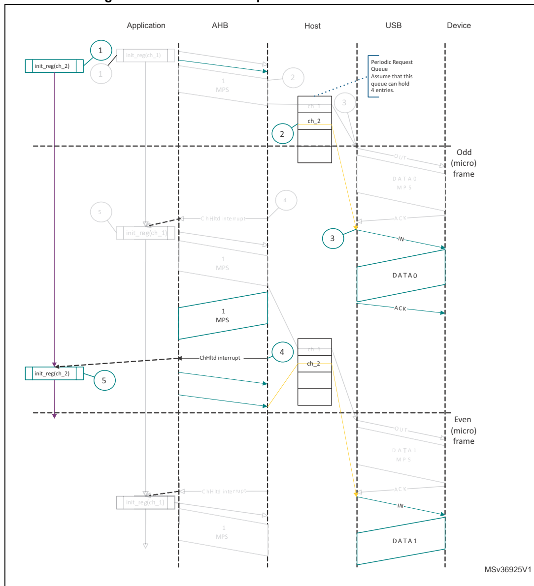
Figure 458. Normal interrupt IN transactions - DMA mode
