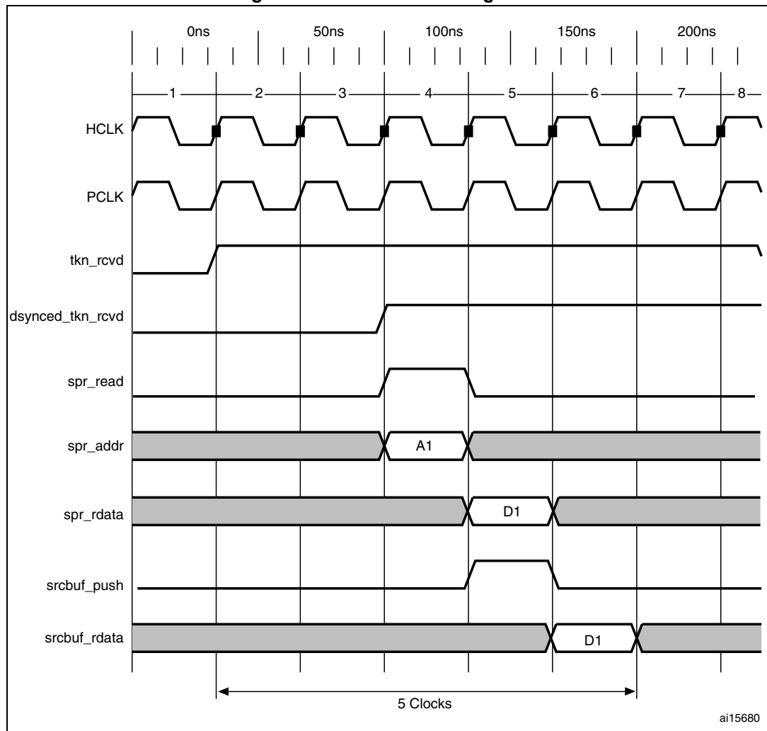
Figure 464. TRDT max timing case
