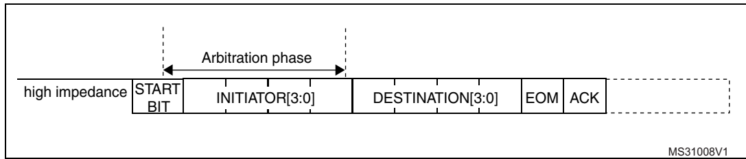
Figure 510. Arbitration phase
