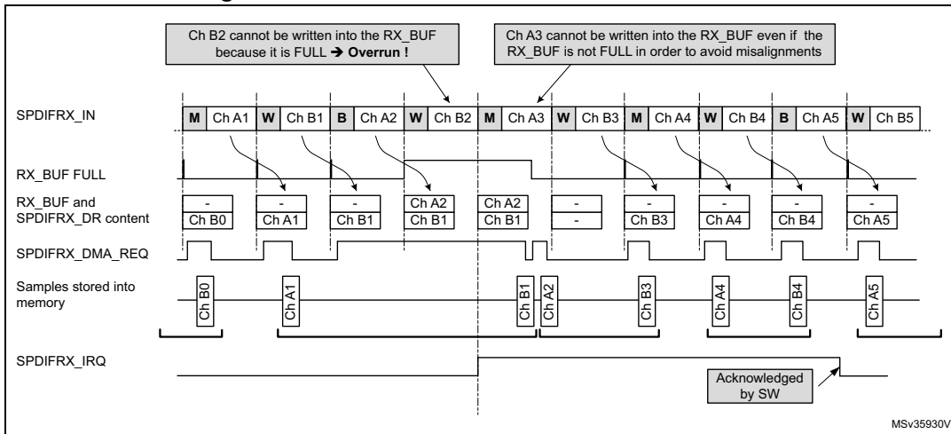
Figure 405.S/PDIF overrun error when RXSTEO = 1
