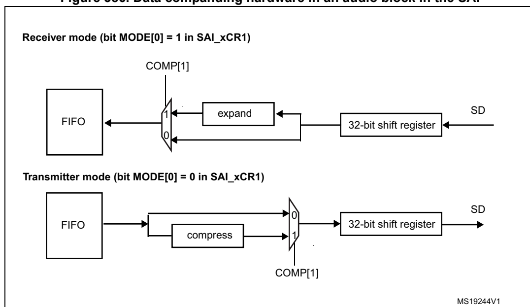
Figure 386. Data companding hardware in an audio block in the SAI
