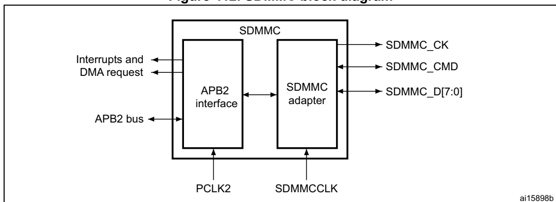
Figure 412. SDMMC block diagram
