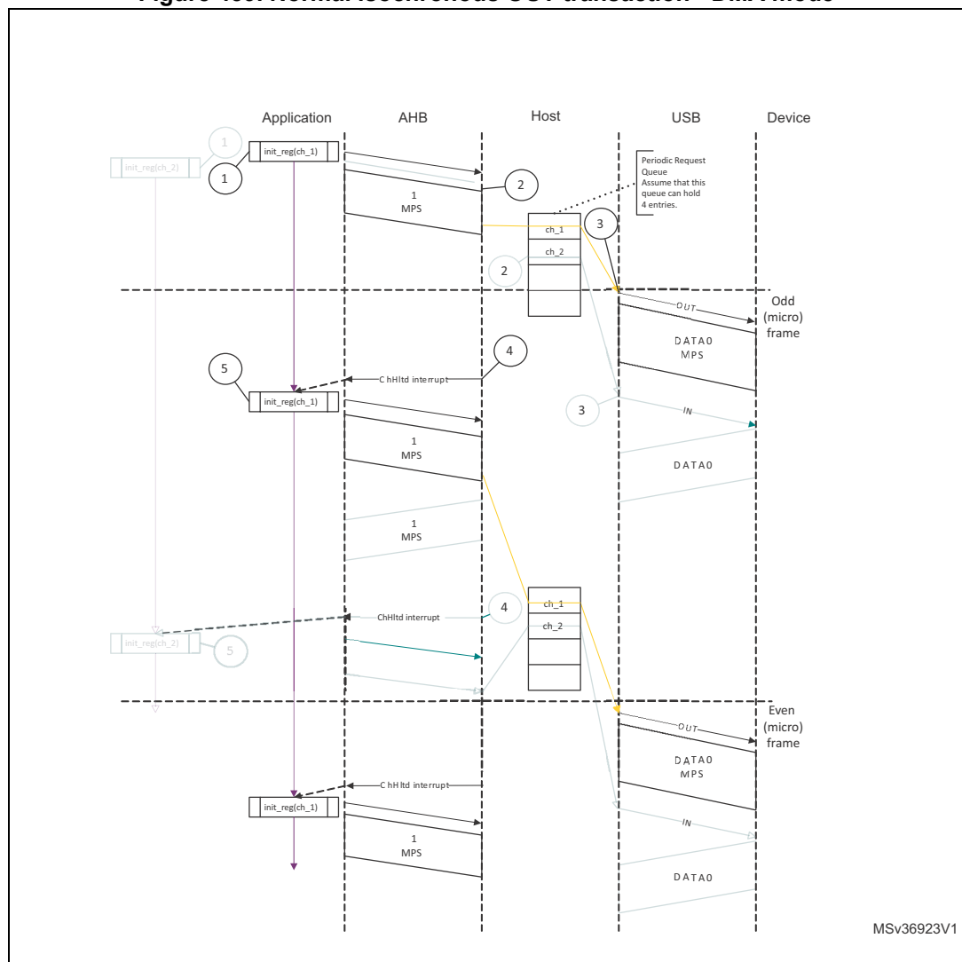
Figure 459. Normal isochronous OUT transaction - DMA mode
