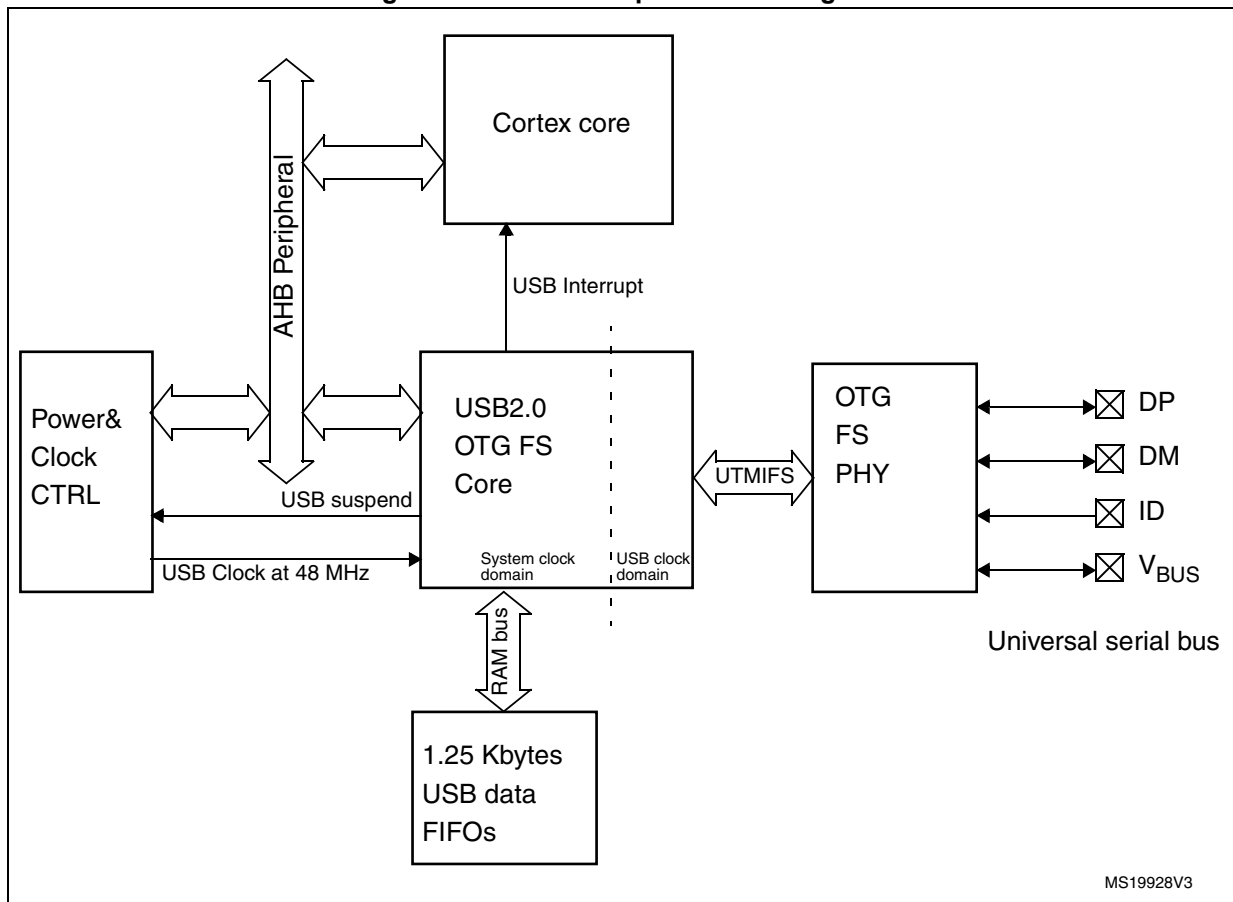
Figure 437. OTG full-speed block diagram
