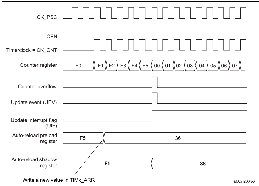
Figure 270. Counter timing diagram, update event when ARPE=1 (TIMx_ARR preloaded)
