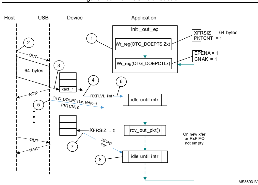
Figure 463. Bulk OUT transaction
