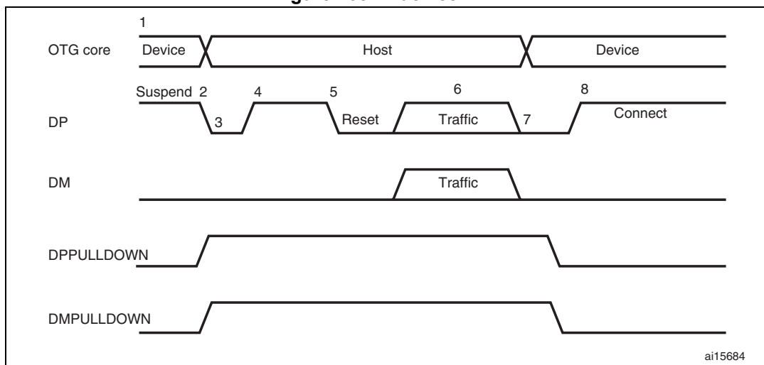
Figure 468. B-device HNP
