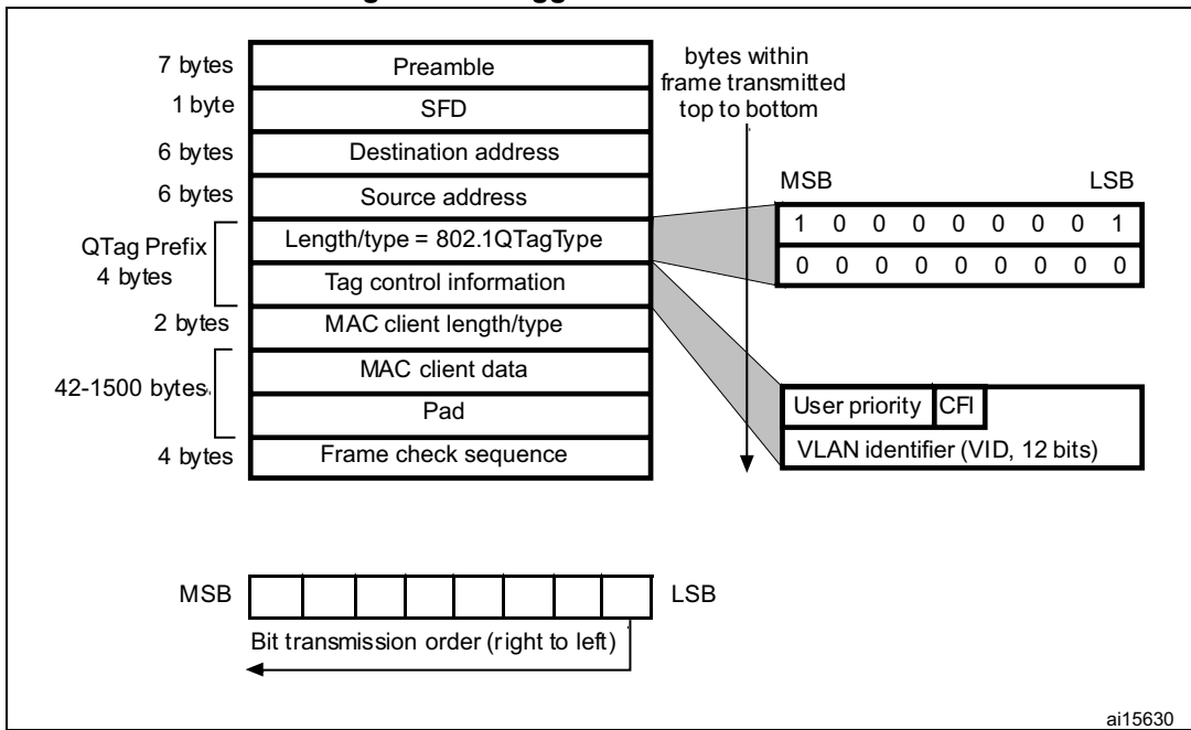
Figure 480. Tagged MAC frame format
