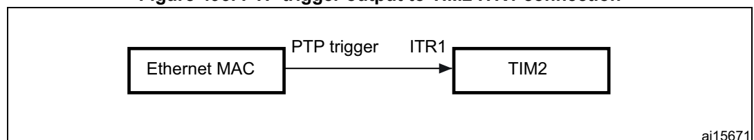
Figure 493. PTP trigger output to TIM2 ITR1 connection
