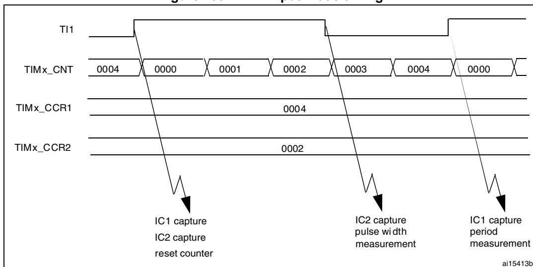
Figure 255. PWM input mode timing
