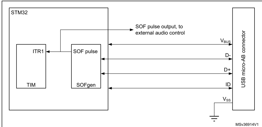
Figure 442. SOF connectivity (SOF trigger output to TIM and ITR1 connection)
