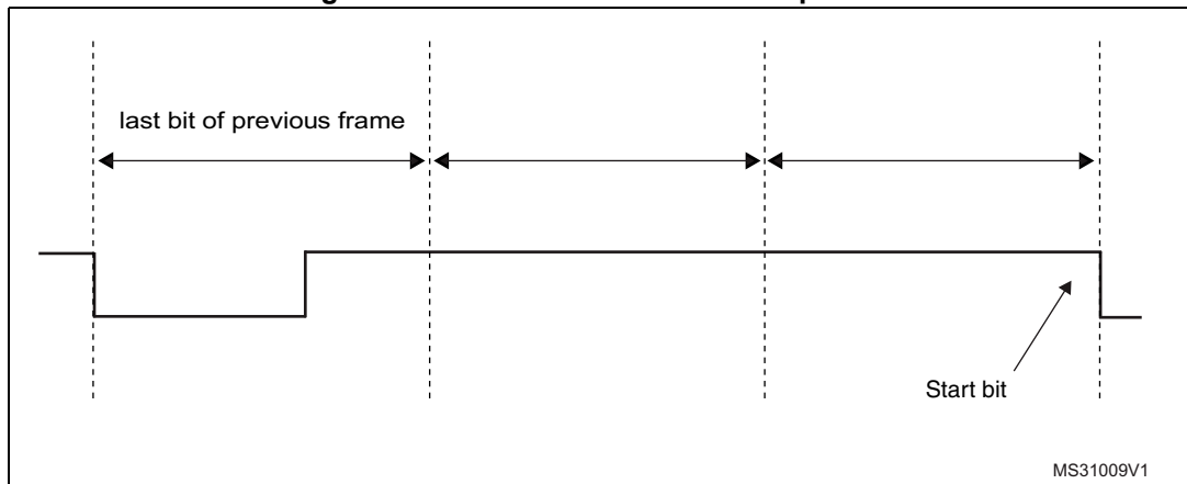
Figure 511. SFT of three nominal bit periods
