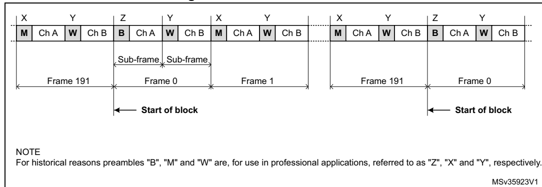
Figure 393.S/PDIF block format
