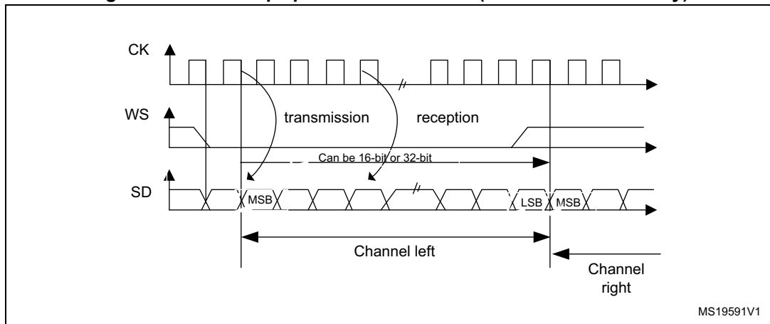
Figure 355. I 2 S Philips protocol waveforms (16/32-bit full accuracy)
