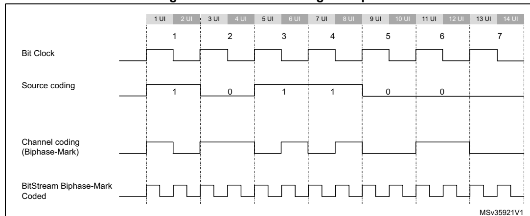
Figure 395. Channel coding example
