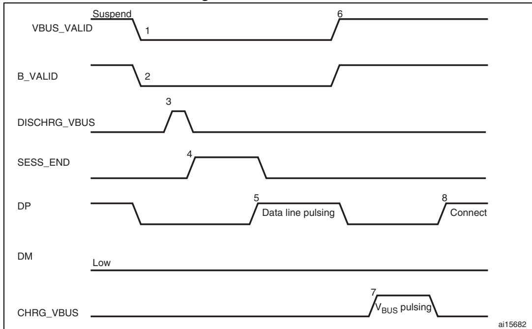
Figure 466. B-device SRP
