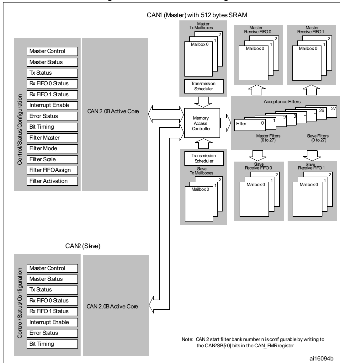
Figure 422. Dual CAN block diagram
