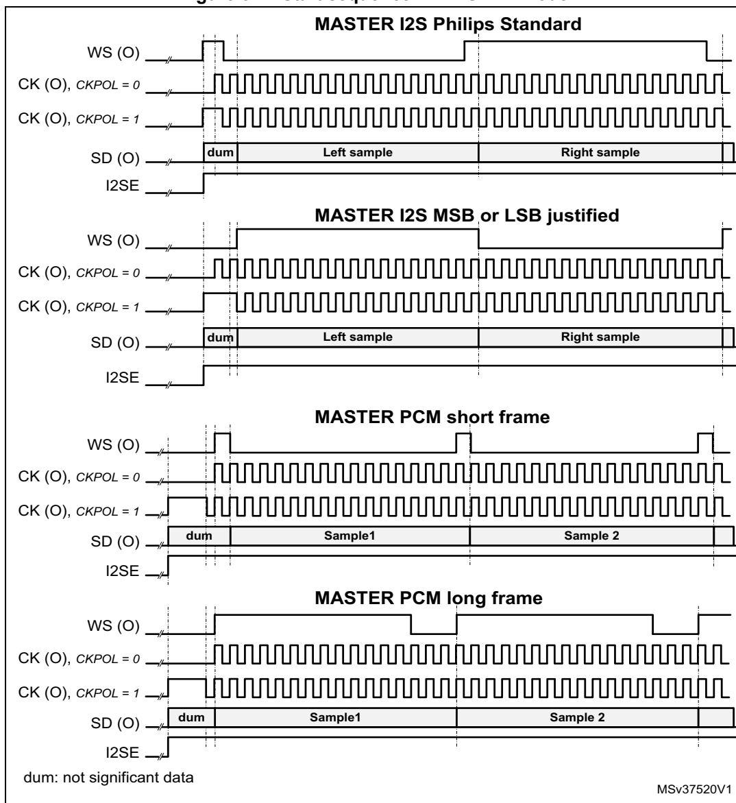
Figure 372. Start sequence in MASTER mode
