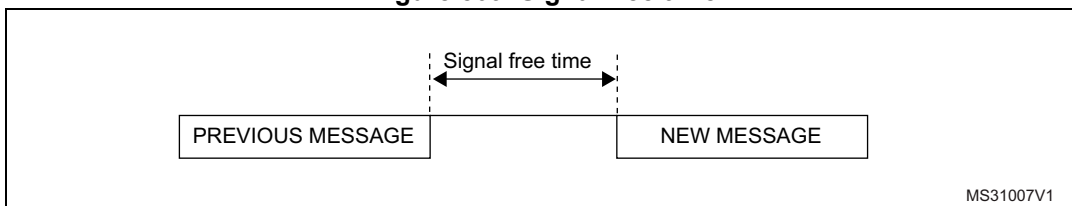
Figure 509. Signal free time
