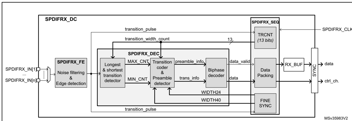
Figure 396.SPDI FRX_DC Decoder
