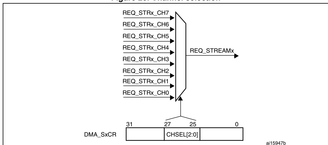
Figure 23. Channel selection
