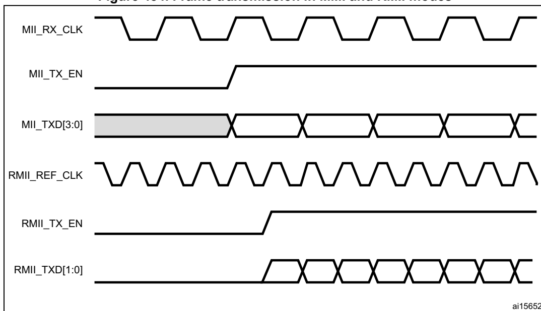
Figure 484. Frame transmission in MII and RMII modes
