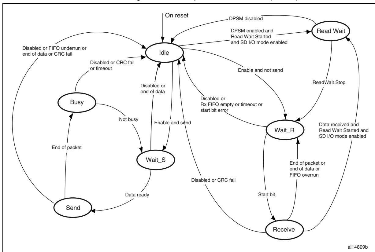
Figure 420. Data path state machine (DPSM)
