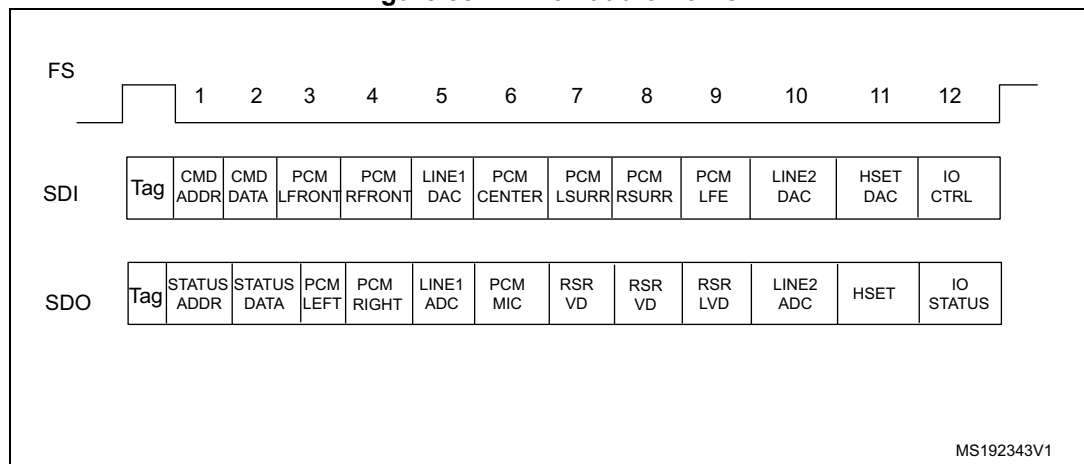
Figure 382. AC'97 audio frame
