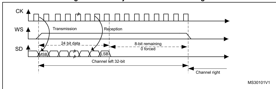
Figure 362. MSB justified 24-bit frame length
