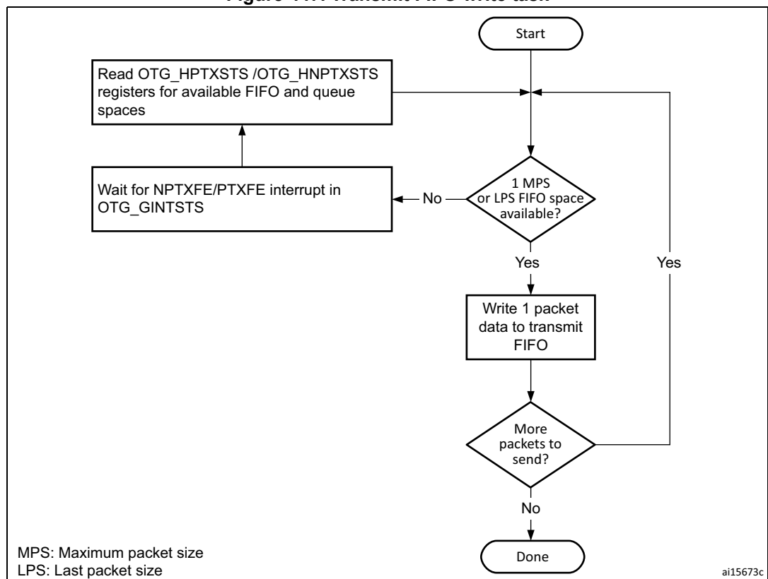
Figure 447. Transmit FIFO write task
