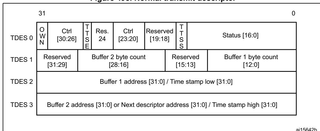
Figure 498. Normal transmit descriptor
