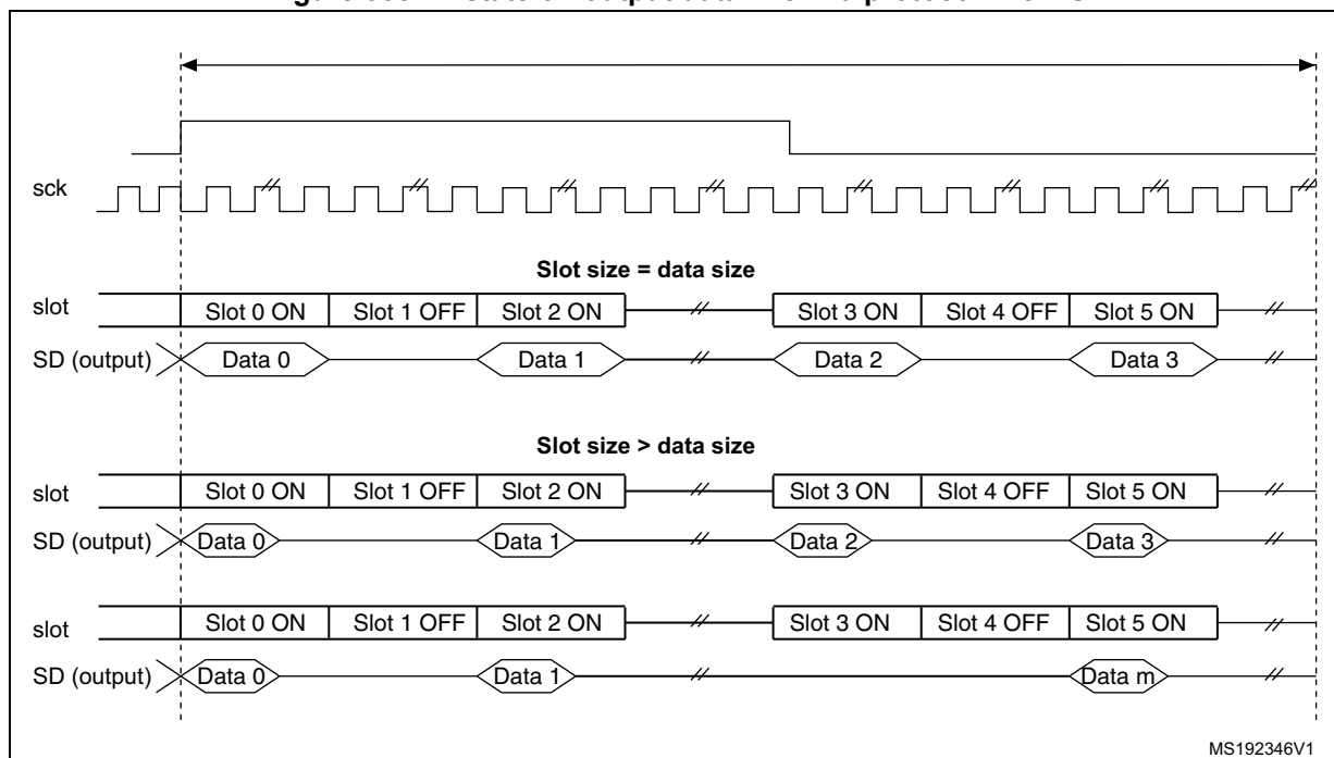
Figure 388. Tristate on output data line in a protocol like I2S
