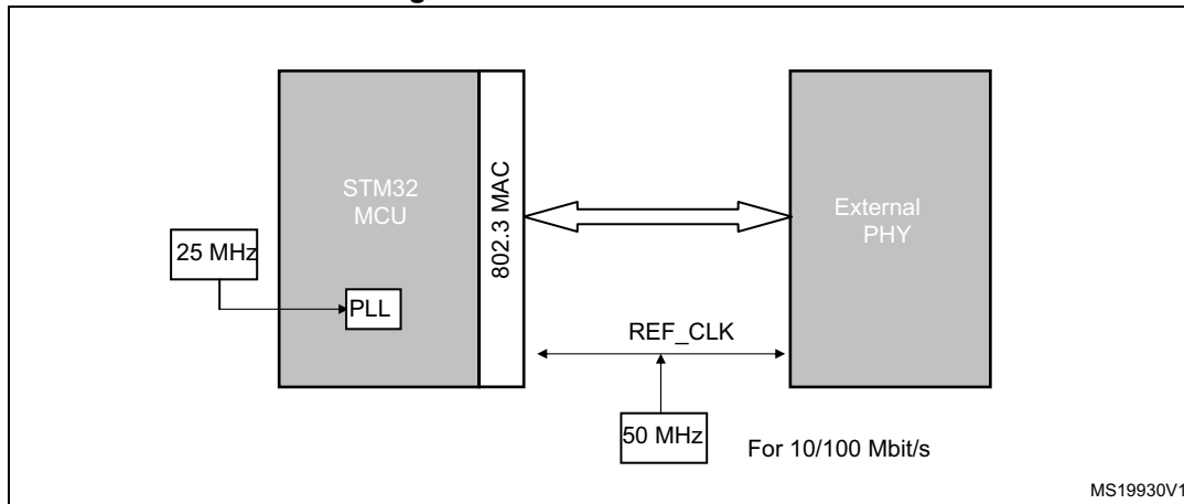
Figure 476. RMII clock sources-
