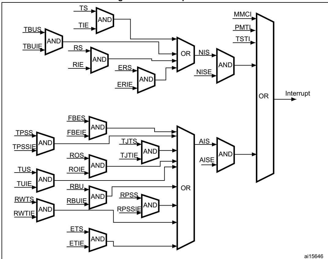
Figure 503. Interrupt scheme
