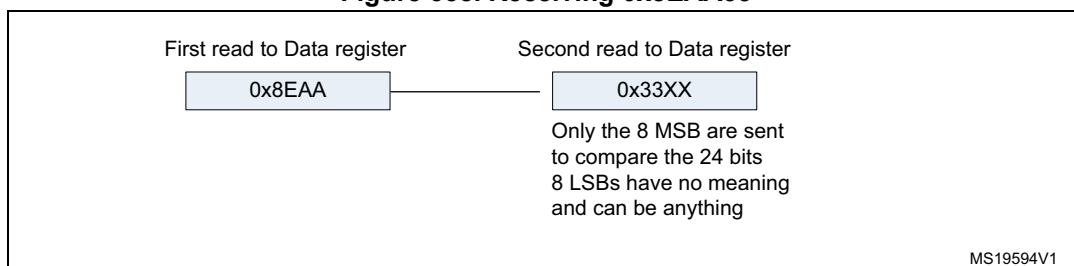
Figure 358. Receiving 0x8EAA33
