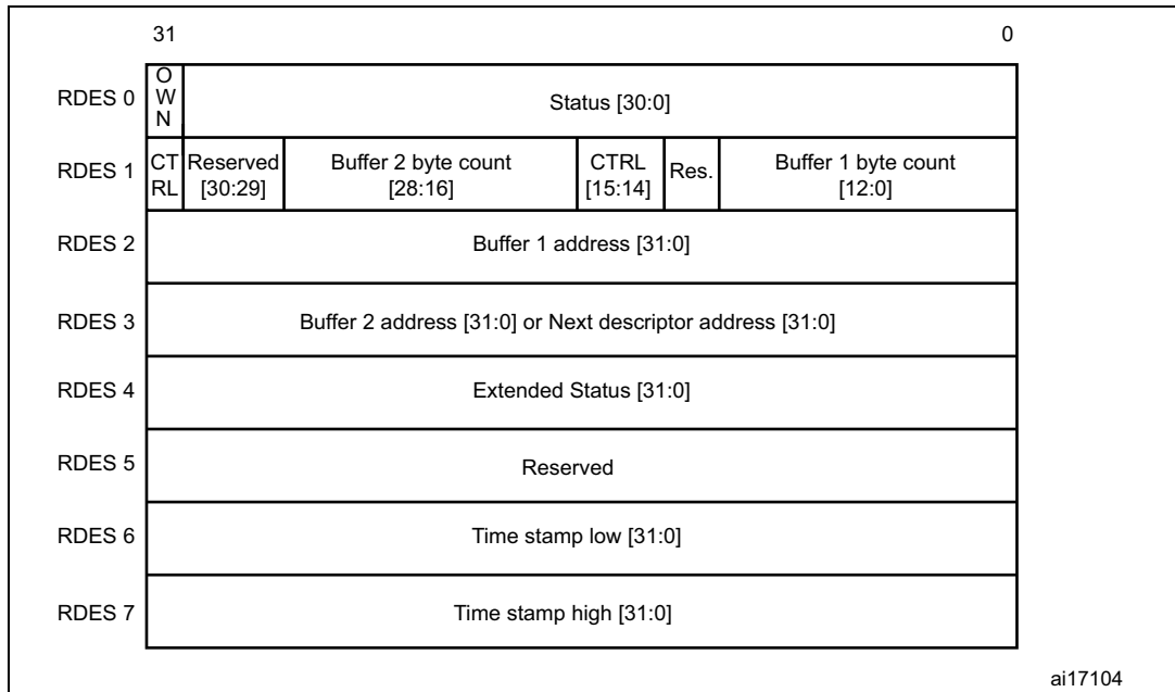
Figure 502. Enhanced receive descriptor field format with IEEE1588 time stamp enabled
