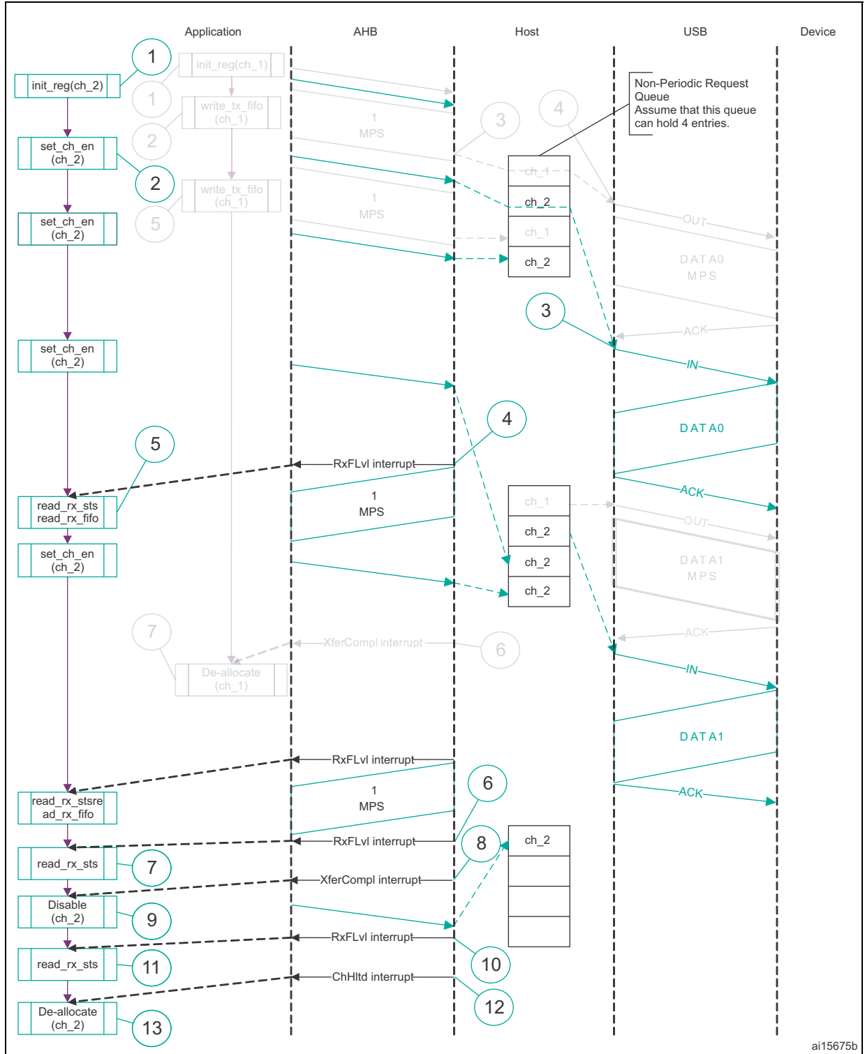
Figure 450. Bulk/control IN transactions
