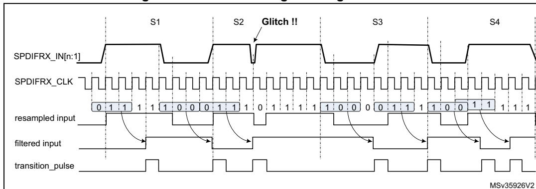
Figure 397.Noise filtering and Edge detection
