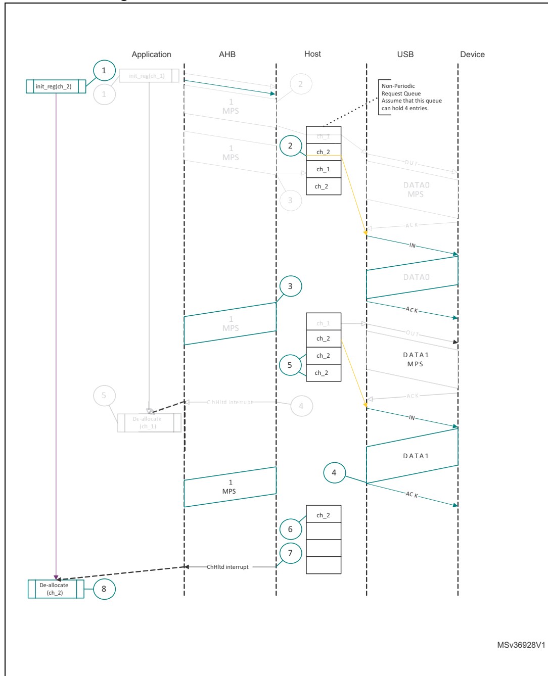
Figure 456. Normal bulk/control IN transaction - DMA
