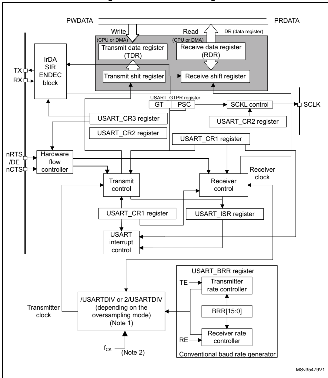
Figure 314. USART block diagram
