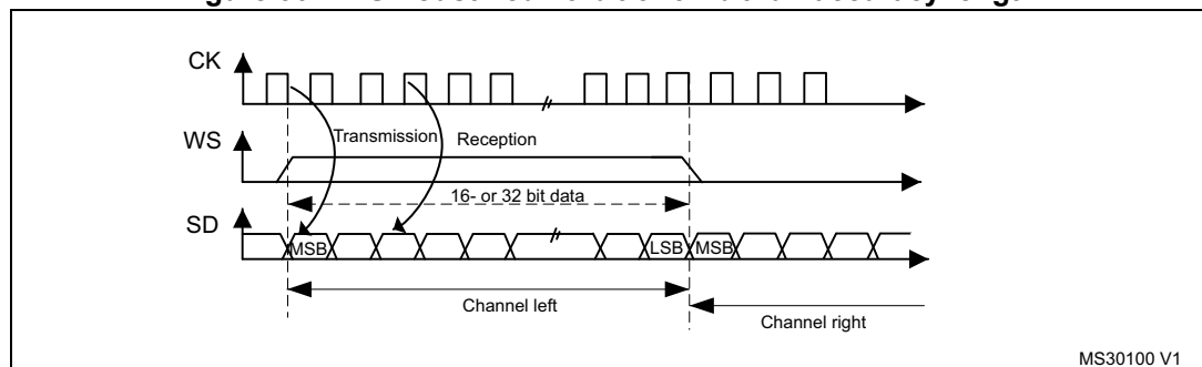
Figure 361. MSB Justified 16-bit or 32-bit full-accuracy length
