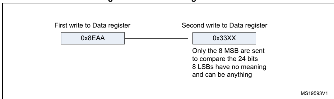
Figure 357. Transmitting 0x8EAA33
