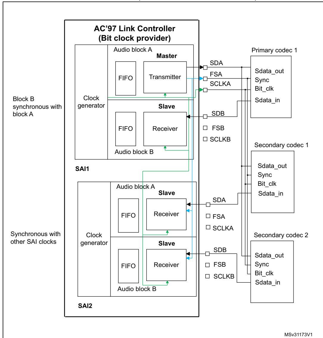
Figure 383. Example of typical AC'97 configuration on devices featuring at least 2 embedded SAIs (three external AC'97 decoders)
