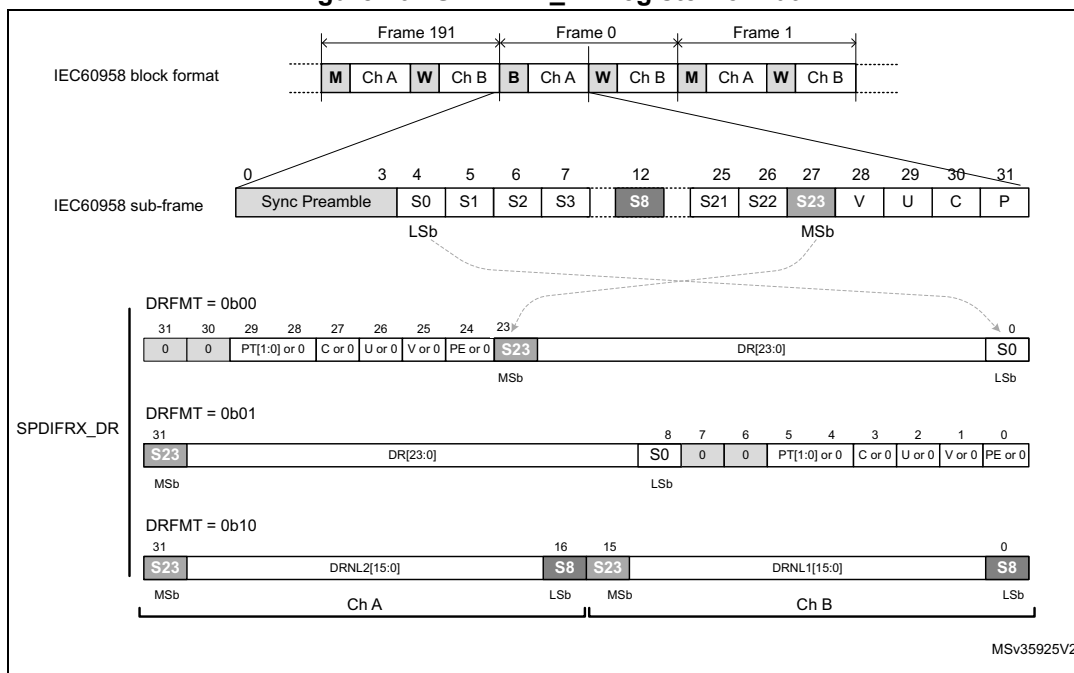
Figure 402.SPDI FRX _DR register format
