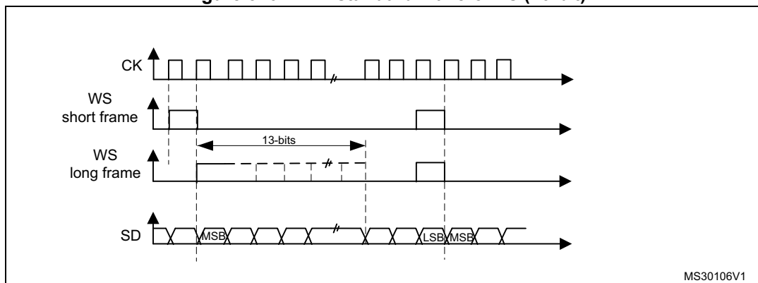
Figure 370. PCM standard waveforms (16-bit)
