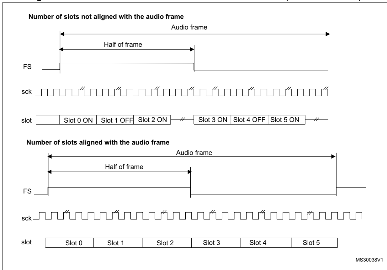
Figure 377. FS role is start of frame + channel side identification (FSDEF = TRIS = 1)
