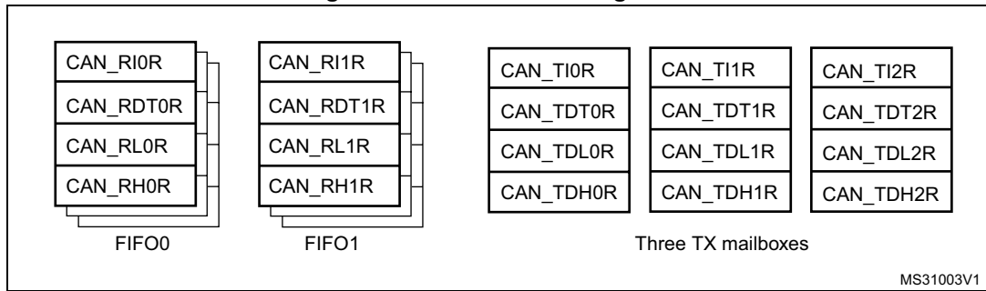
Figure 436. Can mailbox registers
