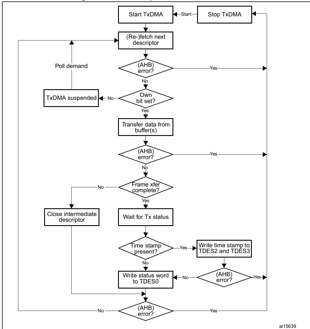
Figure 496. TxDMA operation in default mode
