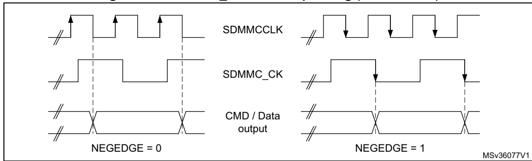
Figure 415. SDMMC_CK clock dephasing (BYPASS = 0)
