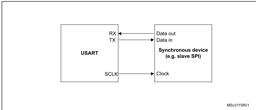
Figure 325. USART example of synchronous transmission
