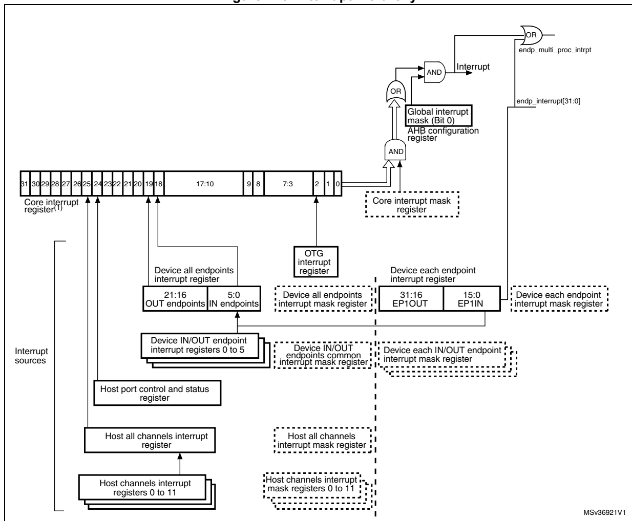
Figure 446. Interrupt hierarchy
