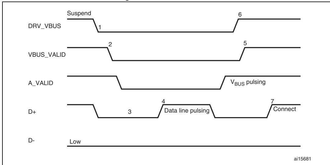
Figure 465. A-device SRP
