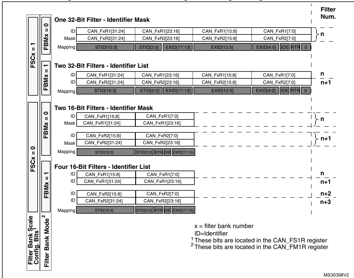
Figure 429. Filter bank scale configuration - register organization
