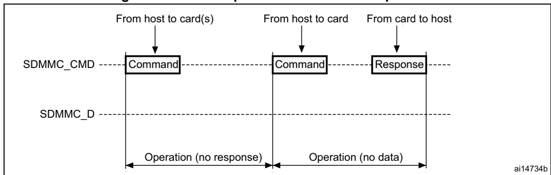
Figure 408. (Multiple) block read operation
