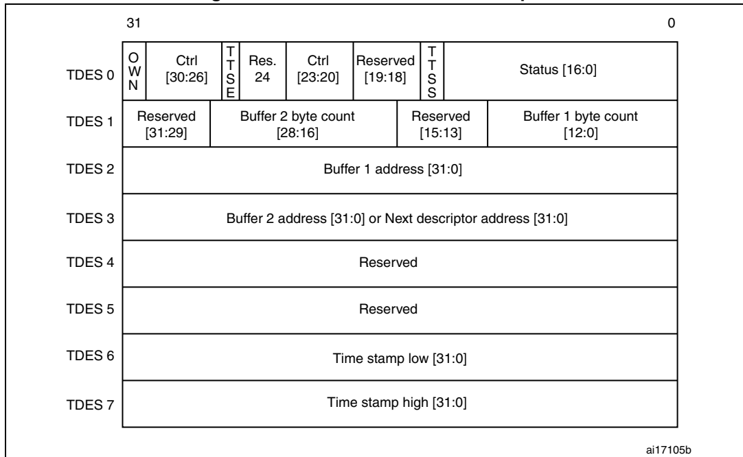
Figure 499. Enhanced transmit descriptor
