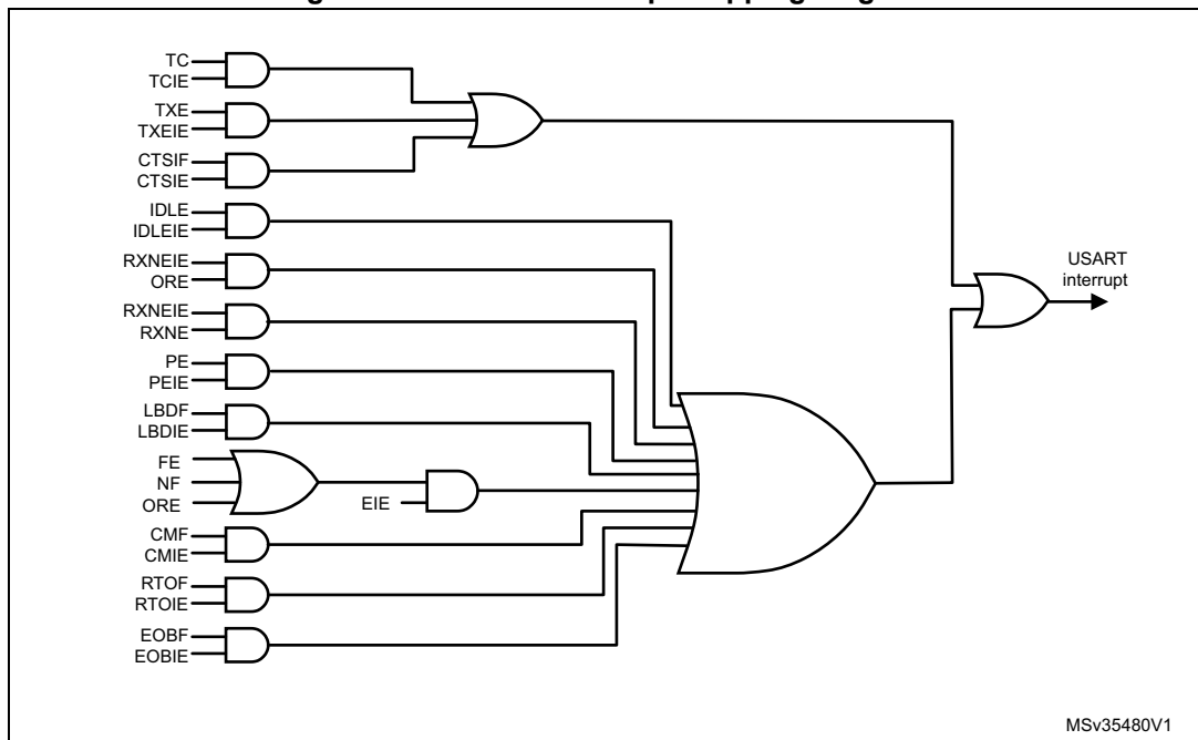
Figure 338. USART interrupt mapping diagram
