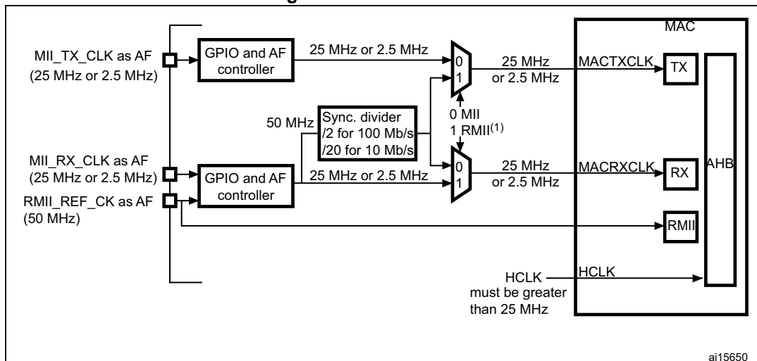
Figure 477. Clock scheme
