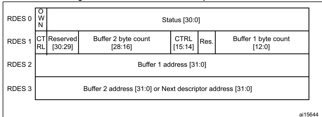
Figure 501. Normal Rx DMA descriptor structure
