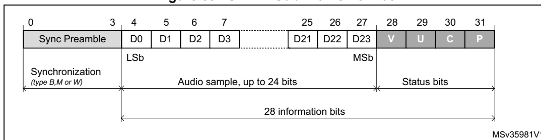
Figure 392.S/PDI F Sub-Frame Format
