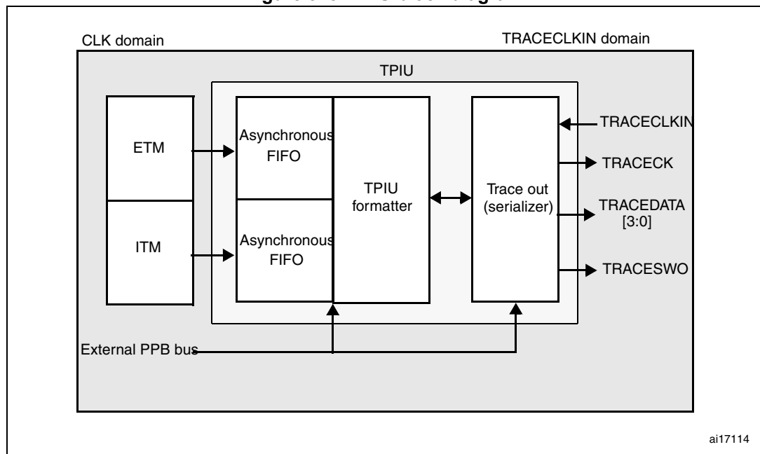
Figure 518. TPIU block diagram
