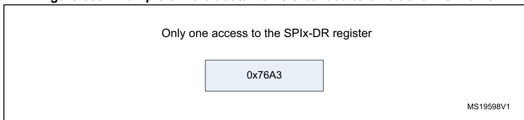
Figure 369. Example of 16-bit data frame extended to 32-bit channel frame
