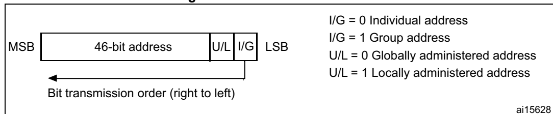
Figure 478. Address field format
