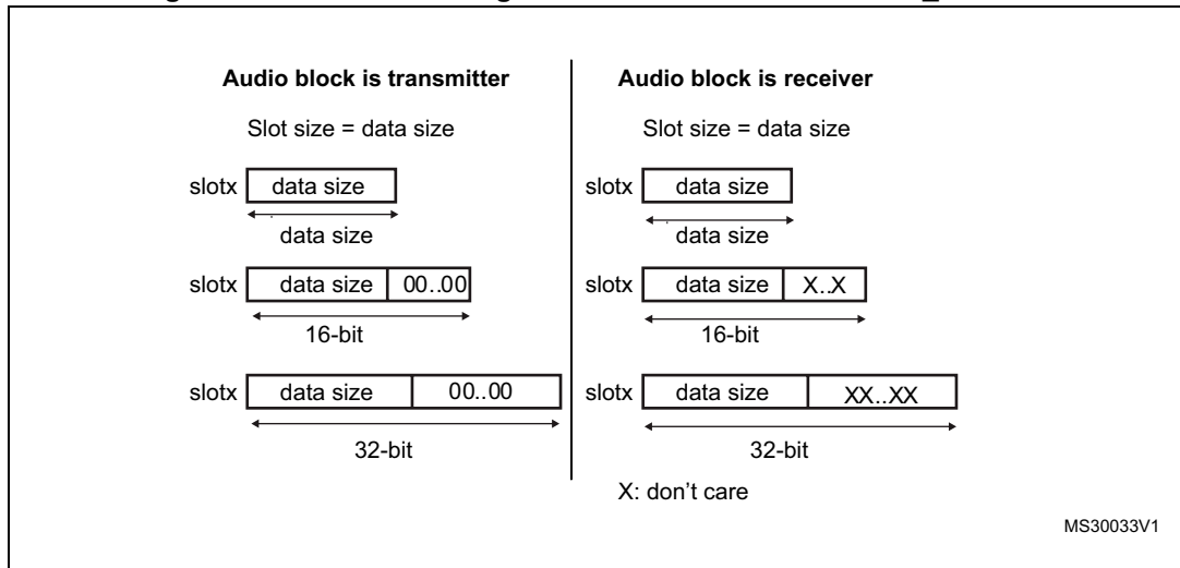
Figure 379. Slot size configuration with FBOFF = 0 in SAI_xSLOTR
