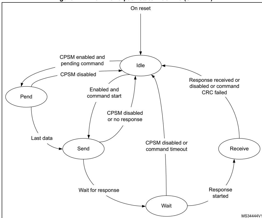
Figure 417. Command path state machine (SDMMC)
