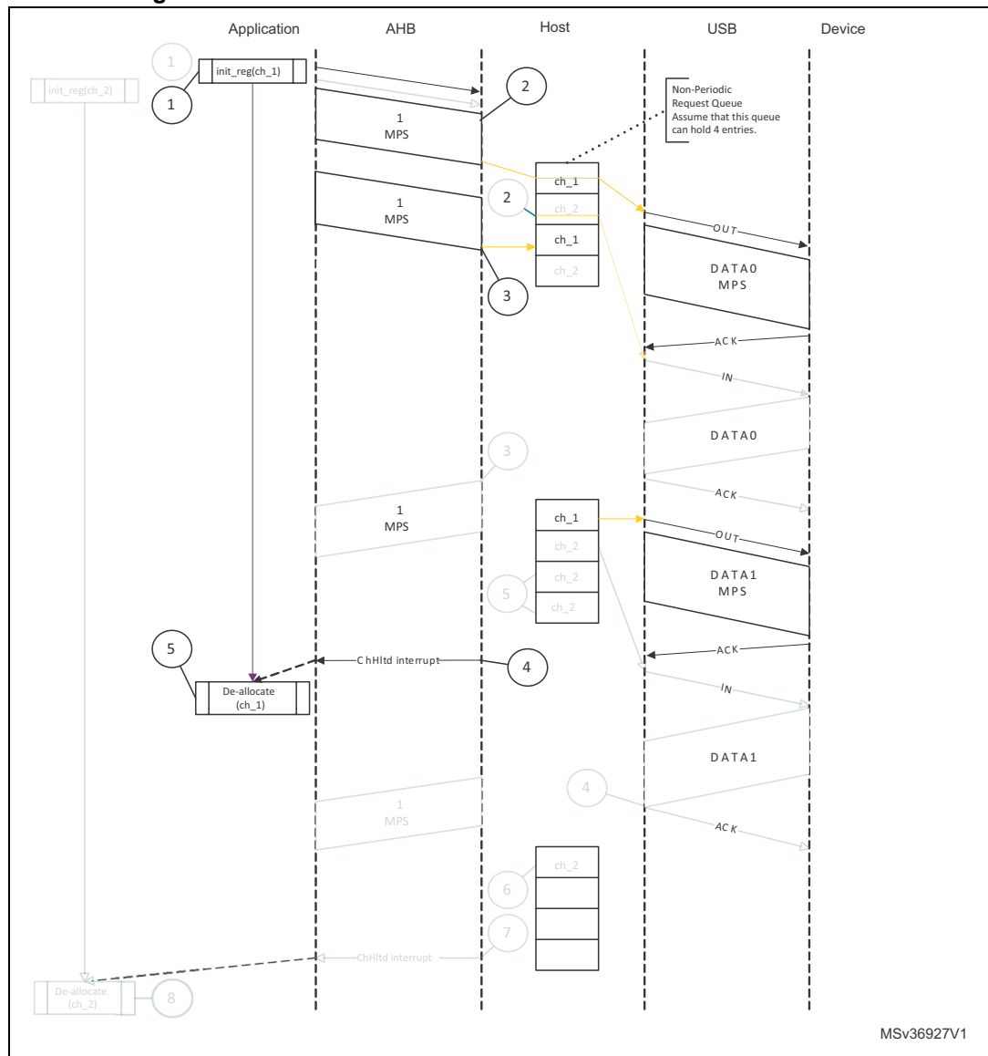
Figure 455. Normal bulk/control OUT/SETUP transactions - DMA
