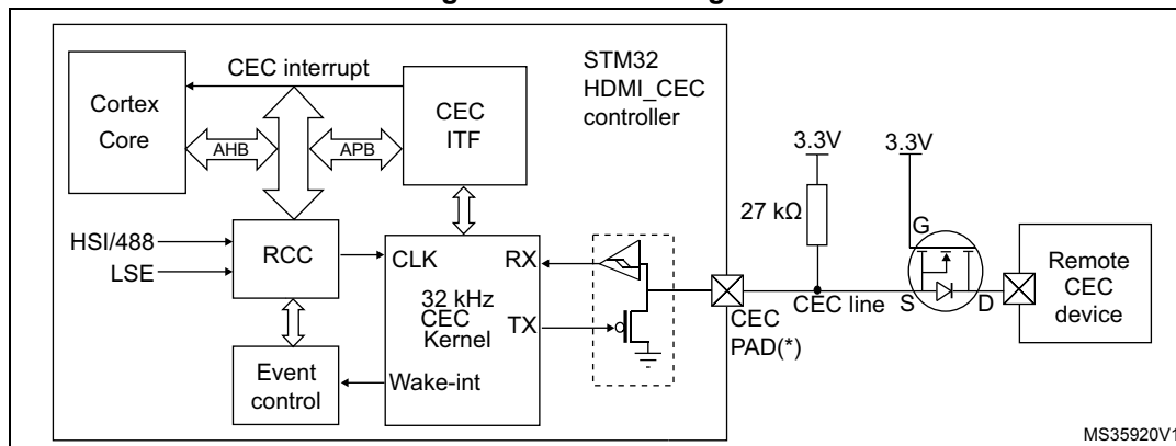
Figure 505. Block diagram
