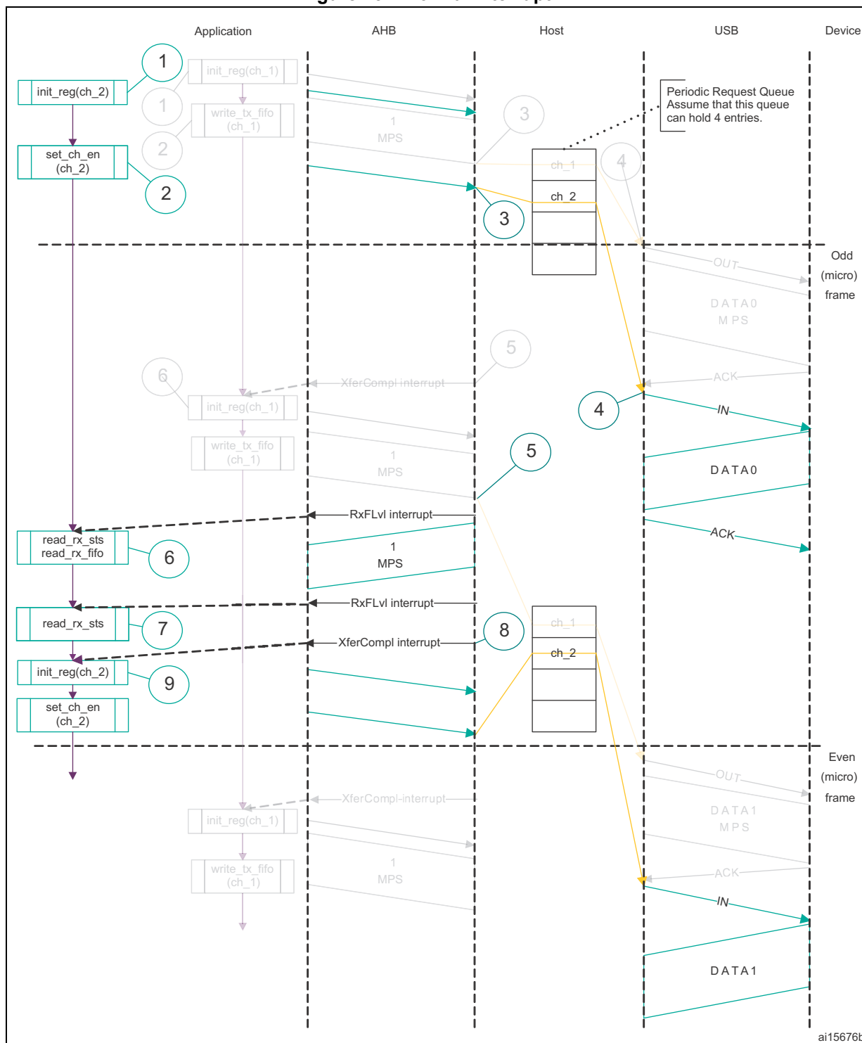
Figure 452. Normal interrupt IN
