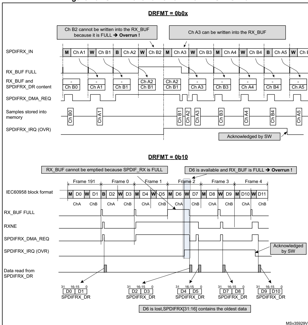
Figure 404.S/PDIF overrun error when RXSTEO = 0
