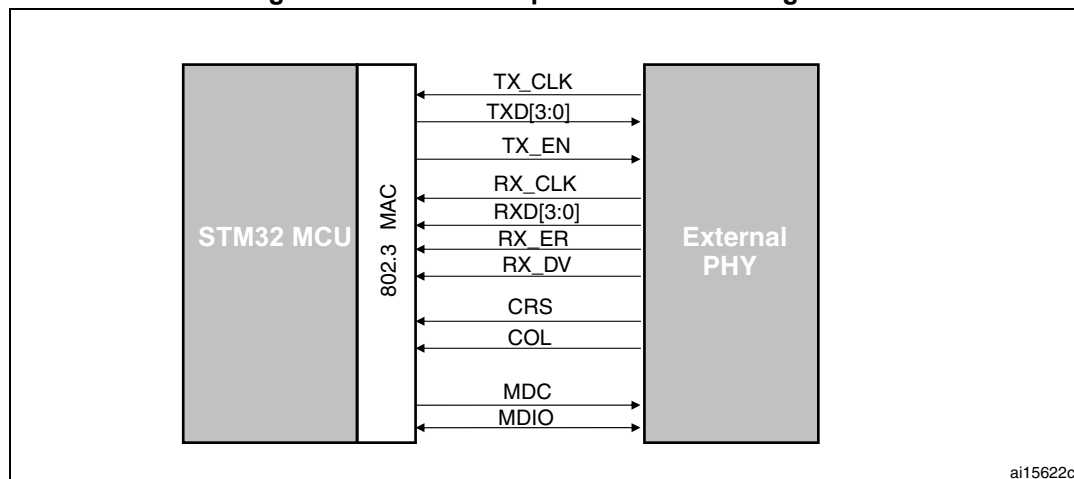
Figure 473. Media independent interface signals
