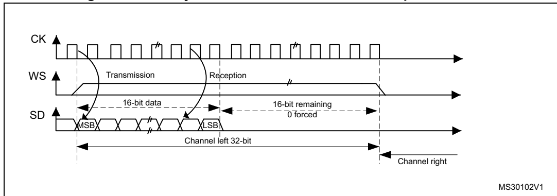
Figure 363. MSB justified 16-bit extended to 32-bit packet frame
