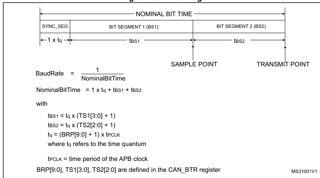
Figure 433. Bit timing
