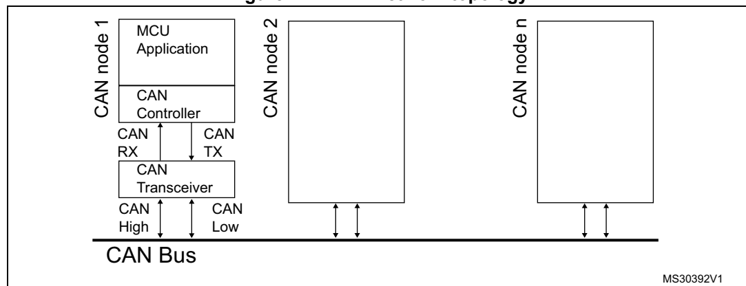
Figure 421. CAN network topology
