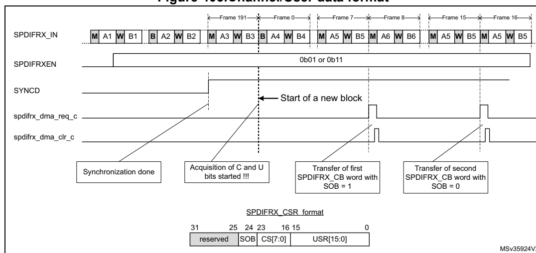
Figure 403. Channel/User data format
