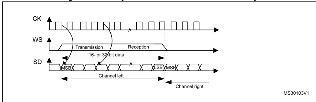
Figure 364. LSB justified 16-bit or 32-bit full-accuracy
