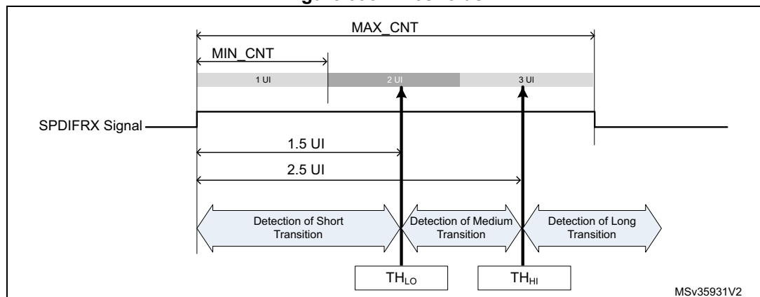
Figure 398.Thresholds
