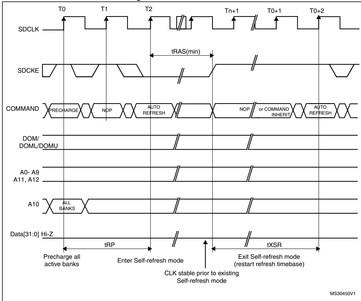
Figure 59. Self-refresh mode
