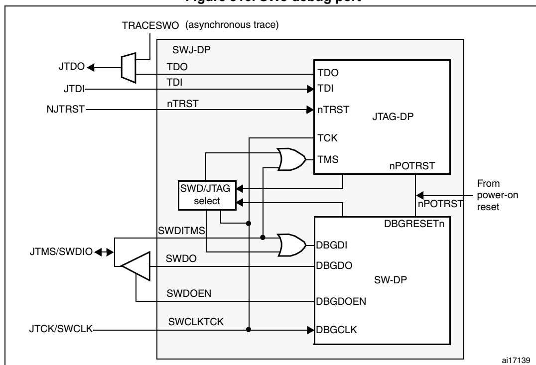
Figure 516. SWJ debug port
