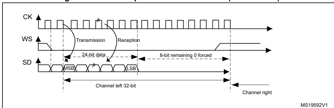
Figure 356. I 2 S Philips standard waveforms (24-bit frame)
