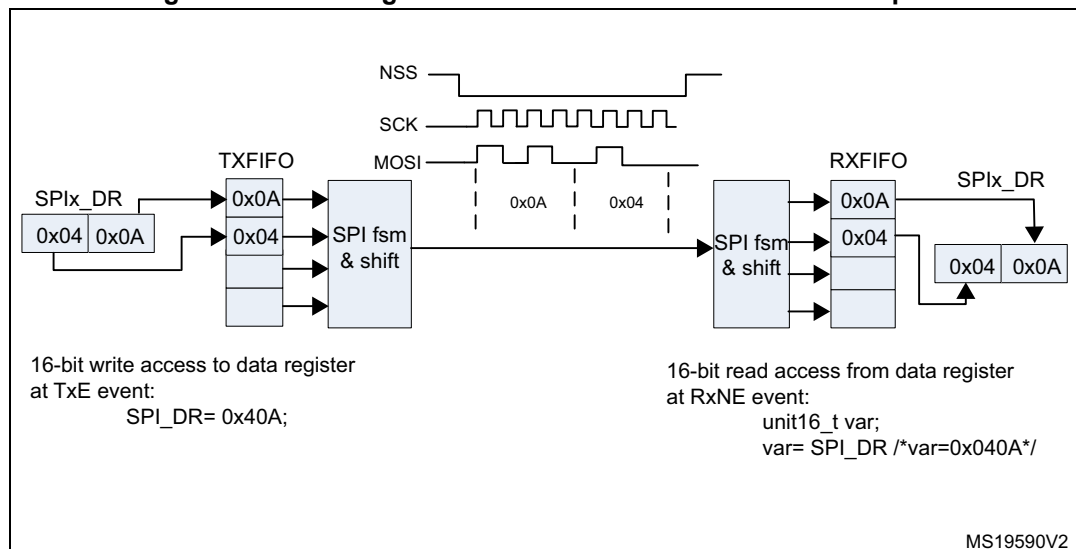
Figure 347. Packing data in FIFO for transmission and reception
