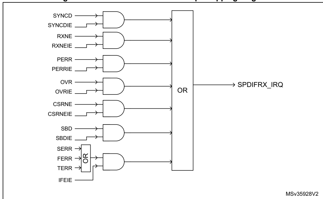
Figure 406.SPDI FRX interface interrupt mapping diagram
