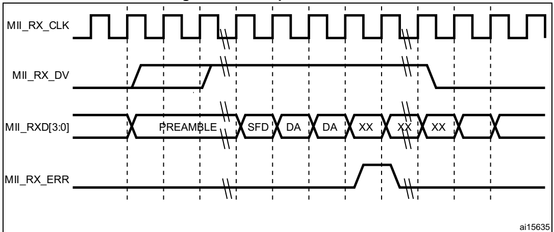
Figure 488. Reception with false carrier indication
