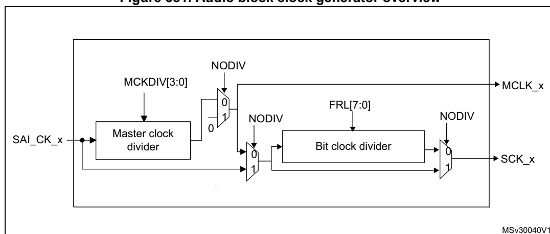
Figure 381. Audio block clock generator overview
