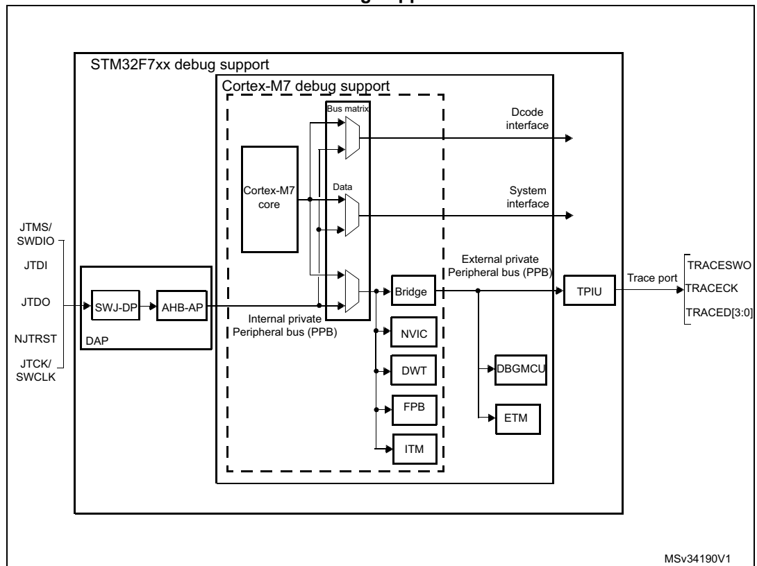
Figure 515. Block diagram of STM32 MCU and Cortex ® -M7 with FPU -level debug support
