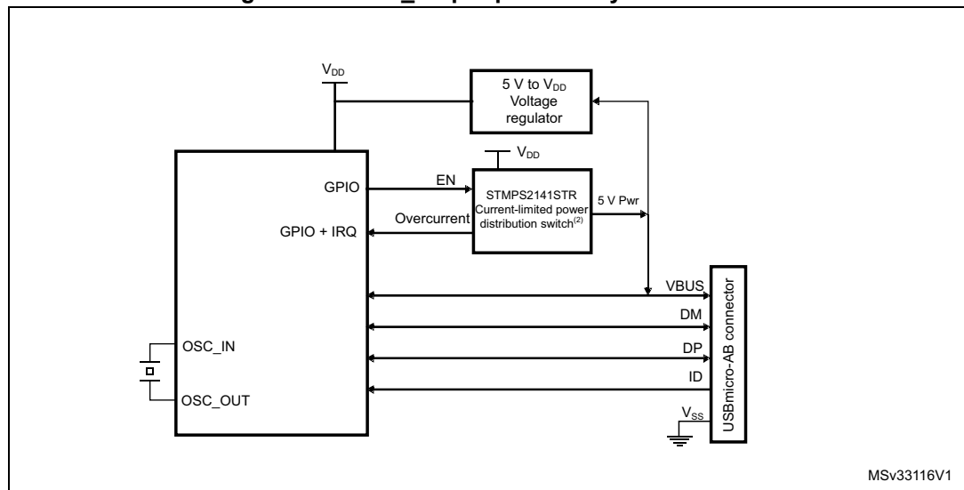
Figure 440. USB_FS peripheral-only connection
