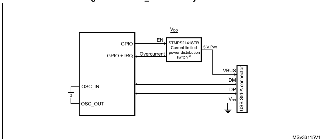
Figure 441. USB_FS host-only connection
