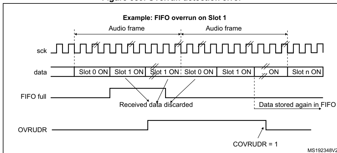
Figure 389. Overrun detection error
