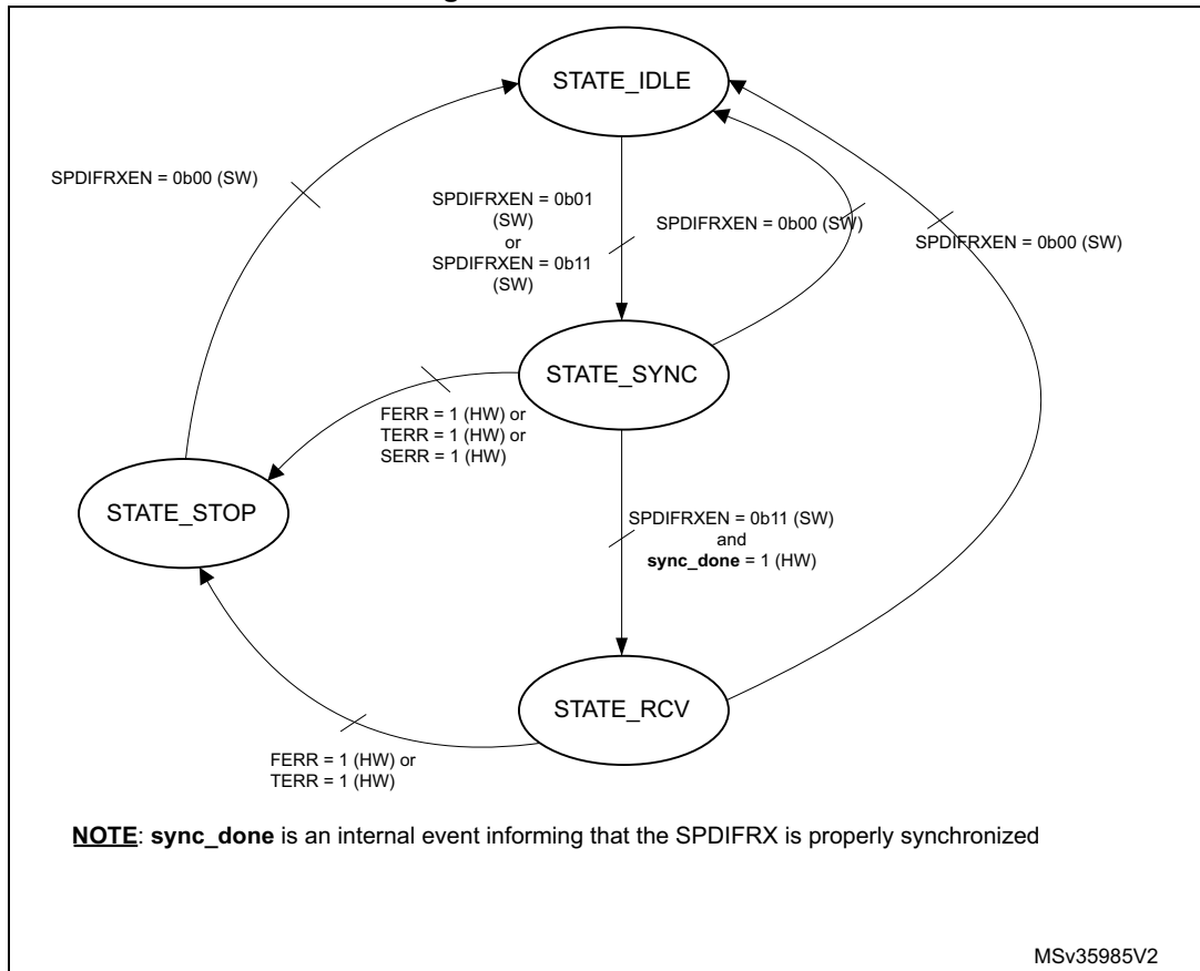
Figure 401.SPDI FRX States
