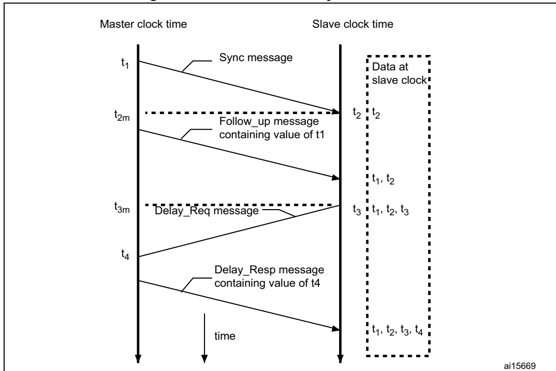
Figure 491. Networked time synchronization
