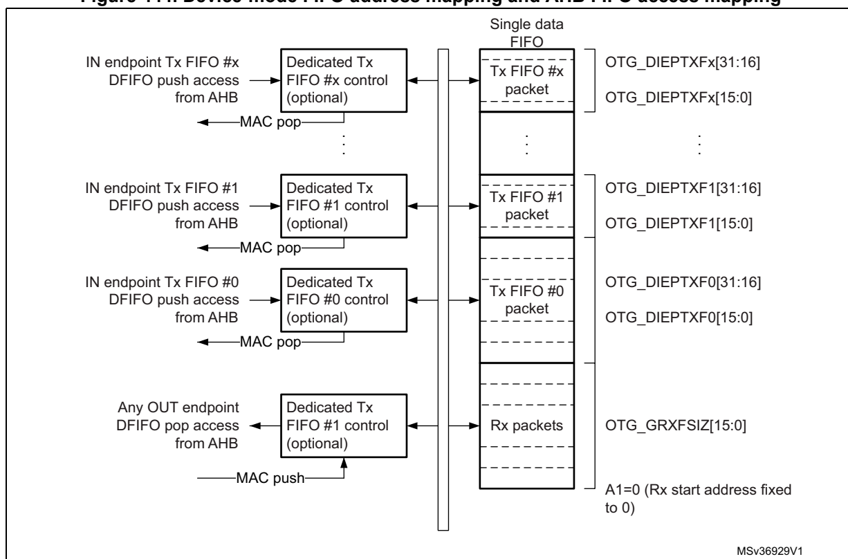
Figure 444. Device-mode FIFO address mapping and AHB FIFO access mapping
