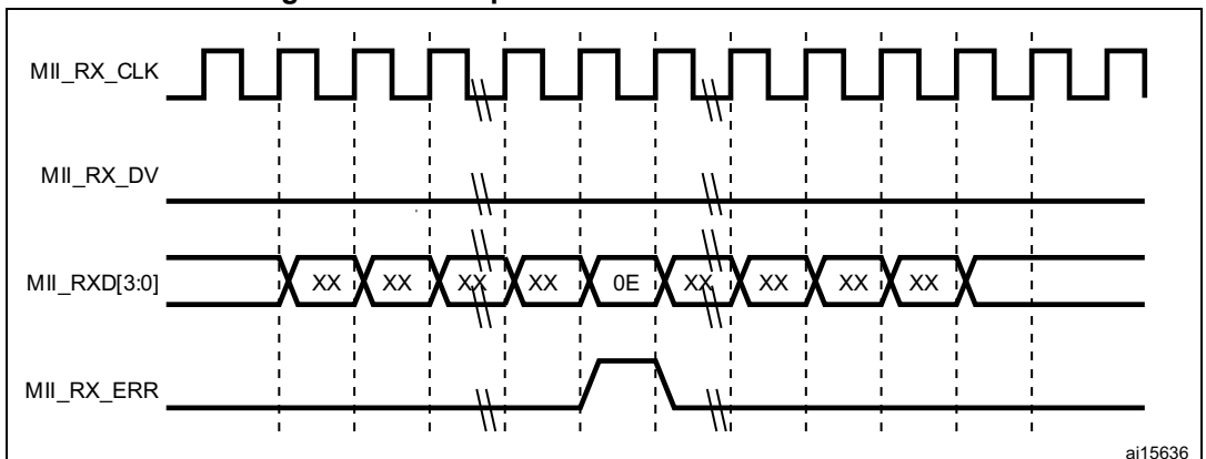
Figure 488. Reception with false carrier indication
