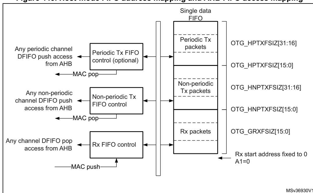
Figure 445. Host-mode FIFO address mapping and AHB FIFO access mapping
