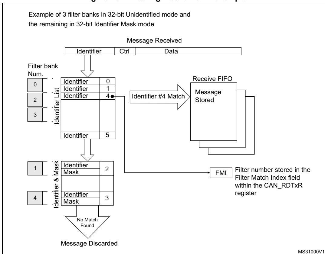
Figure 431. Filtering mechanism - example
