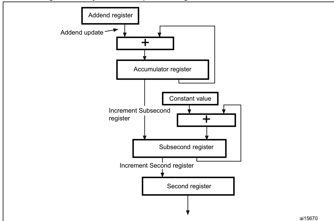
Figure 492. System time update using the Fine correction method
