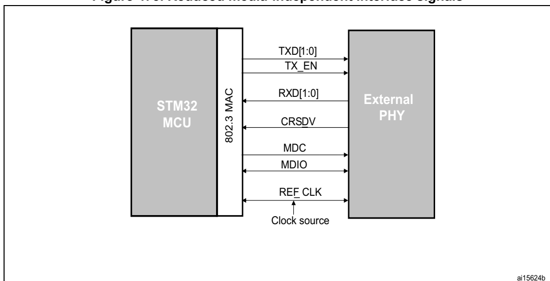
Figure 475. Reduced media-independent interface signals
