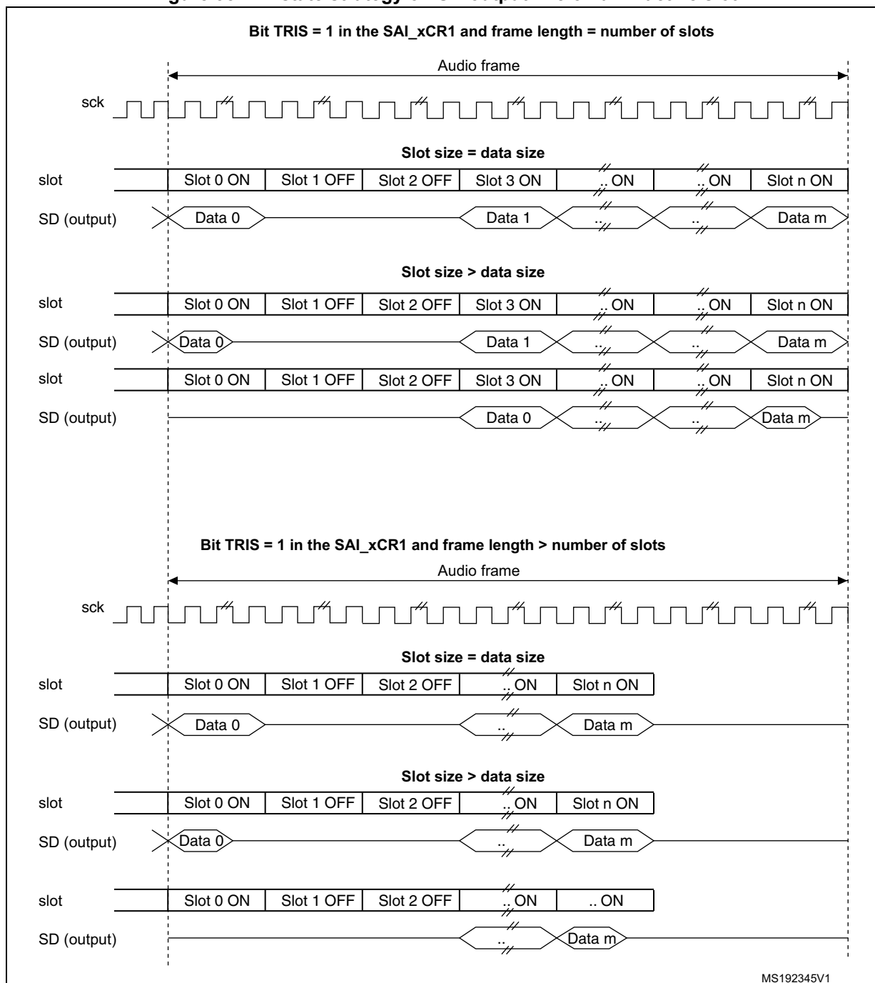
Figure 387. Tristate strategy on SD output line on an inactive slot
