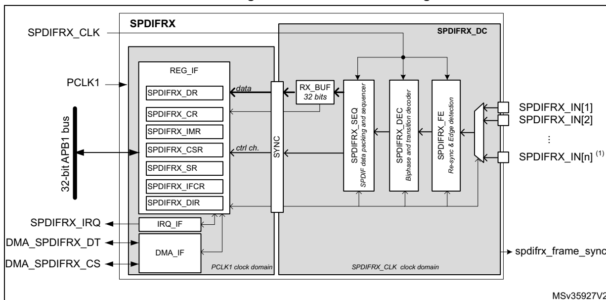
Figure 391.SPDI FRX block diagram
