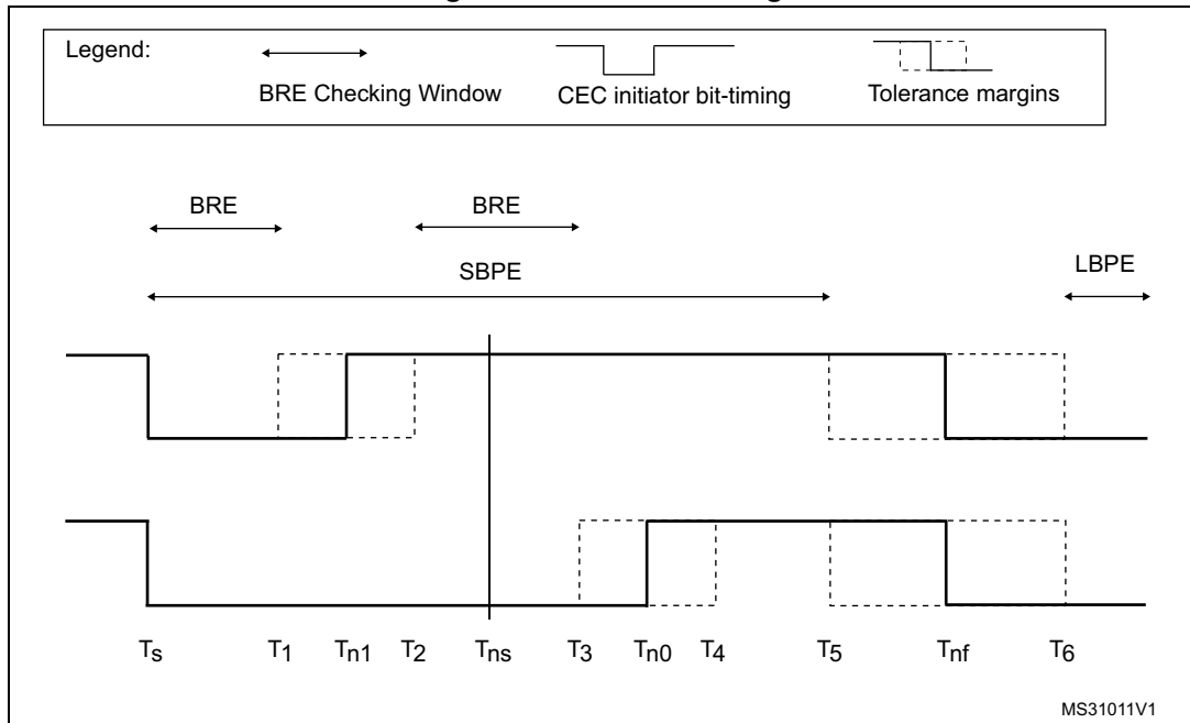
Figure 513. Error handling
