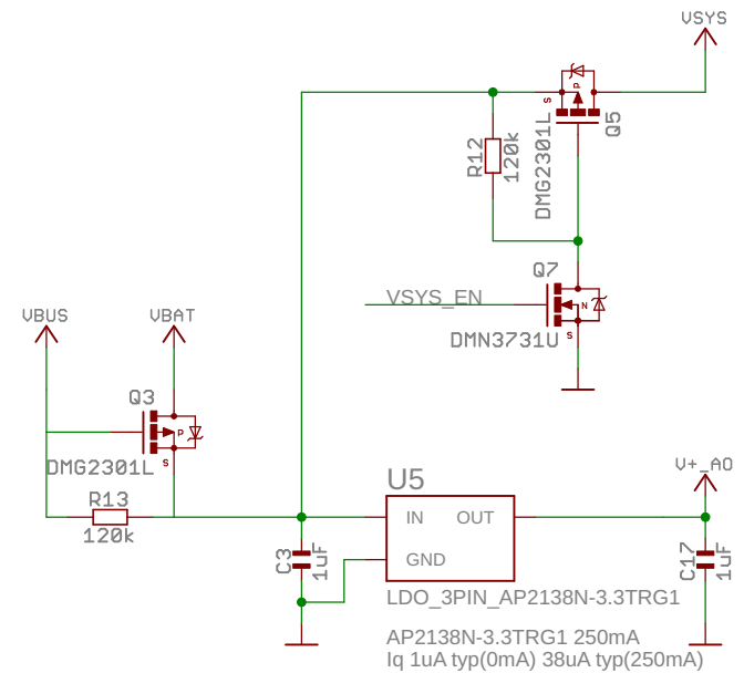
Battery and always-on 3v3 power
