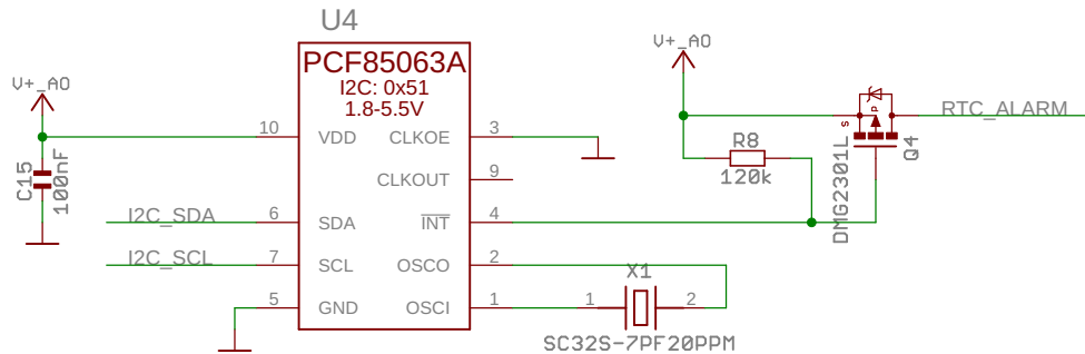
RTC with crystal
