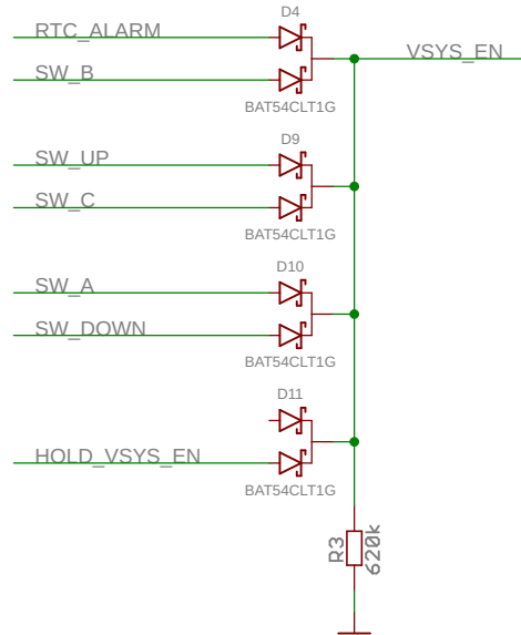
Wake from power-down connections
