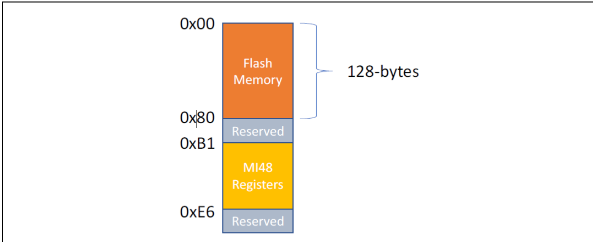
Fig. 8. Memory map of the MI48, showing the User Flash at address 0x00 – available only when bit 0 of the USER_FLASH_CTRL is set to 1.
