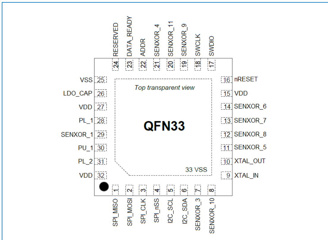
Fig. 2. MI48Ax QFN33-pin Diagram. In this version, the host is interfaced via SPI and I 2 C buses, and a DATA_READY signal.
