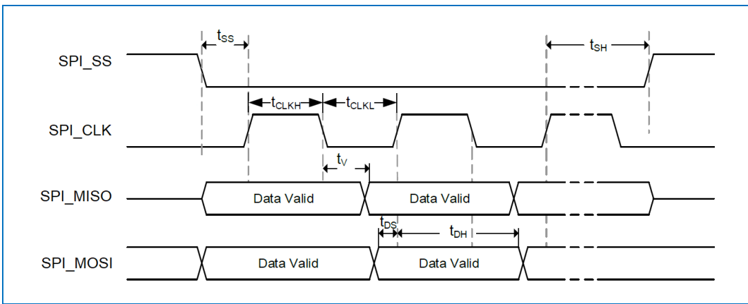
Fig. 10. SPI Interface timing diagram.
