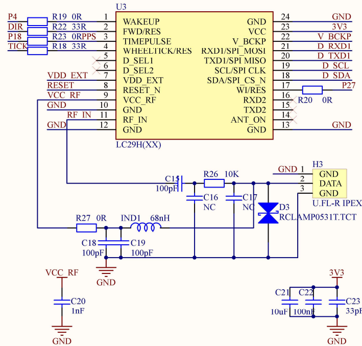
LC29H(XX) Module
