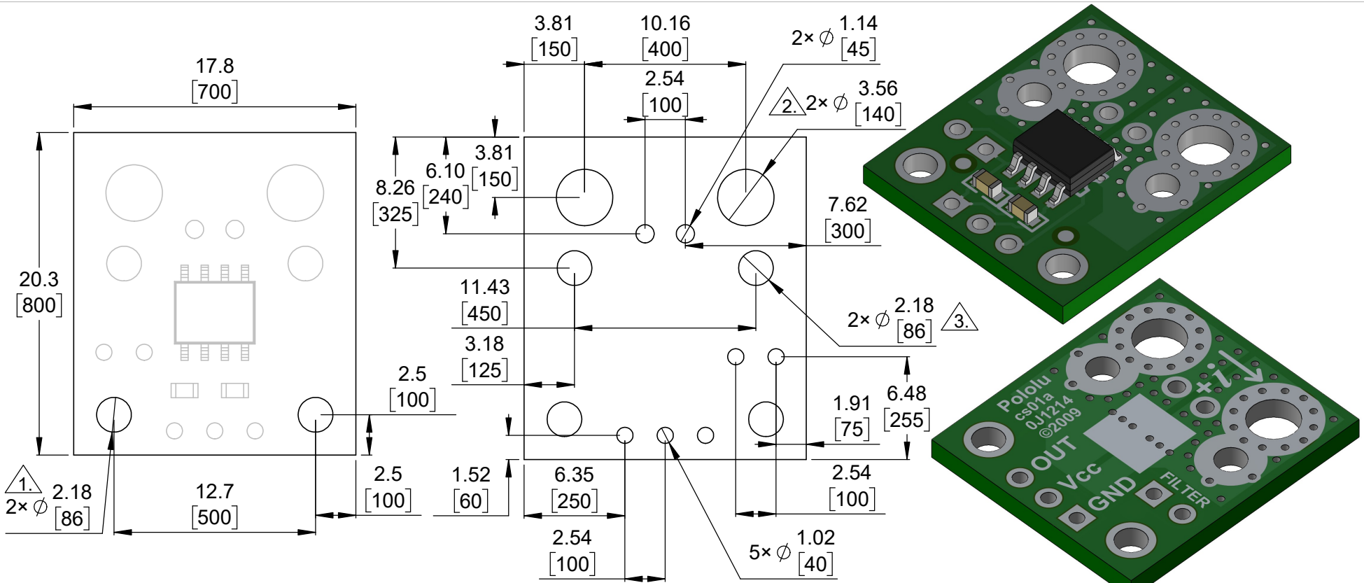
1 Board dimensions (top view) Scale 3:1
