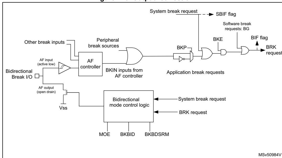
Figure 275. Output redirection
