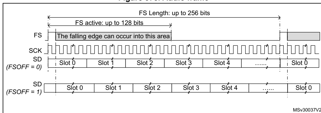
Figure 378. Audio frame
