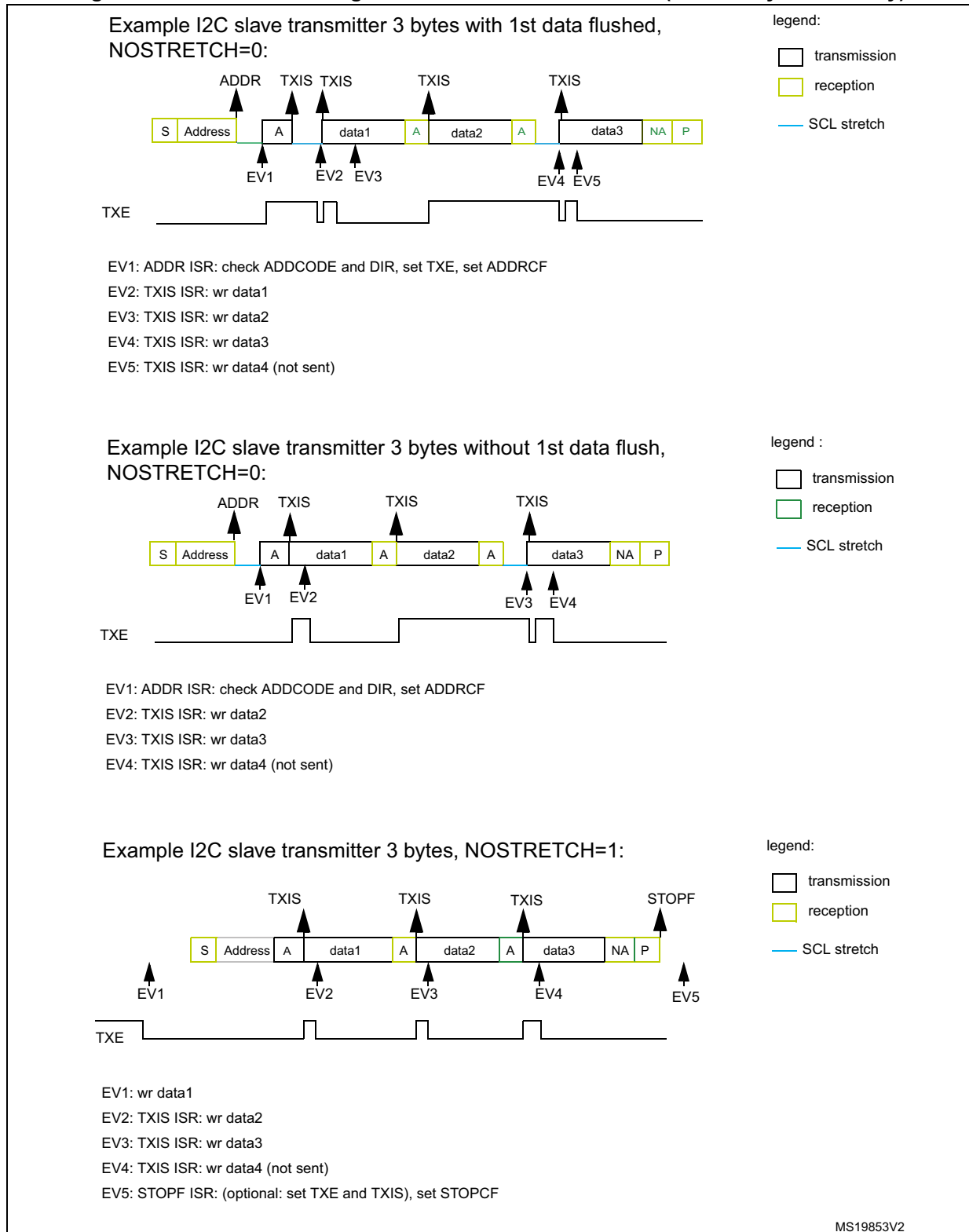
Figure 299. Transfer bus diagrams for I2C slave transmitter (mandatory events only)
