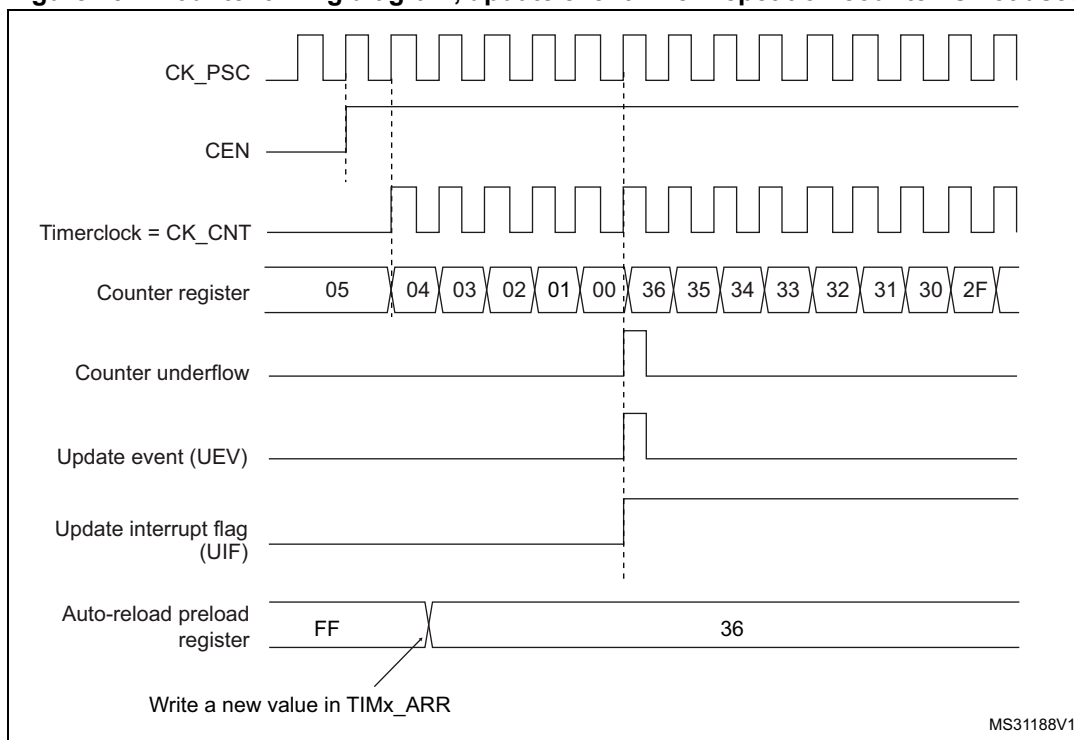
Figure 157. Counter timing diagram, update event when repetition counter is not used
