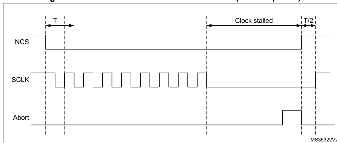
Figure 39. NCS when CKMODE = 1 with an abort (T = CLK period)
