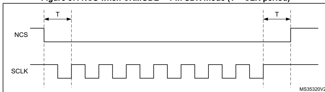
Figure 37. NCS when CKMODE = 1 in SDR mode (T = CLK period)
