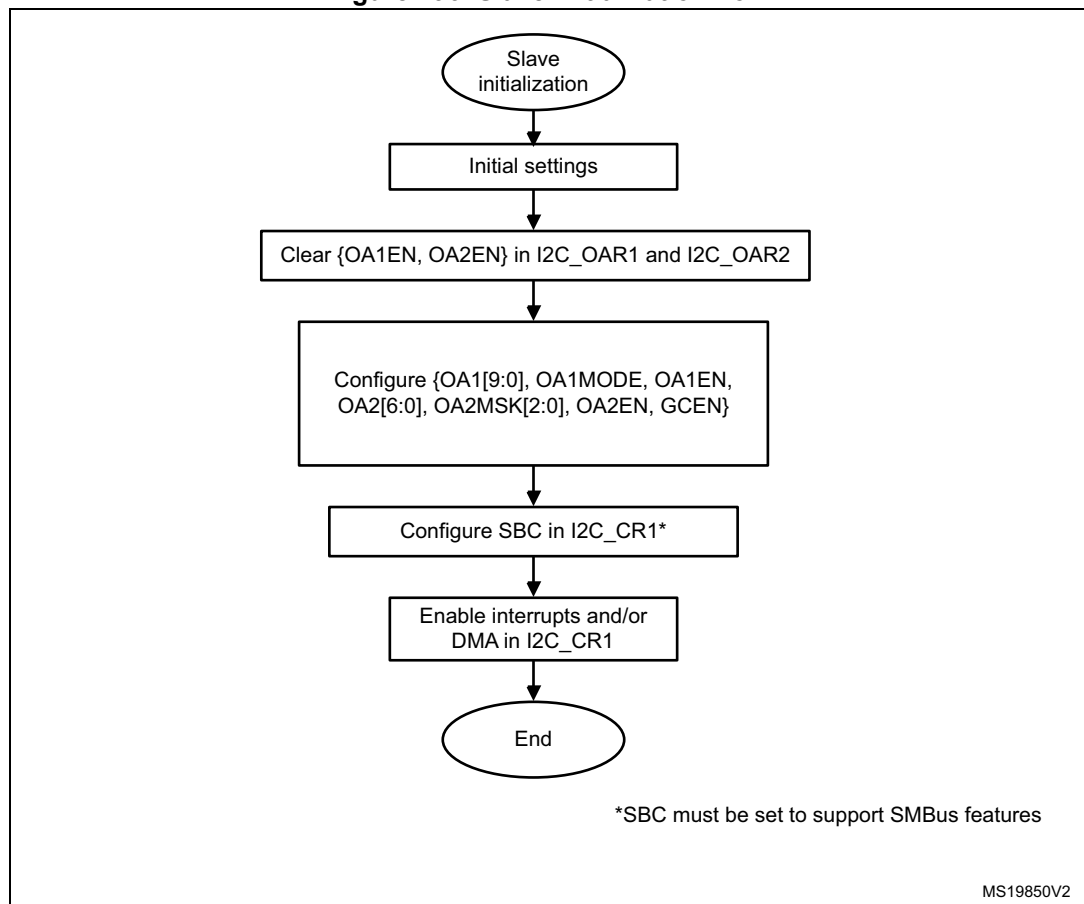
Figure 296. Slave initialization flow
