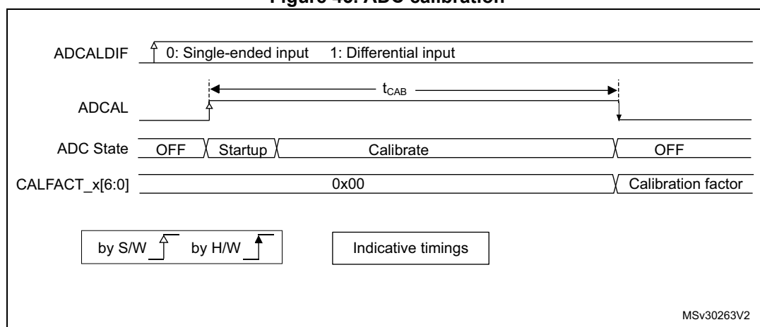
Figure 43. ADC calibration
