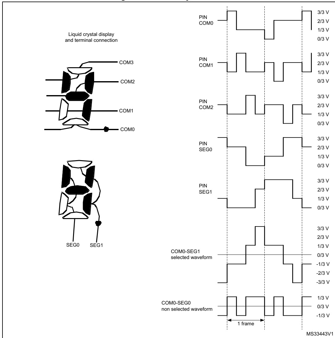
Figure 102. 1/4 duty, 1/3 bias
