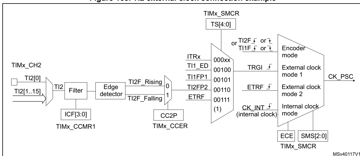
Figure 168. T12 external clock connection example
