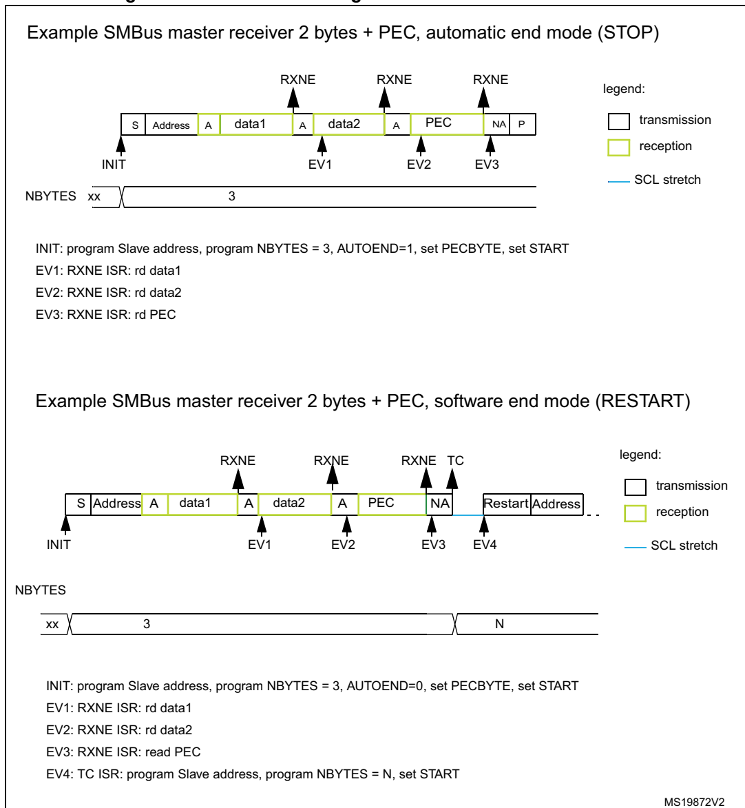
Figure 319. Bus transfer diagrams for SMBus master receiver
