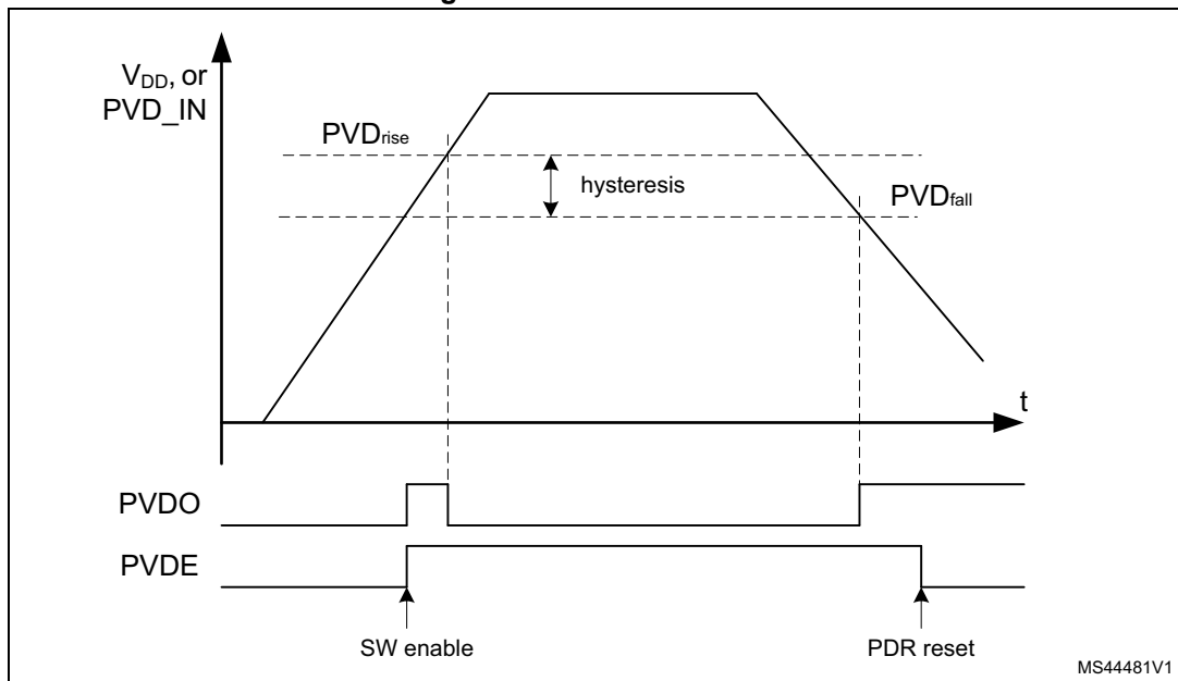
Figure 10. PVD thresholds
