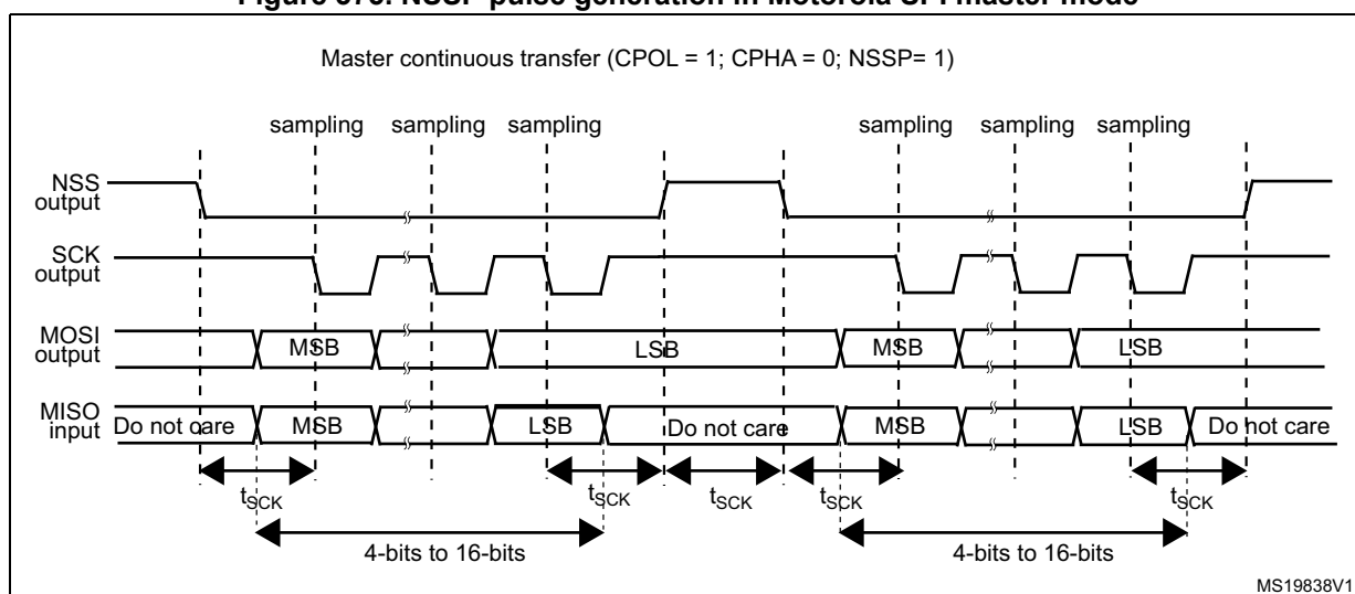
Figure 375. NSSP pulse generation in Motorola SPI master mode
