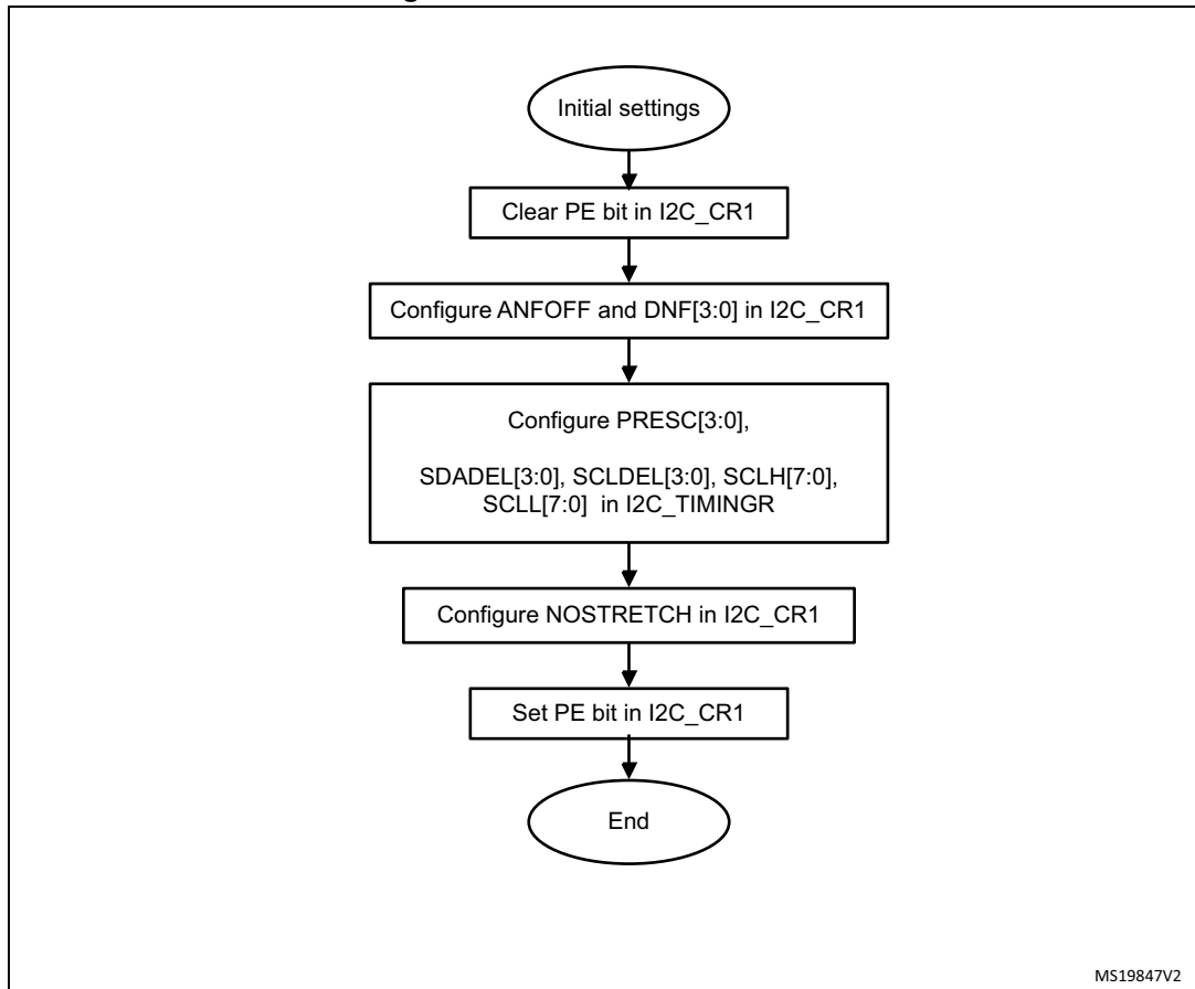
Figure 293. I2C initialization flow
