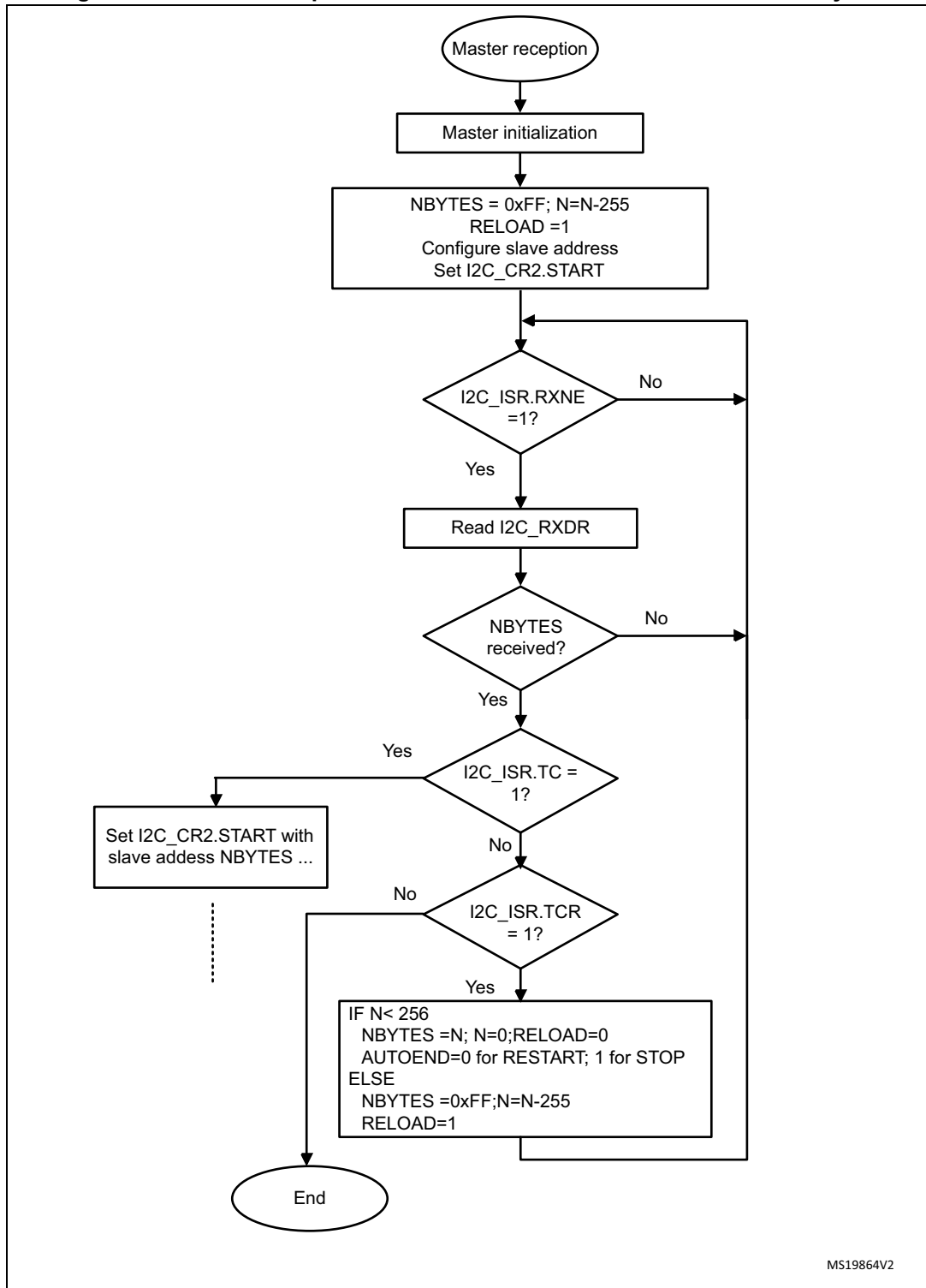
Figure 311. Transfer sequence flow for I2C master receiver for N > 255 bytes
