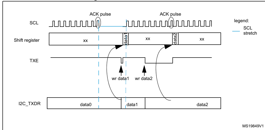
Figure 295. Data transmission
