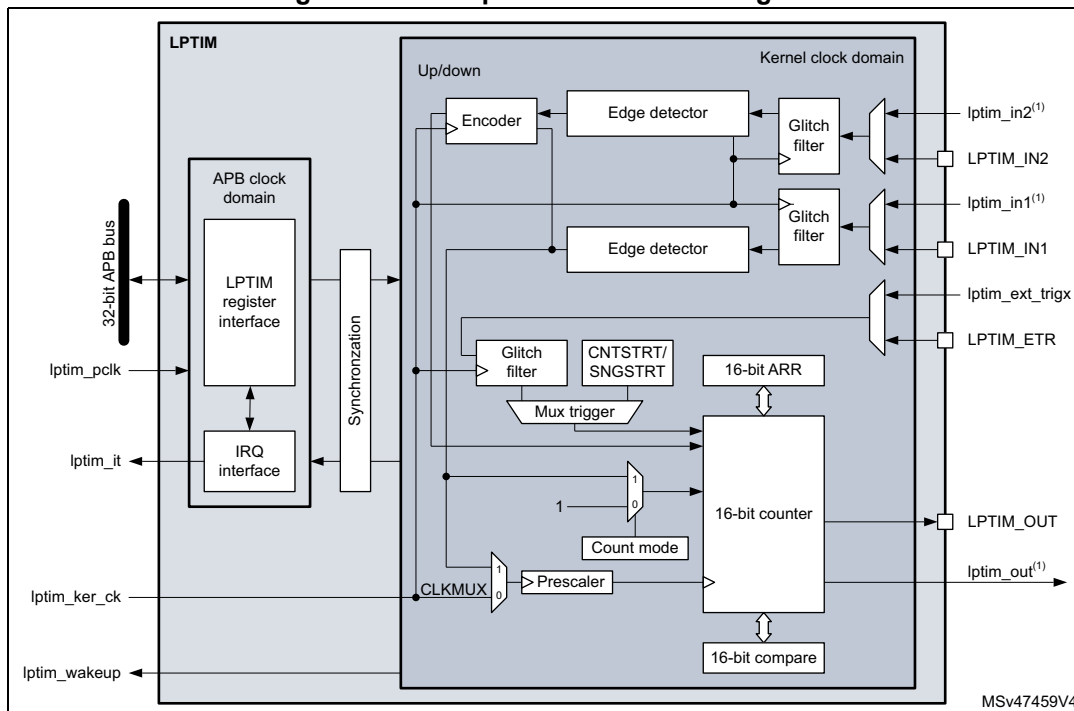
Figure 278. Low-power timer block diagram
