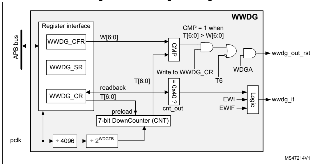
Figure 288. Watchdog block diagram
