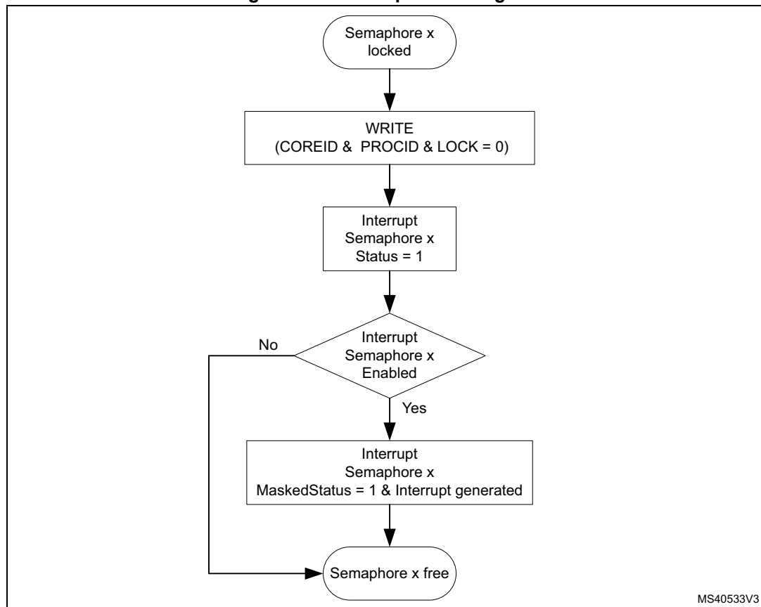
Figure 407. Interrupt state diagram
