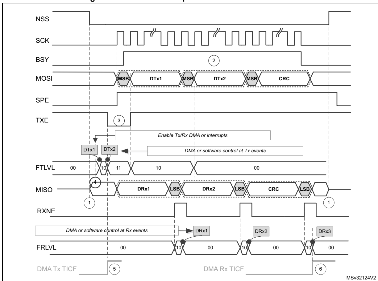
Figure 373. Master full-duplex communication with CRC
