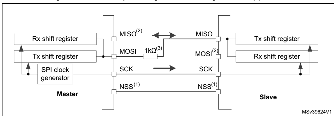
Figure 363. Half-duplex single master/ single slave application
