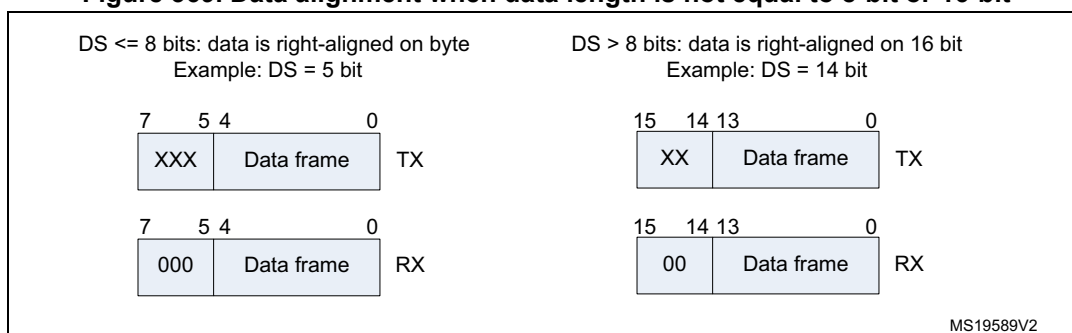
Figure 369. Data alignment when data length is not equal to 8-bit or 16-bit
