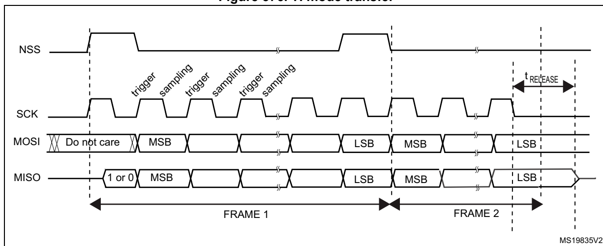
Figure 376. TI mode transfer
