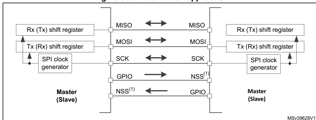
Figure 366. Multi-master application
