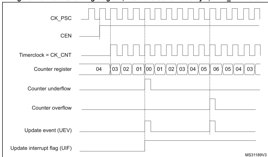
Figure 218. Counter timing diagram, internal clock divided by 1, TIMx_ARR=0x6
