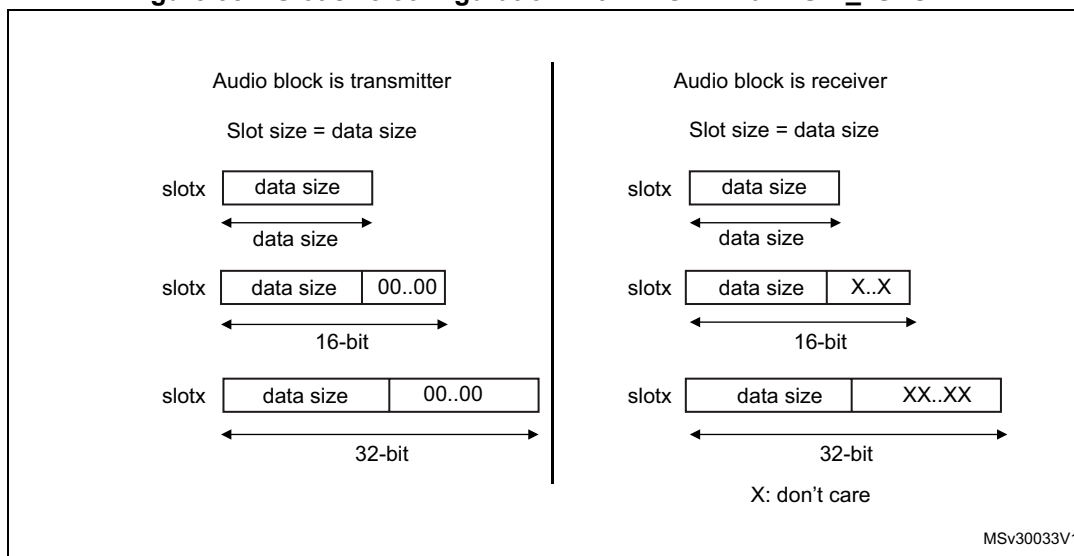
Figure 381. Slot size configuration with FBOFF = 0 in SAI_xSLOTR
