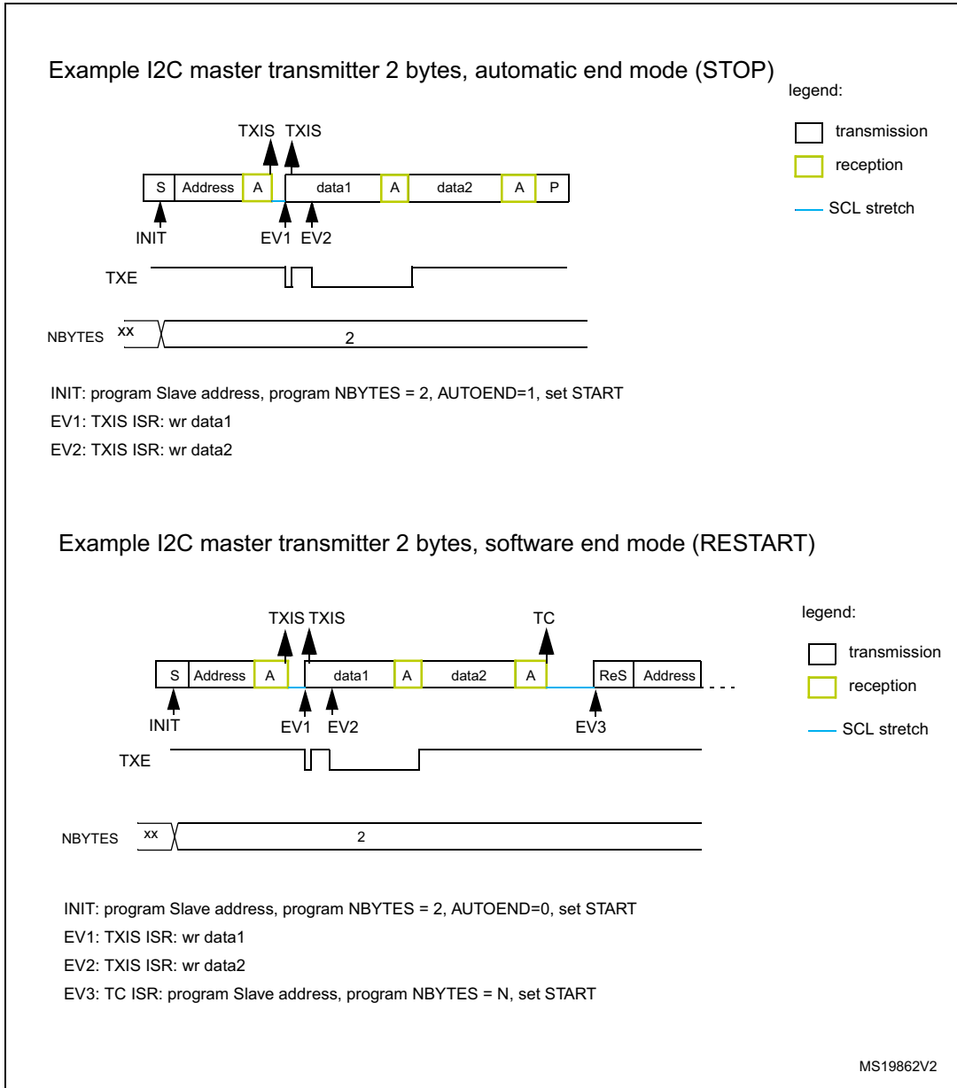
Figure 309. Transfer bus diagrams for I2C master transmitter (mandatory events only)
