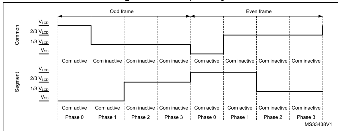
Figure 97. 1/3 bias, 1/4 duty
