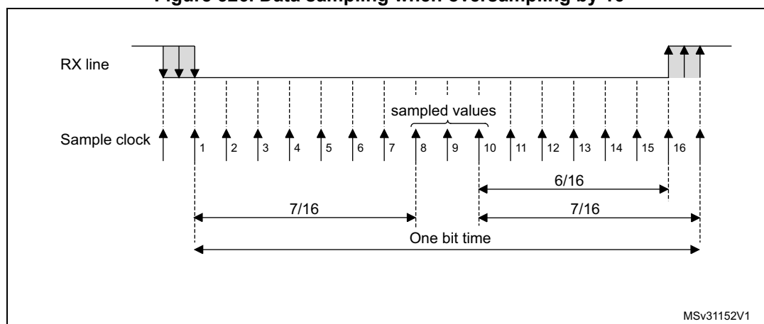
Figure 326. Data sampling when oversampling by 16
