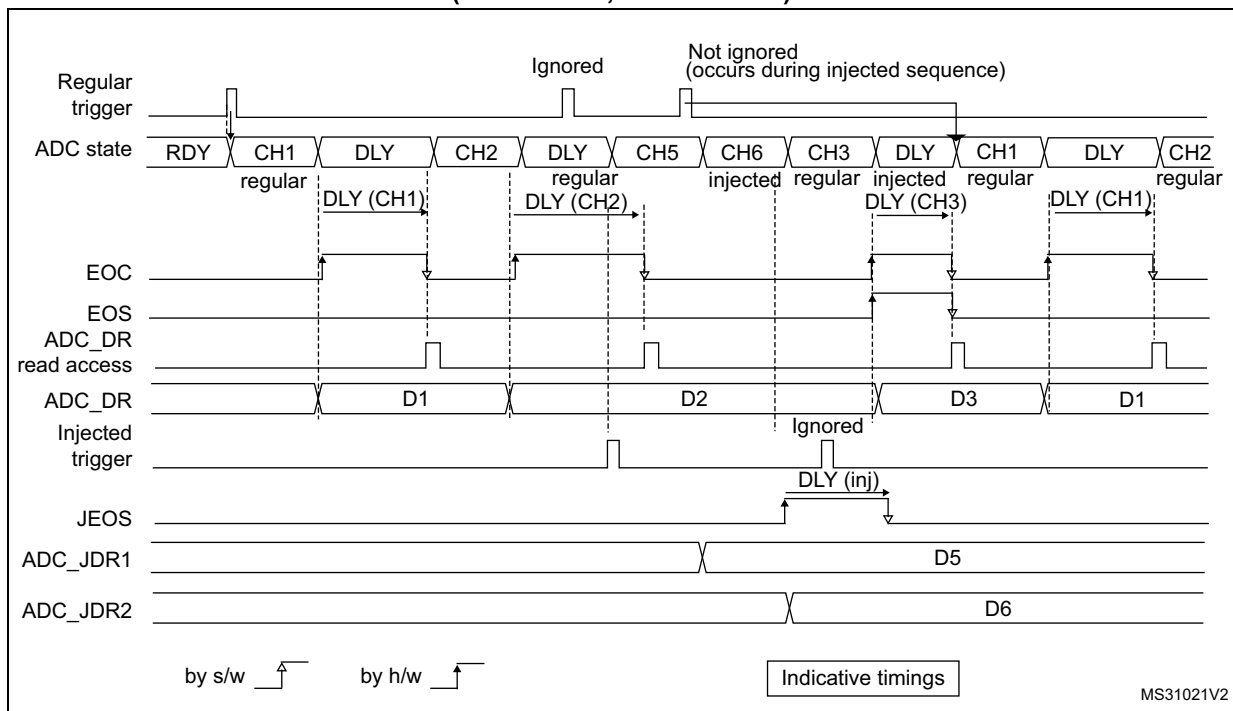
Figure 73. AUTDLY = 1, regular HW conversions interrupted by injected conversions (DISCEN = 0; JDISCEN = 0)
