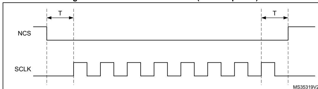
Figure 36. NCS when CKMODE = 0 (T = CLK period)
