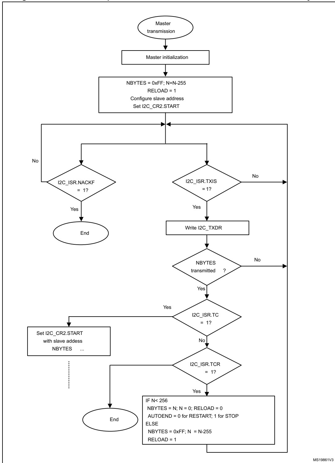
Figure 308. Transfer sequence flow for I2C master transmitter for N > 255 bytes
