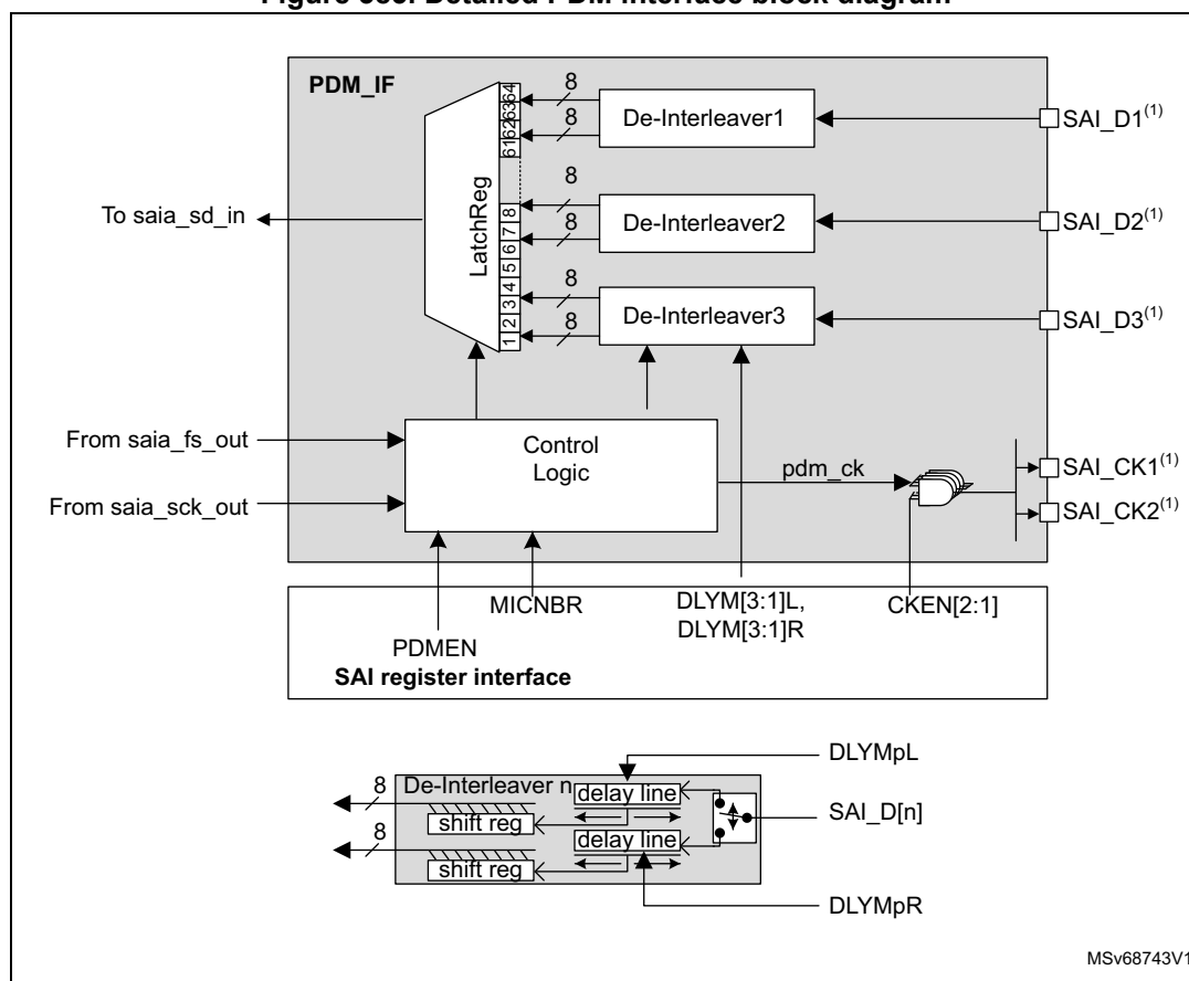
Figure 385. Detailed PDM interface block diagram
