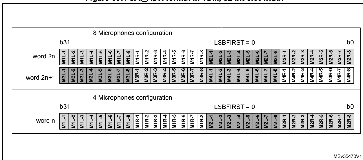
Figure 387. SAI_ADR format in TDM, 32-bit slot width
