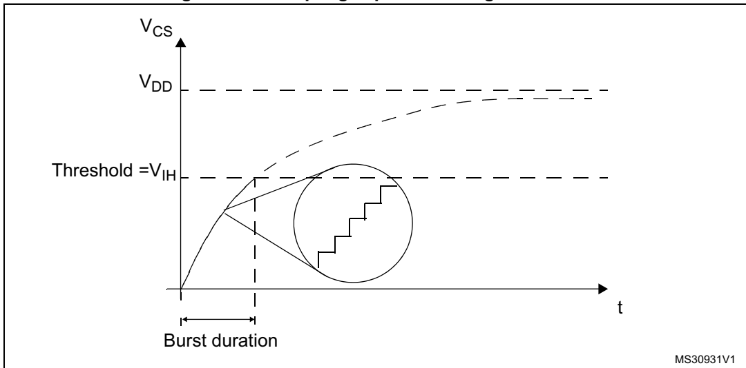
Figure 110. Sampling capacitor voltage variation
