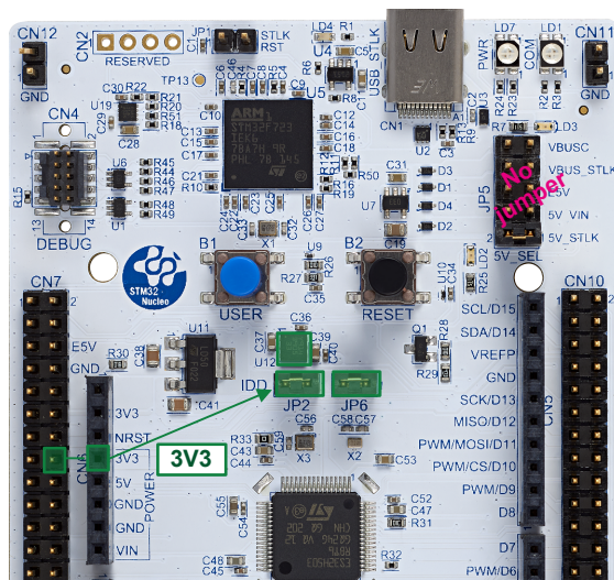
Figure 14. Power supply input from external 3V3
