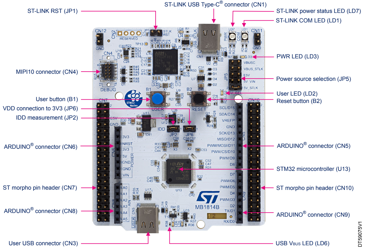
Figure 5. Top layout
