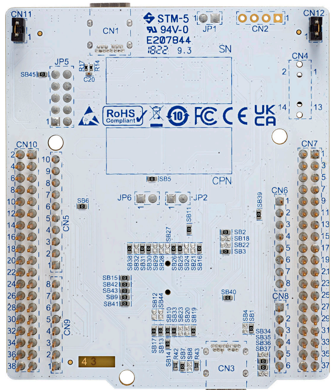
Figure 2. NUCLEO-H503RB bottom view
