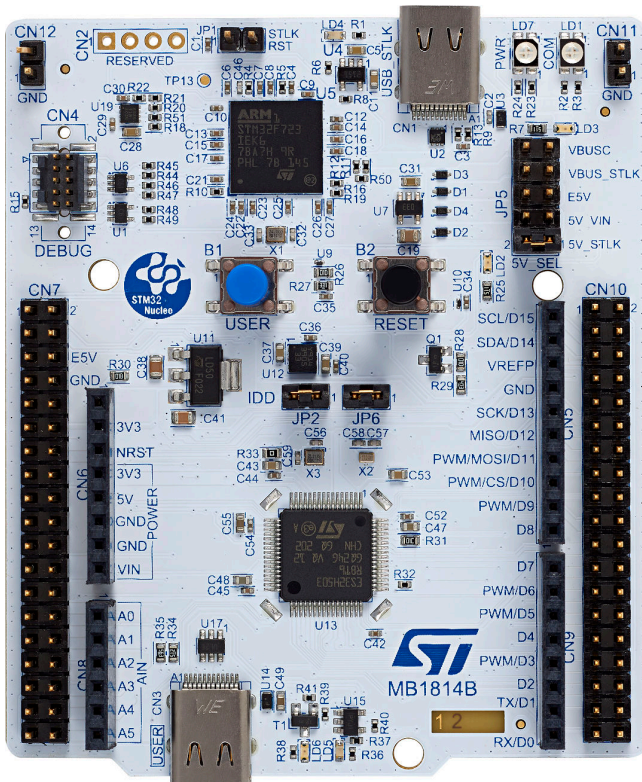
Figure 1. NUCLEO-H503RB top view
