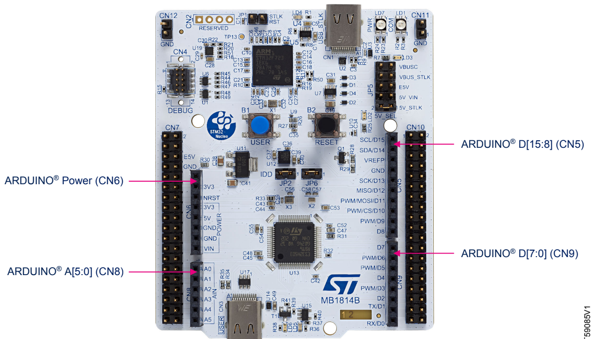
Figure 17. ARDUINO® connectors
