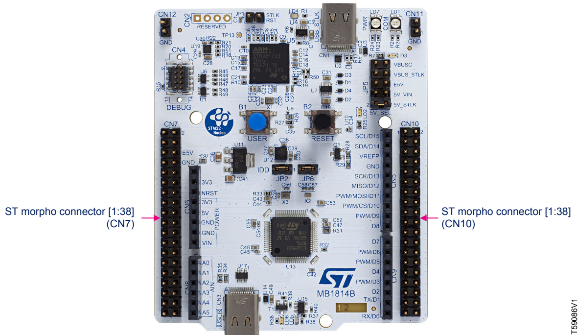
Figure 18. ST morpho connectors (CN7 and CN10)
