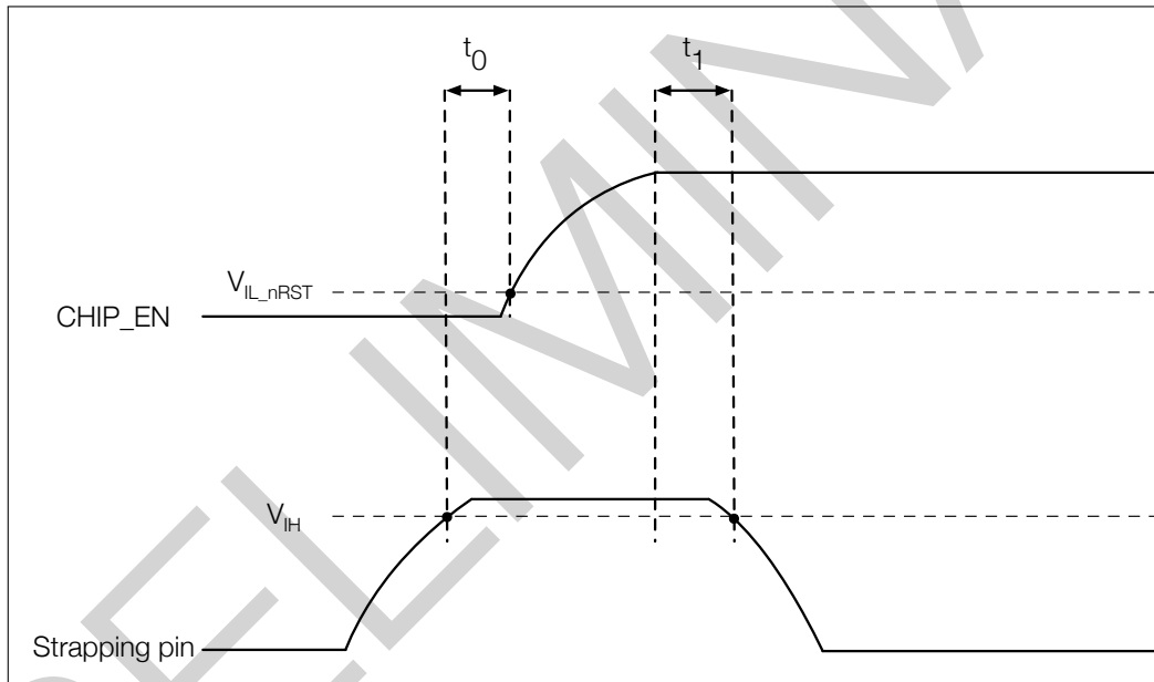
Figure 4: Setup and Hold Times for the Strapping Pin
