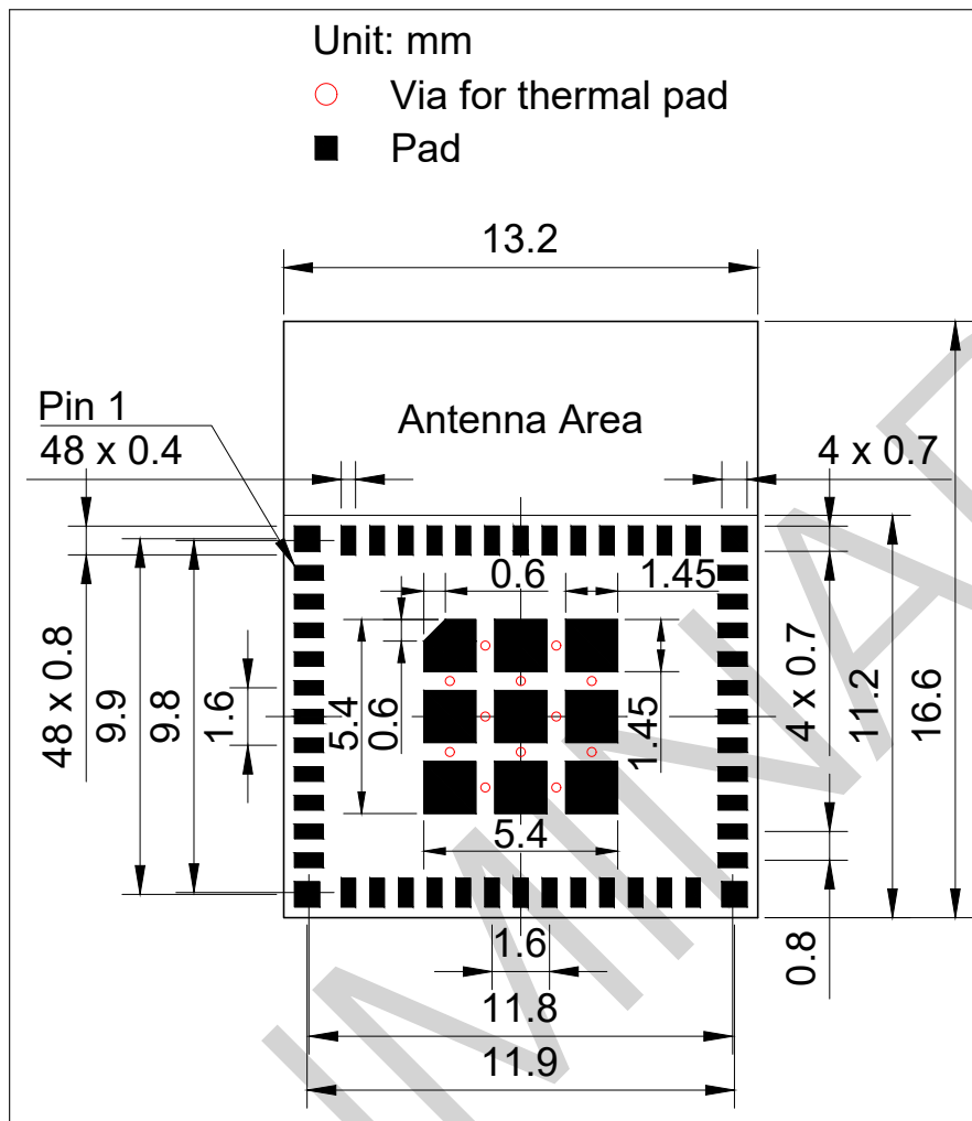
Figure 10: ESP32-H2-MINI-1 Recommended PCB Land Pattern
