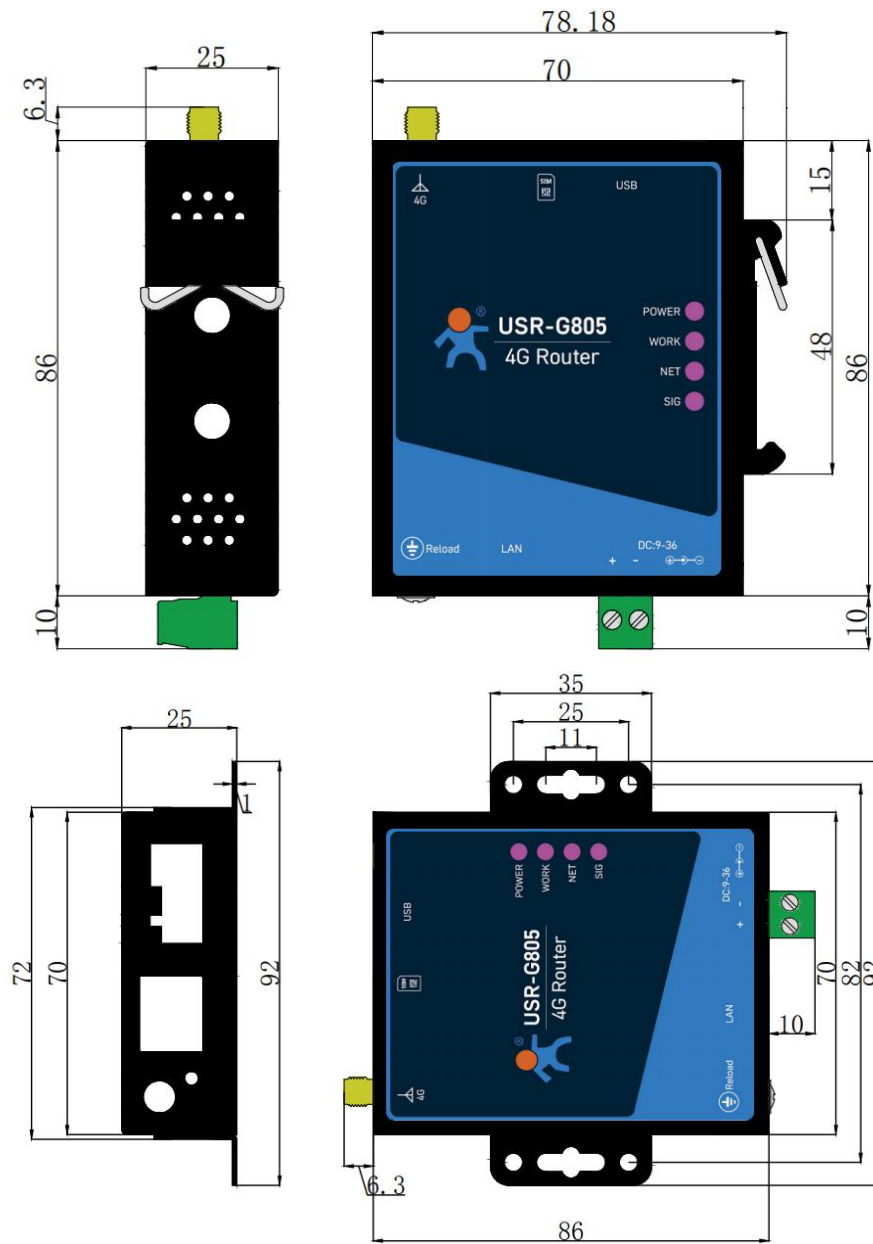
USR-G805 Dimensions
