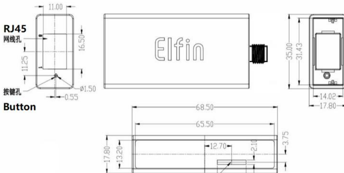
Figure 7. Elfin-EW4X Mechanical Dimension
