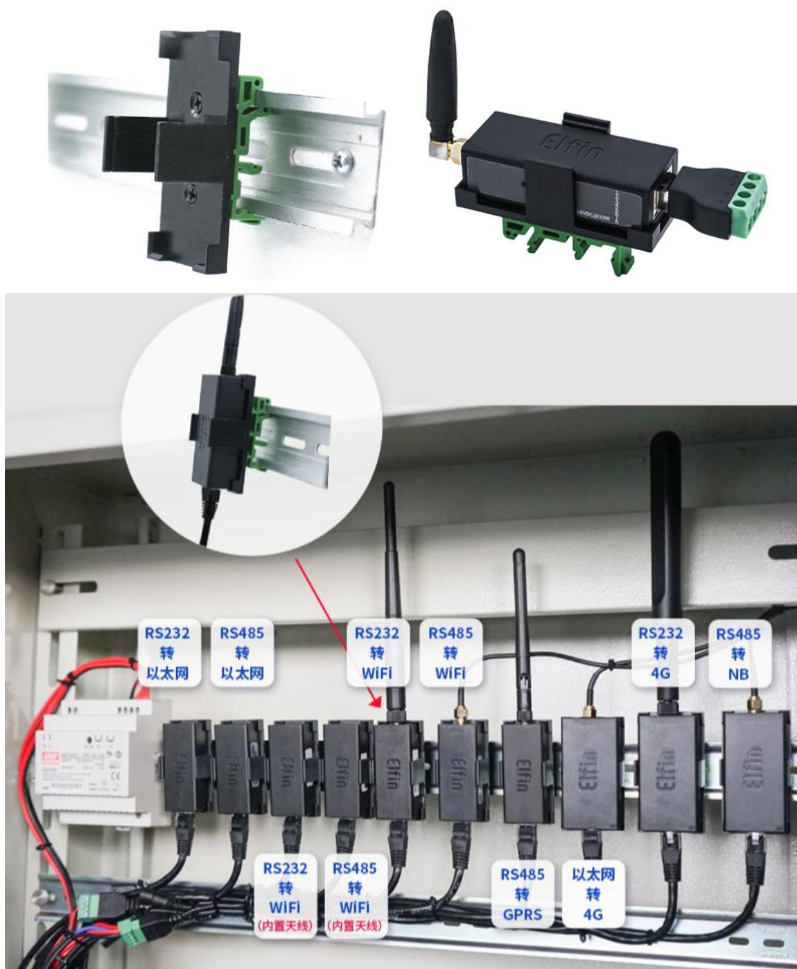
Figure 25. Bracket Install Picture
