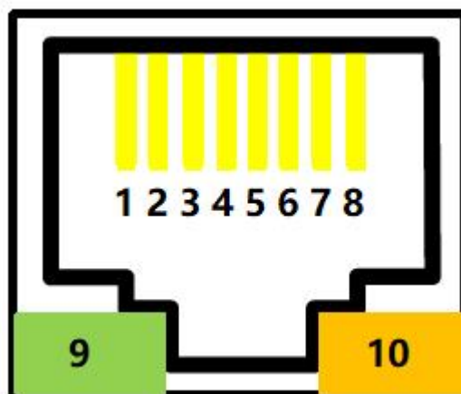
Figure 5. Elfin-EW41 RJ45 Interface Pin
