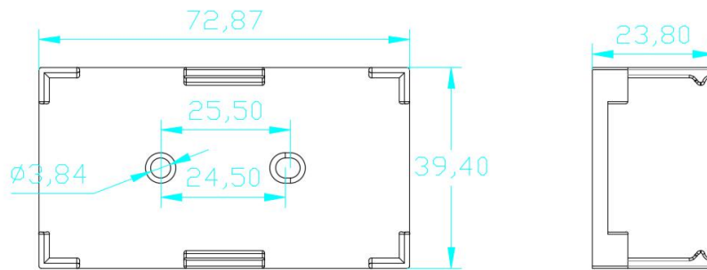
Figure 22. Fixed support dimensions drawing
