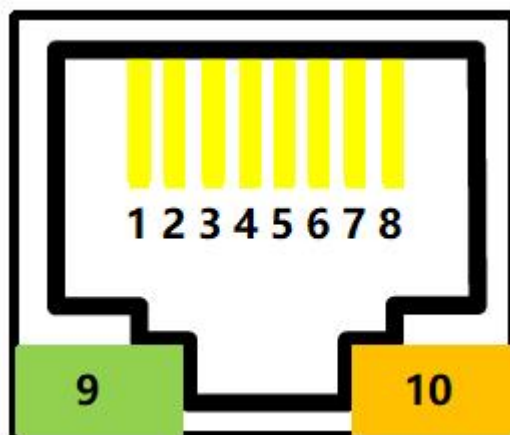
Figure 6. Elfin-EW42 RJ45 Interface Pin
