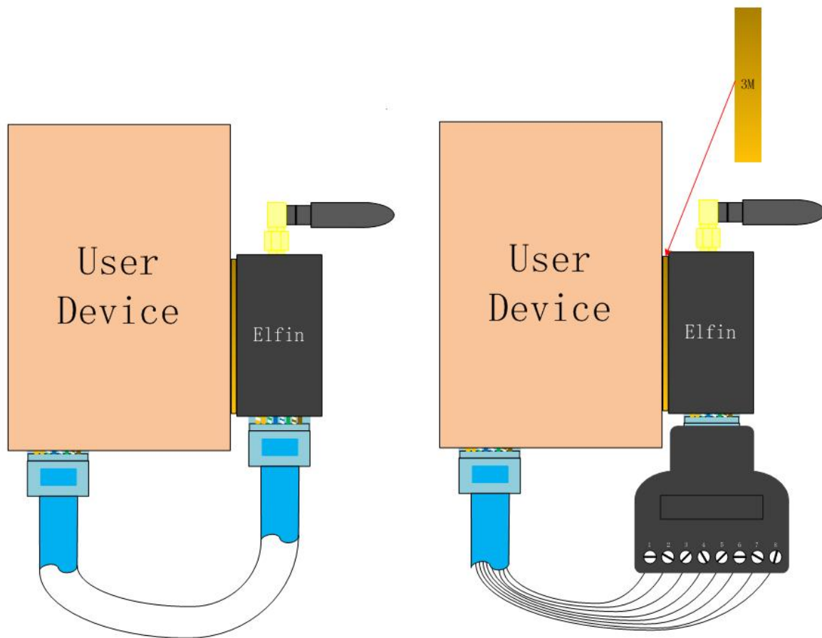
Figure 26. Product Installation
