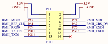
ETH
