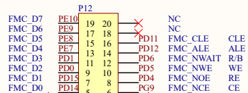
NAND FLASH
