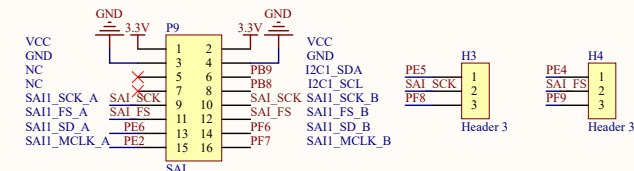
SAI_A
