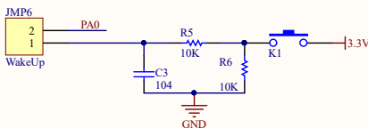
WakeUp Button
