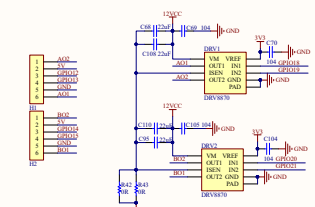
Motor Driver
