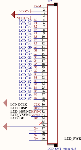
LCD_SMT_40pin_0.5
