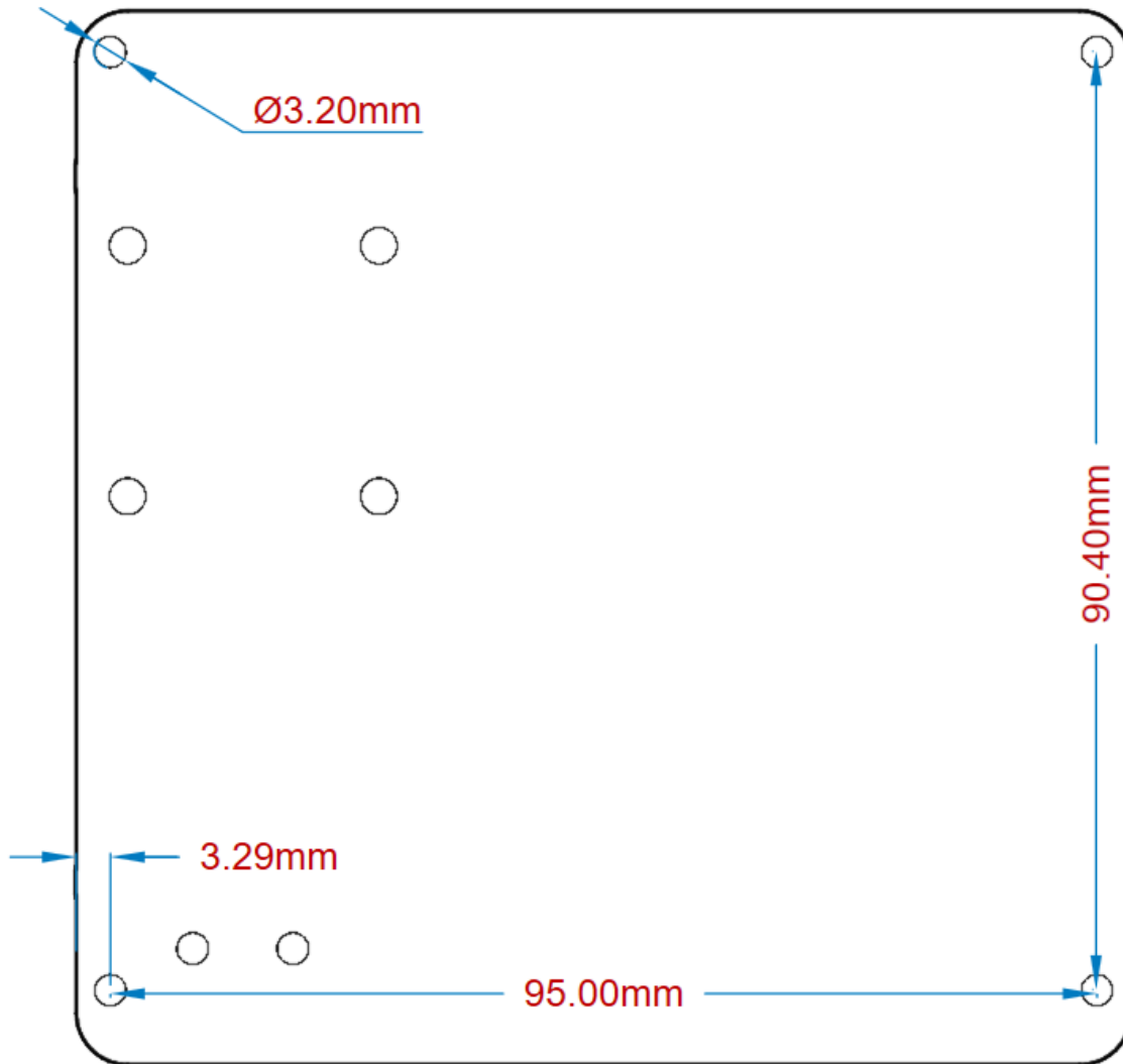
Mounting holes
