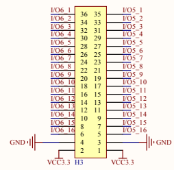
32I/Os_1
