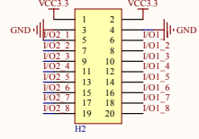
16I/Os_1
