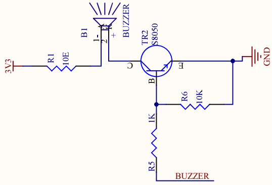
BUZZER DRIVER
