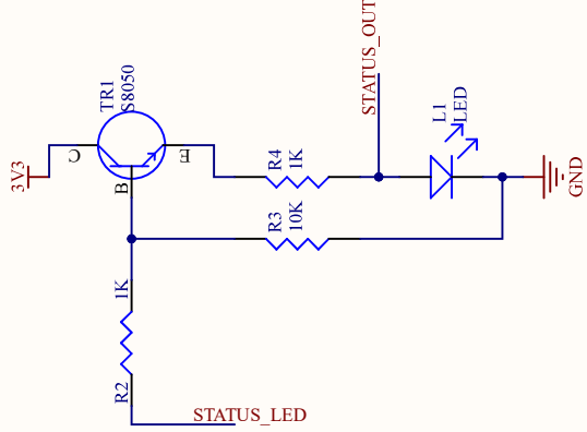
LED DRIVER
