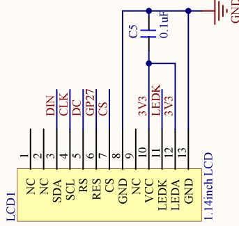
1.14inch LCD
