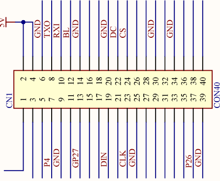
RASPBERRY PI INTERFACE
