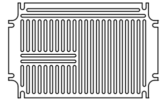
Baseplate, P/N ZMB180.120 IOT p3
