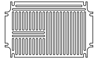
Baseplate, P/N ZMB180.120 IOT m3
