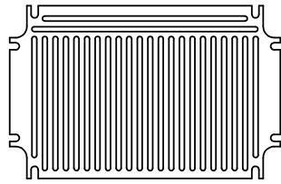
Baseplate, P/N ZMB180.120 IOT m2
