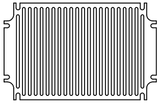
Baseplate, P/N ZMB180.120 IOT p1
