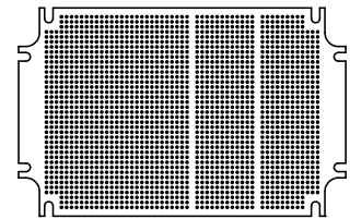
Universal PCB, P/N ZP.180.120 PCB A
