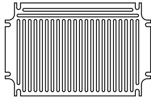
Baseplate, P/N ZMB180.120 IOT p2
