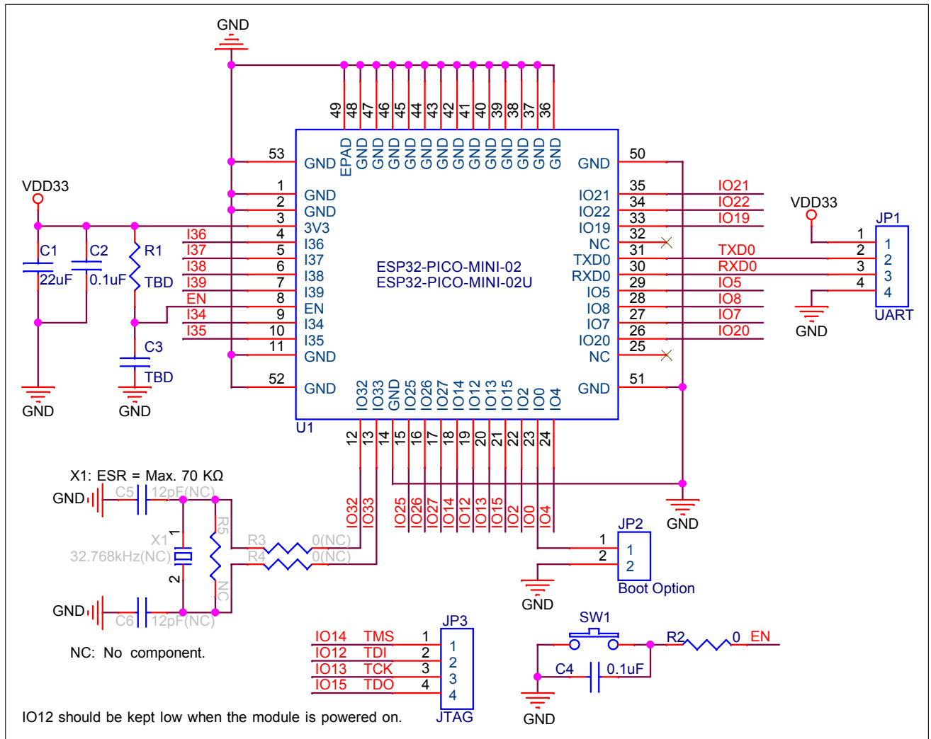
Figure 7: Peripheral Schematics
