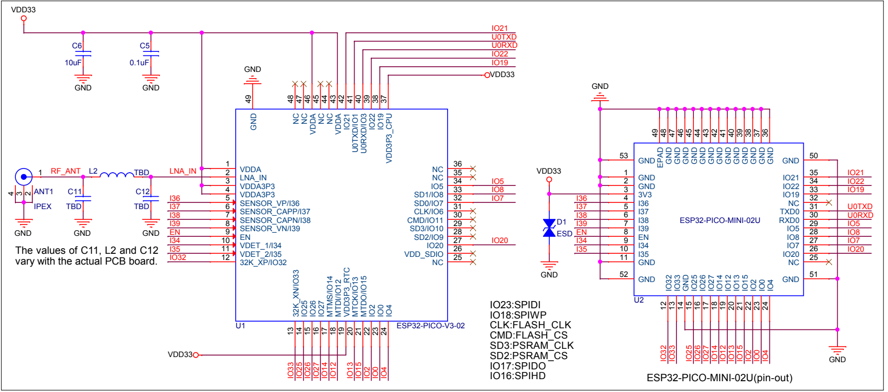
Figure 6: ESP32-PICO-MINI-02U Schematics
