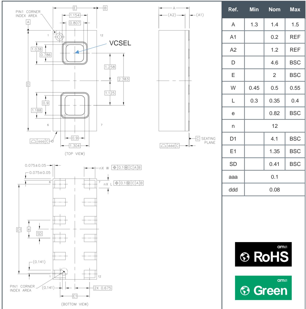
Figure 150: OLGA12 Package Outline Drawing
