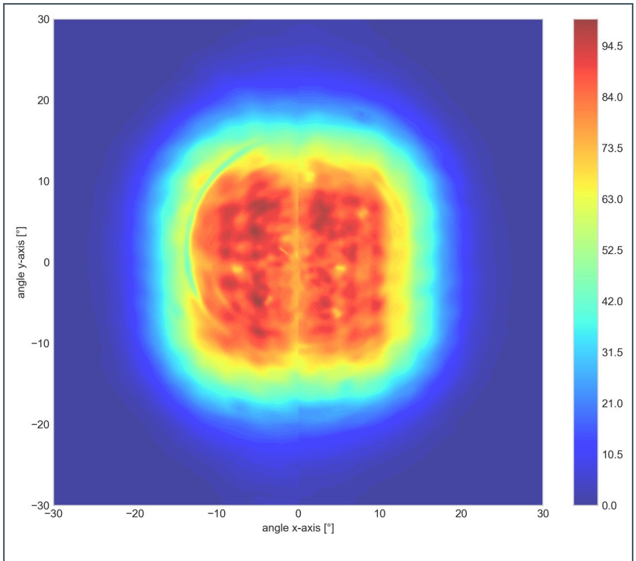
Figure 41: Field of Illumination Shown in Pseudocolors in [%] of Max Range
