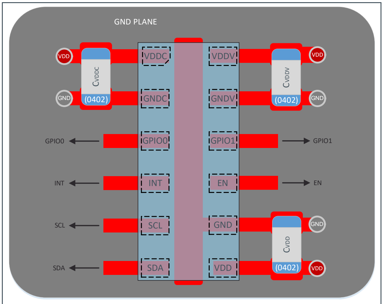
Figure 148: PCB Layout Recommendation
