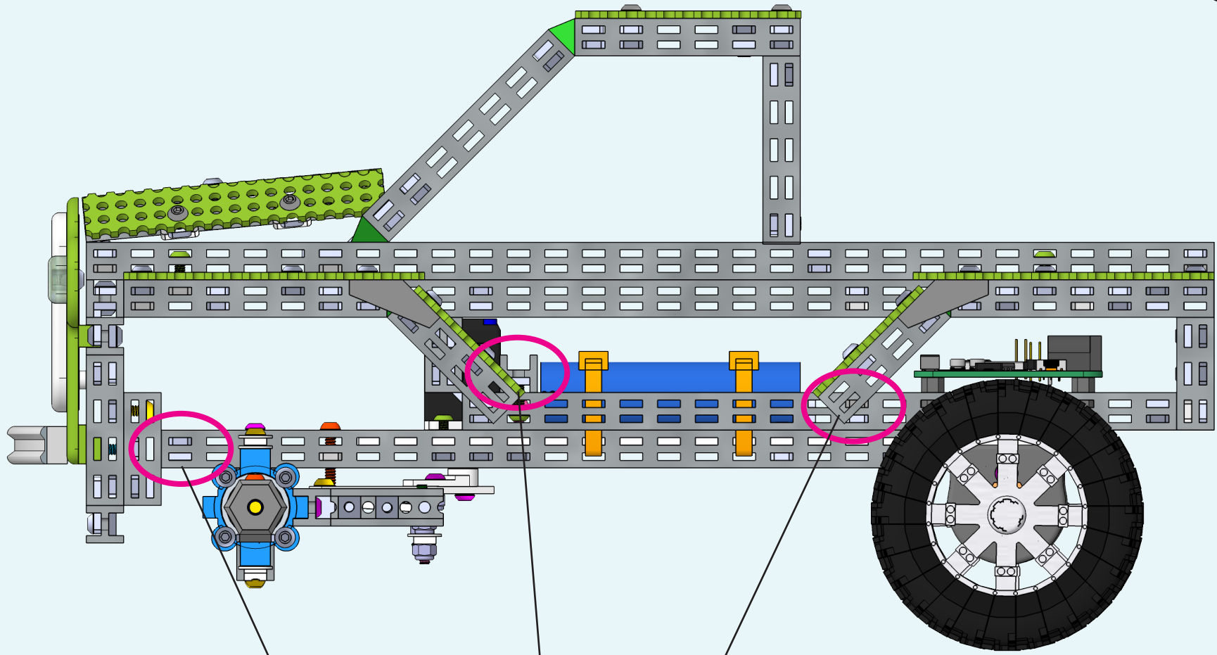
Contact points between chassis and body-top.
