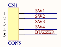
BUTTON CONNECTOR
