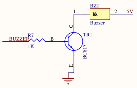
BUZZER
