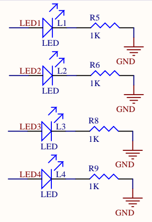
LED
