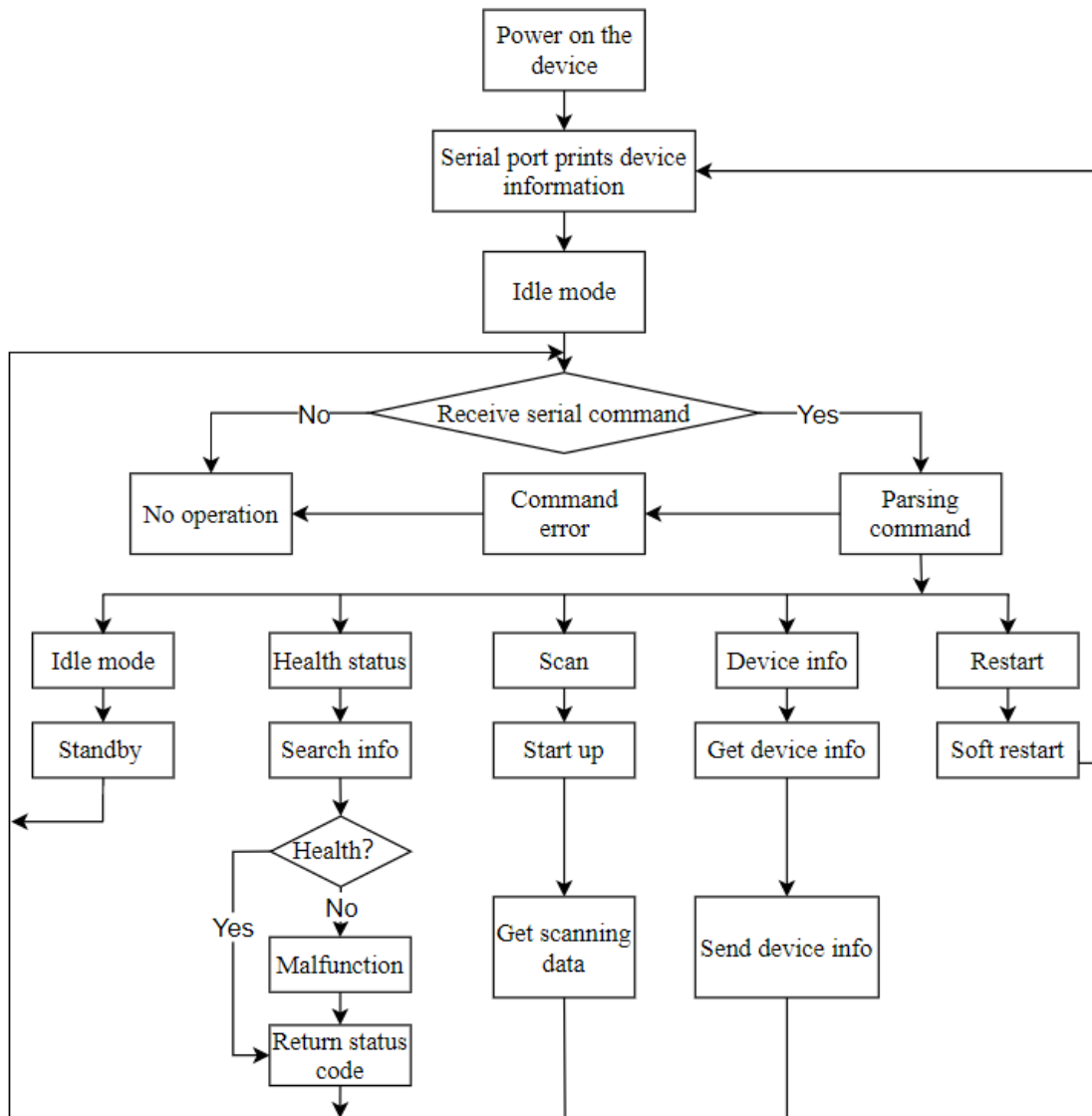
FIG 1 YDLIDAR X4 WORKFLOW
