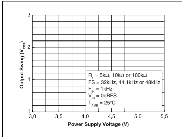
Figure 13. Output swing vs. power supply voltage
